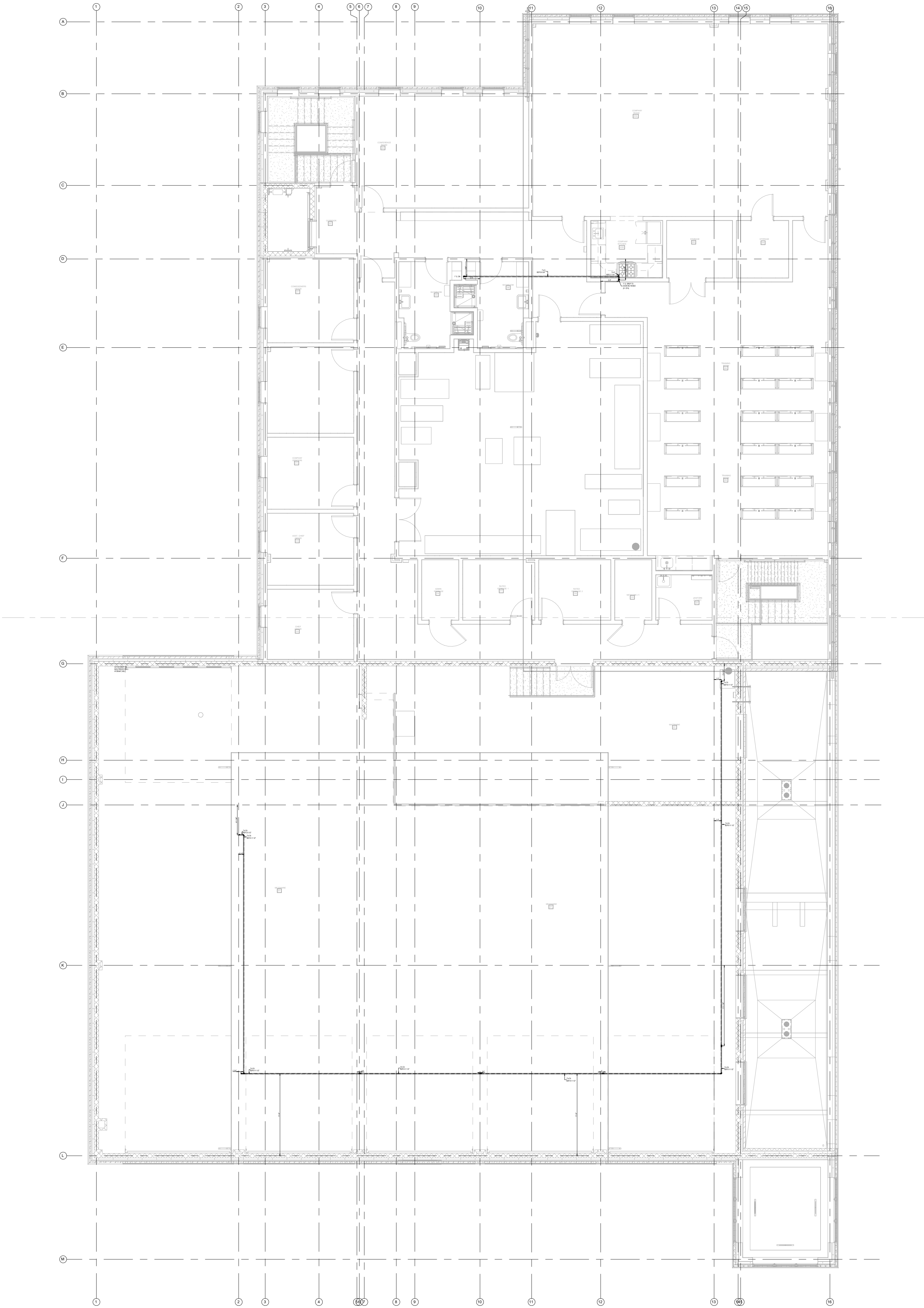
1 #4 PLUMBING- PHASE-2 BLDG 2 PLUMBING SHOP DWG LEVEL-2 GAS PLAN 1/4" = 1'-0"
