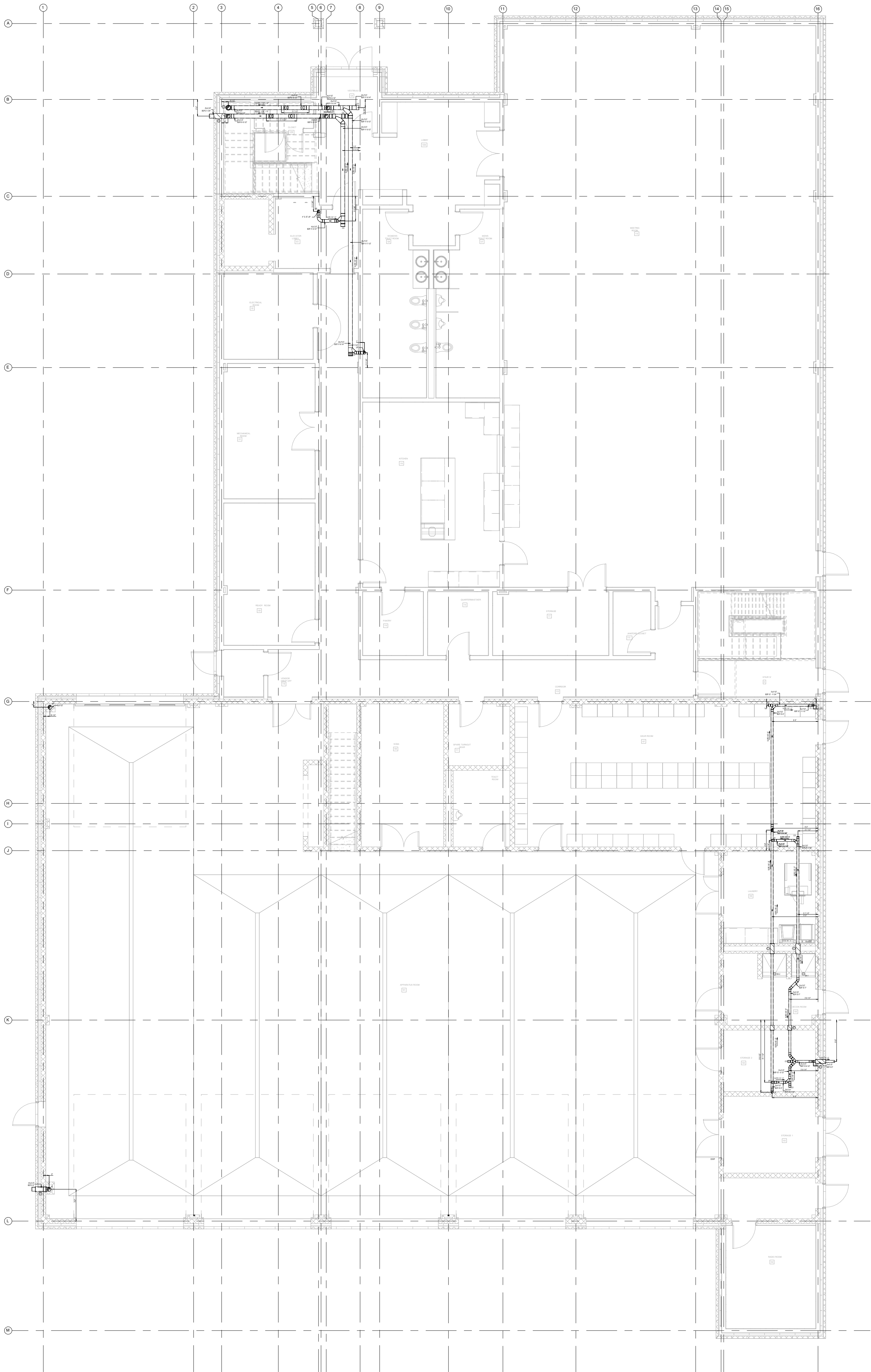
1 #4 PLUMBING- PHASE-2 BLDG 2 PLUMBING SHOP DWG LEVEL-1 STORM DRAIN PLAN 1/4" = 1'-0"
