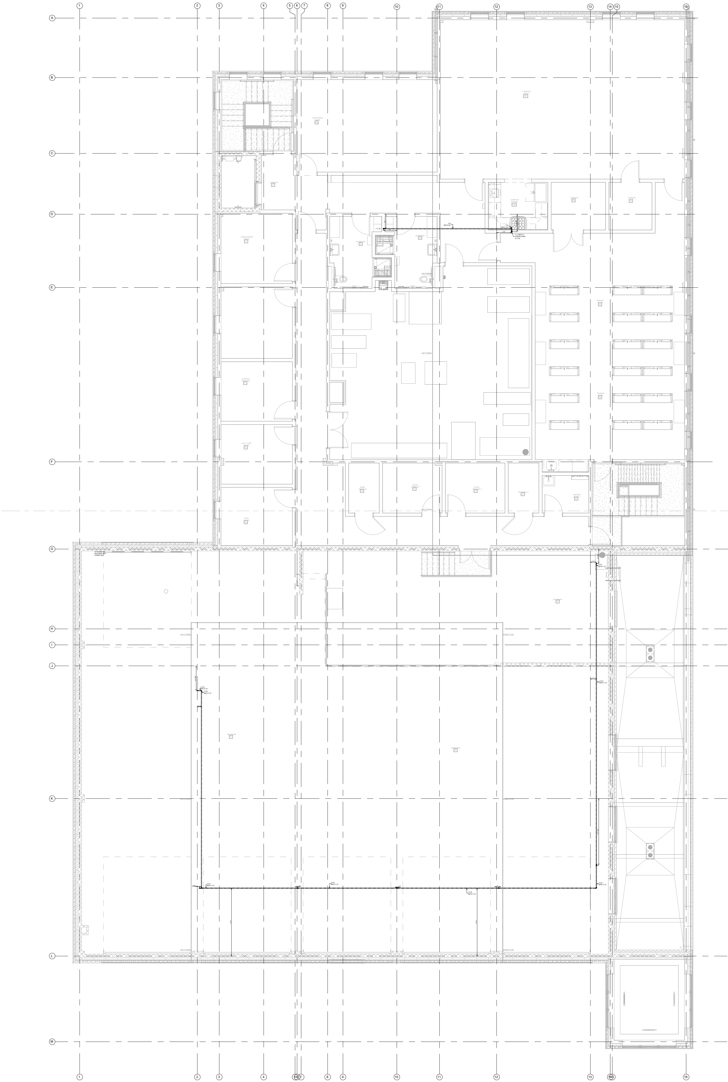
1 #4 PLUMBING- PHASE-2 BLDG 2 PLUMBING SHOP DWG LEVEL-2 GAS PLAN 1/4" = 1'-0"
