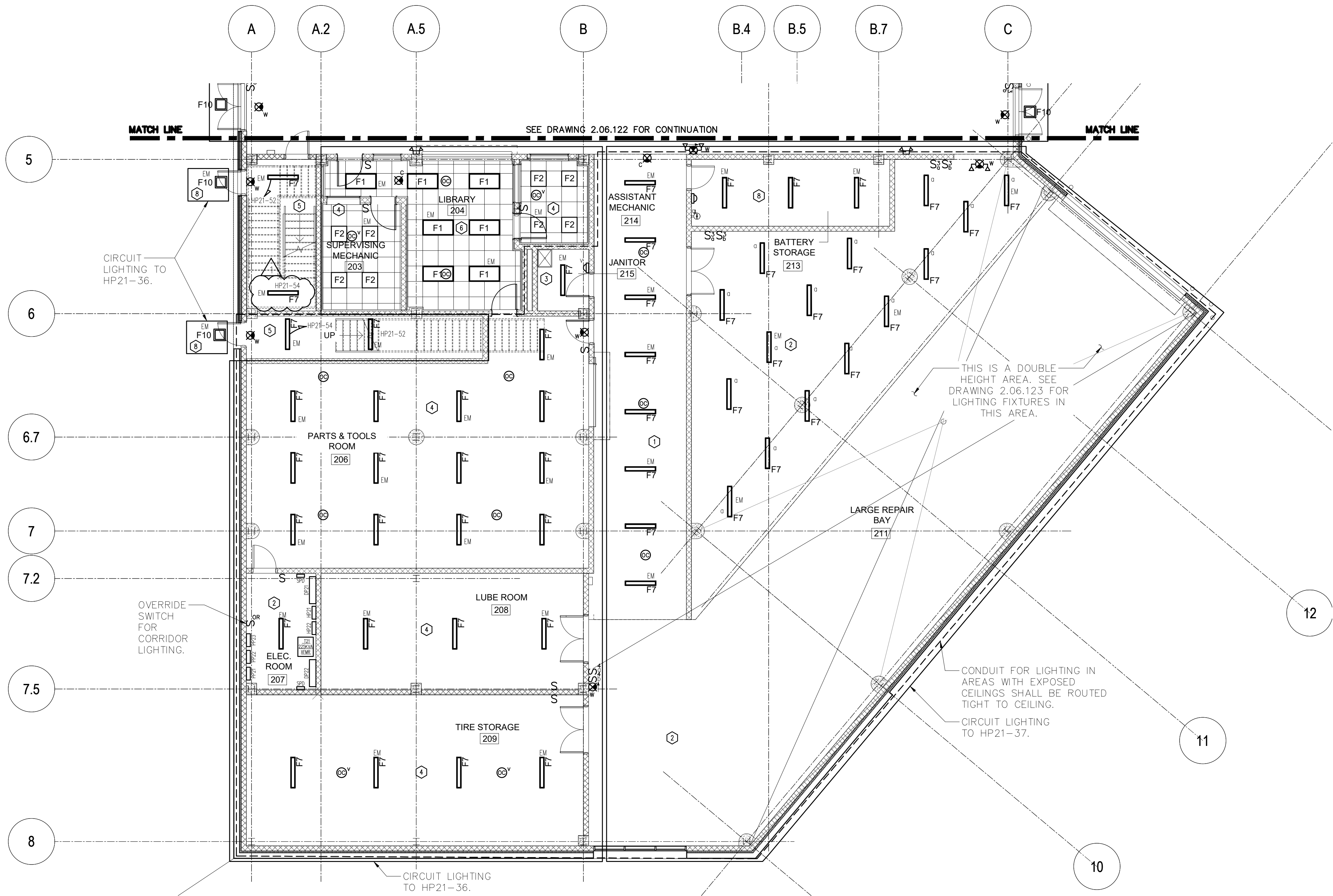
1 ELECTRICAL BUILDING 02 LIGHTING PART PLAN SCALE: 1/8" = 1'-0"
