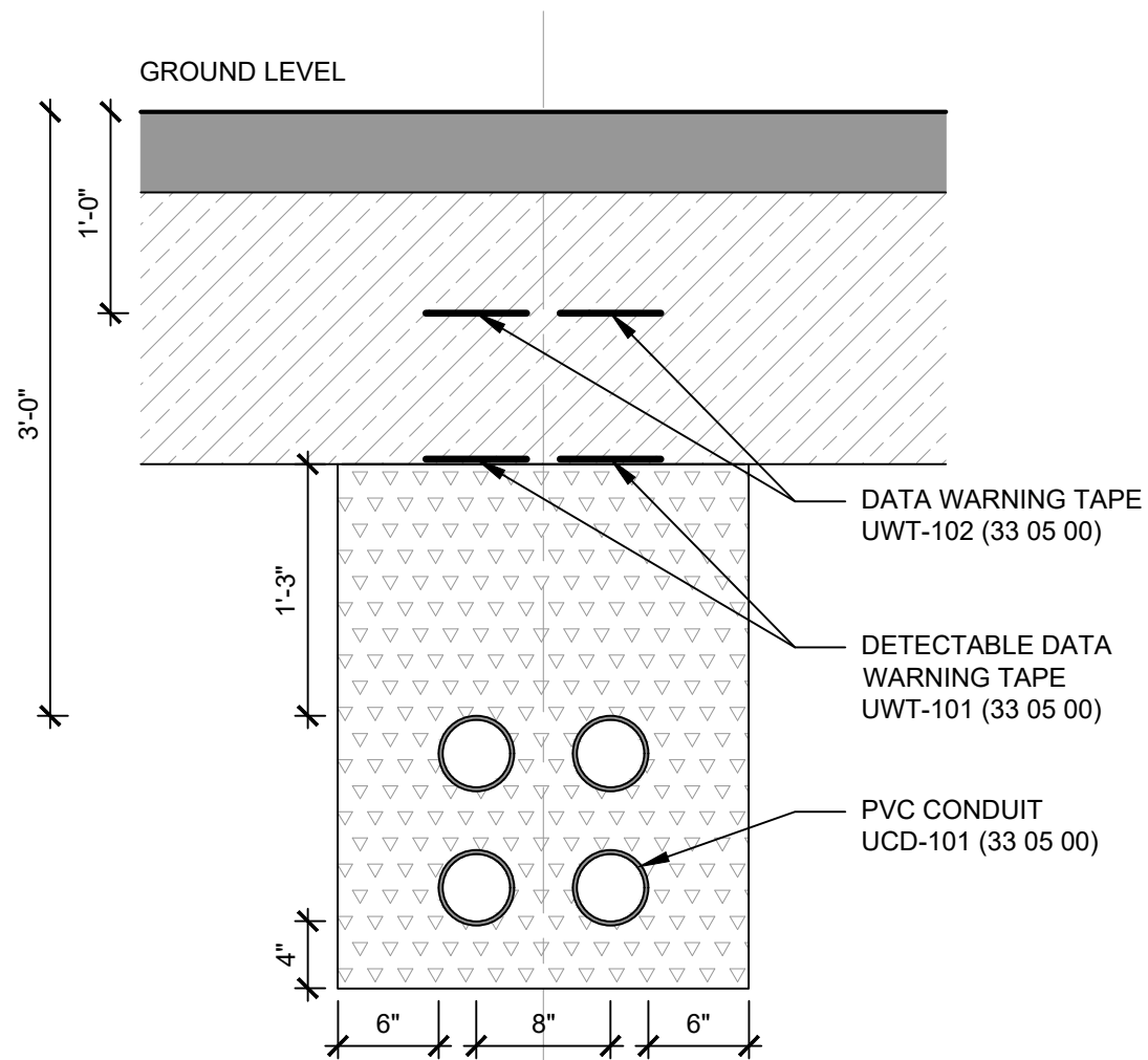
06 DATA - PAVED SURFACE 1" = 1' 0 6" 1' 2'
