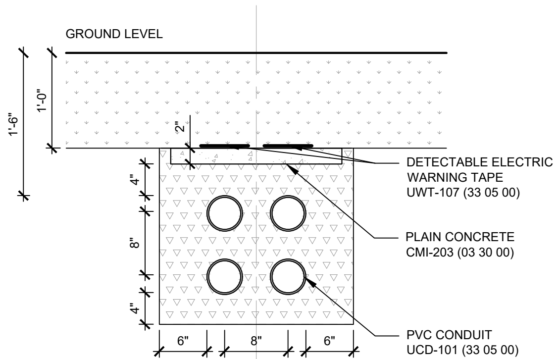
11 ELECTRIC - NON-PAVED/SHALLOW SURFACE 1" = 1' 0 6" 1' 2'
