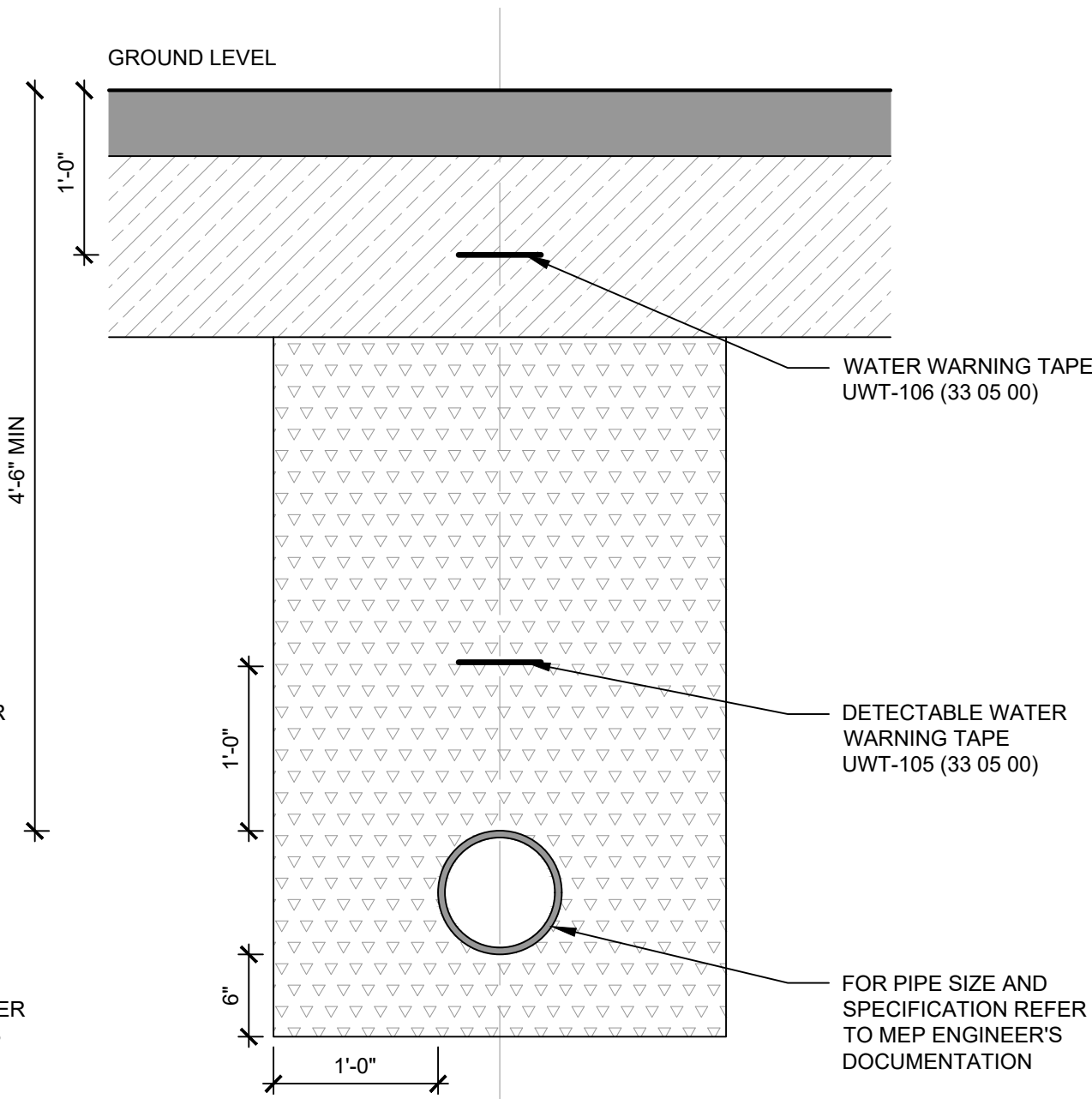
04 WATER - PAVED SURFACE 1" = 1' 0 6" 1' 2'
