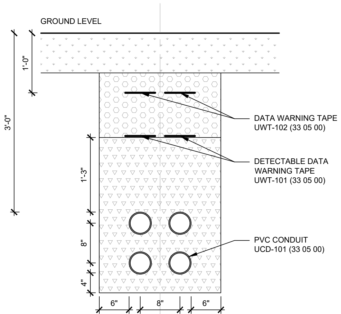
05 DATA - NON-PAVED SURFACE 1" = 1' 0 6" 1' 2'
