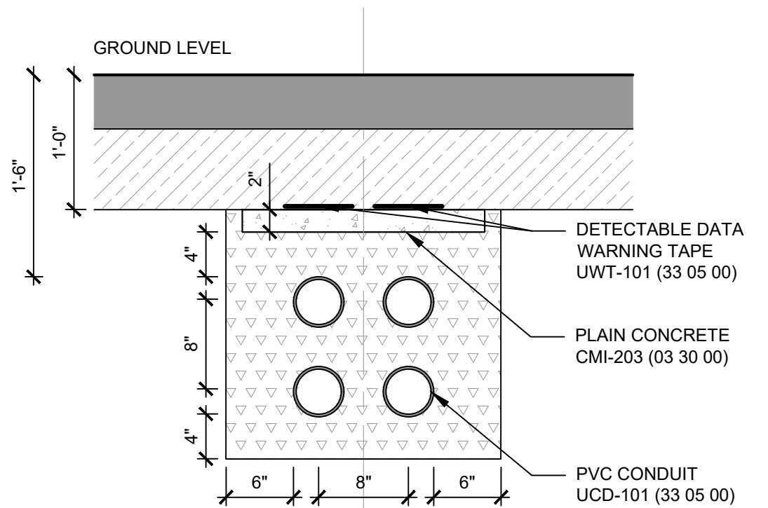
10 DATA - PAVED/SHALLOW SURFACE 1" = 1' 0 6" 1' 2'
