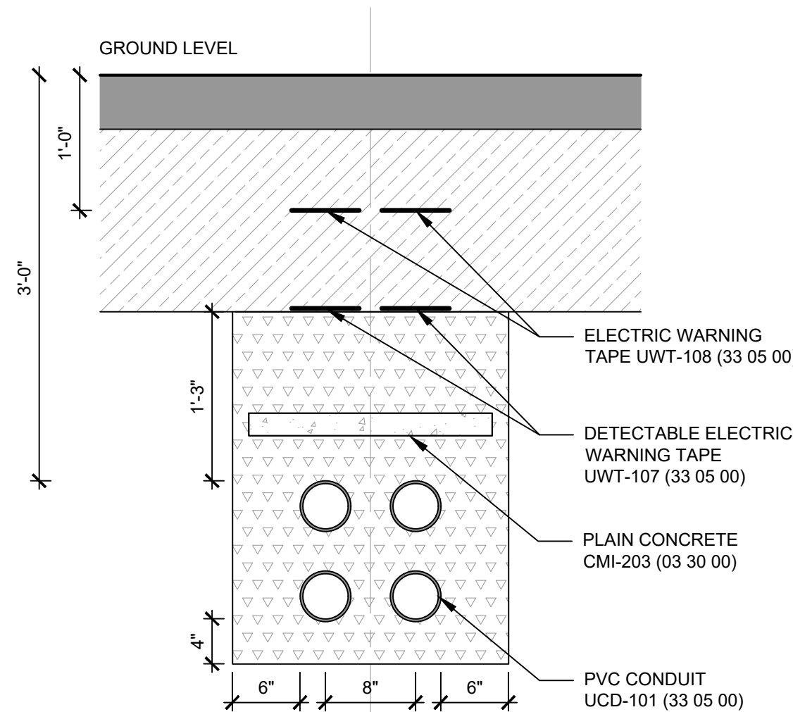
08 ELECTRIC - PAVED SURFACE 1" = 1' 0 6" 1' 2'
