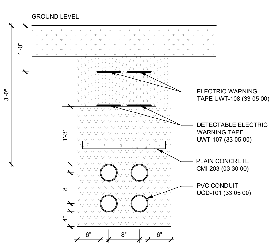
07 ELECTRIC - NON-PAVED SURFACE 1" = 1' 0 6" 1' 2'
