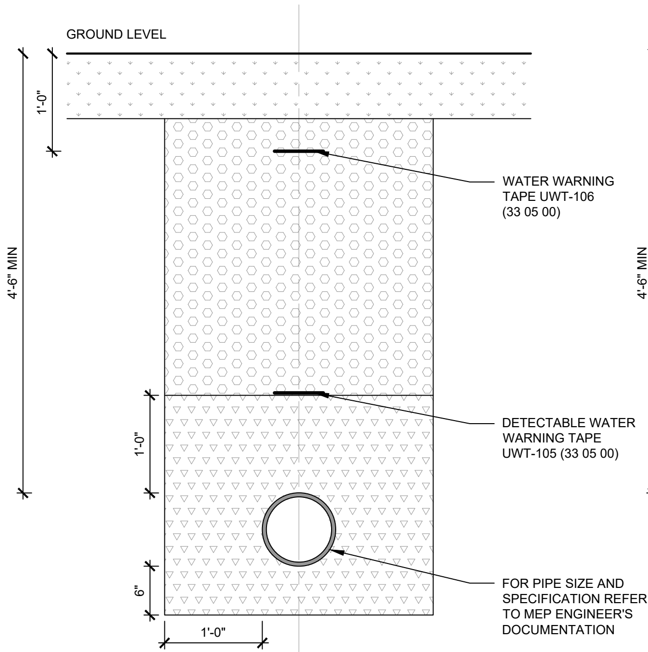
03 WATER - NON-PAVED SURFACE 1" = 1' 0 6" 1' 2'
