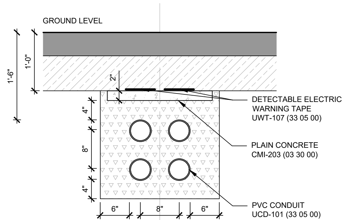
12 ELECTRIC - PAVED/SHALLOW SURFACE 1" = 1' 0 6" 1' 2'
