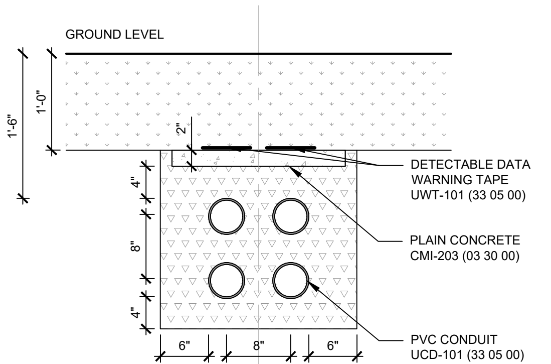
09 DATA - NON-PAVED/SHALLOW SURFACE 1" = 1' 0 6" 1' 2'
