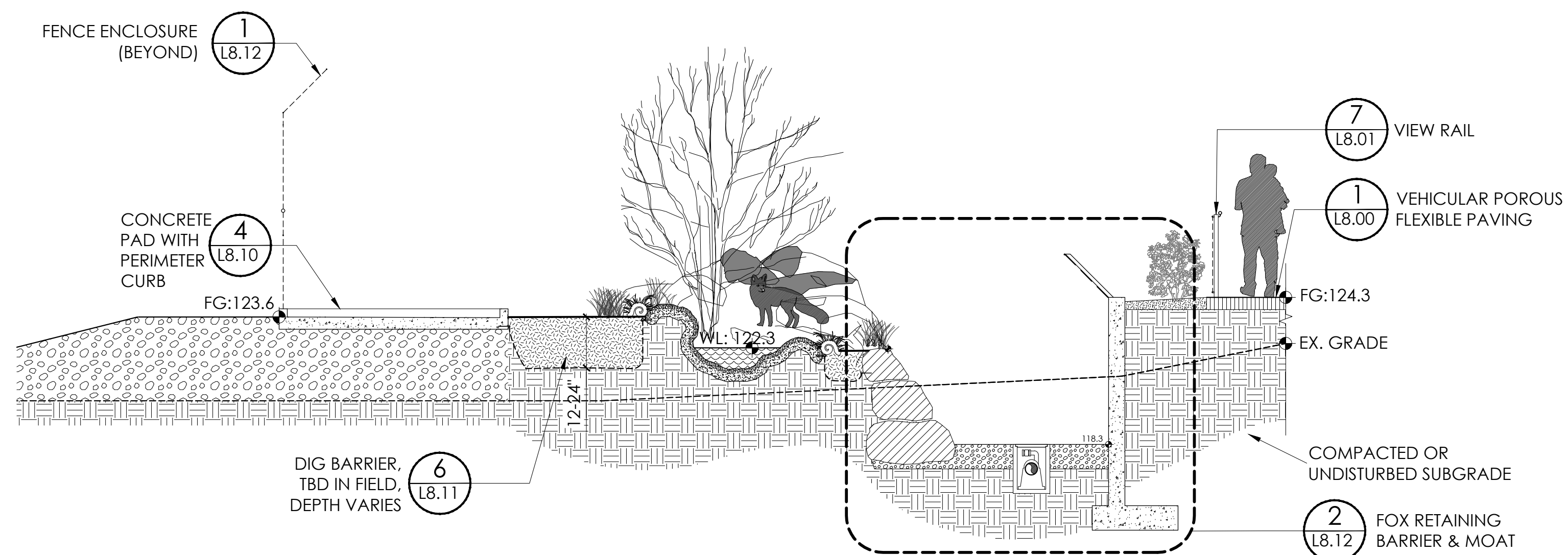
2 SECTION AT FOX HABITAT - ALTERNATE #1 L7.10 SCALE: 1/4" = 1'-0"
