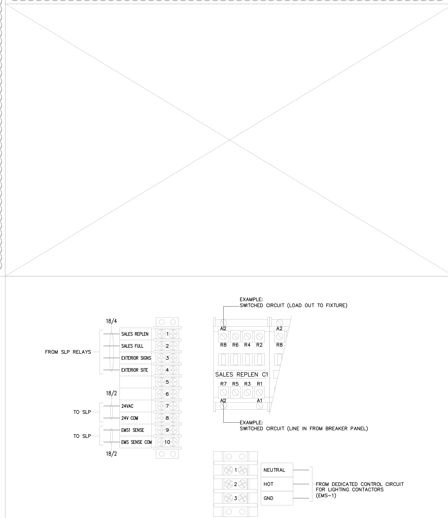
LCP LIGHTING CONTROL PANEL WIRING DETAIL 1 NO SCALE
