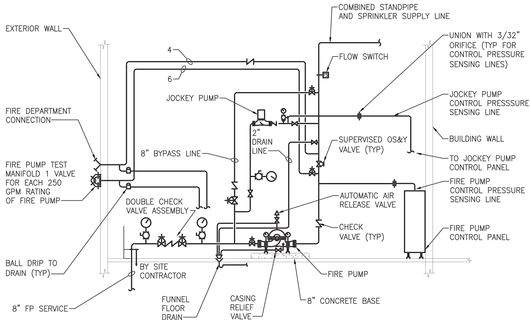
FIRE PUMP DETAIL NO SCALE
