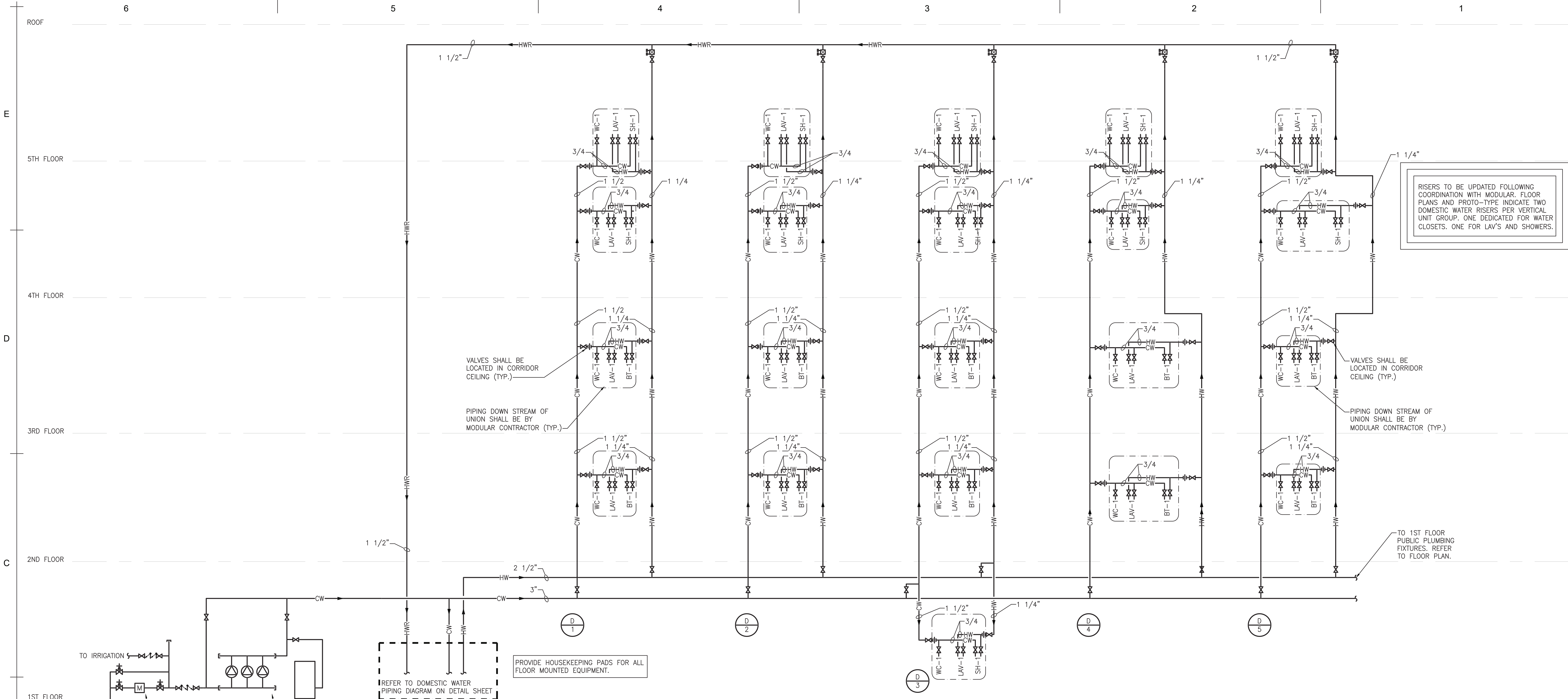
DOMESTIC WATER RISER DIAGRAM NO SCALE
