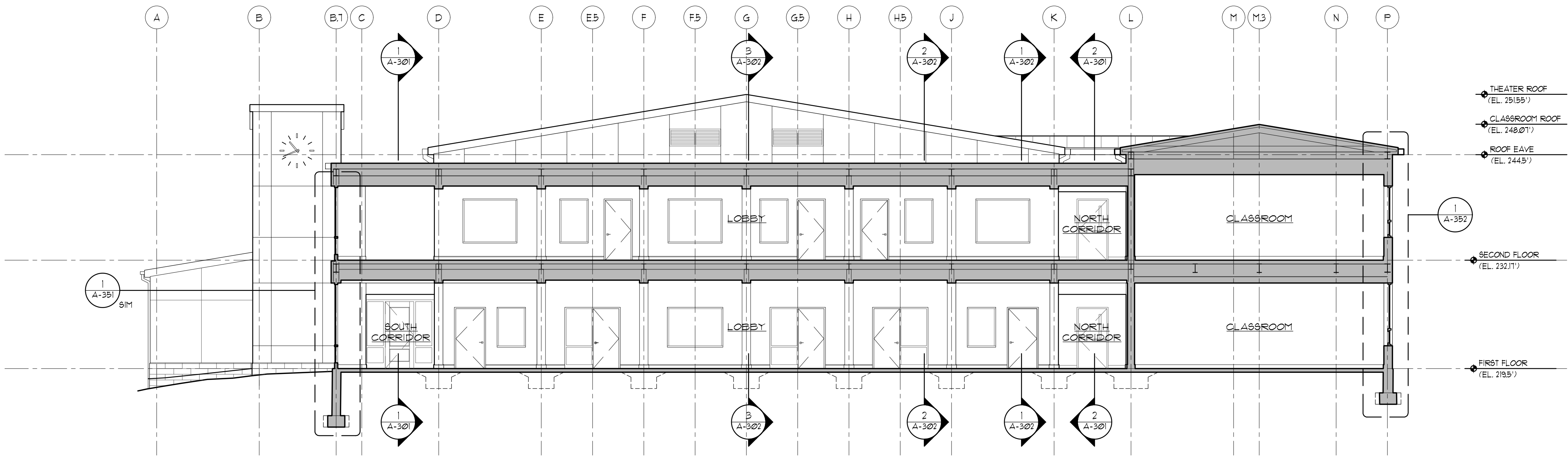
2 BUILDING SECTION BETWEEN COLUMN LINES 8 & 8.8 SCALE: 1/8"=1'-0"
