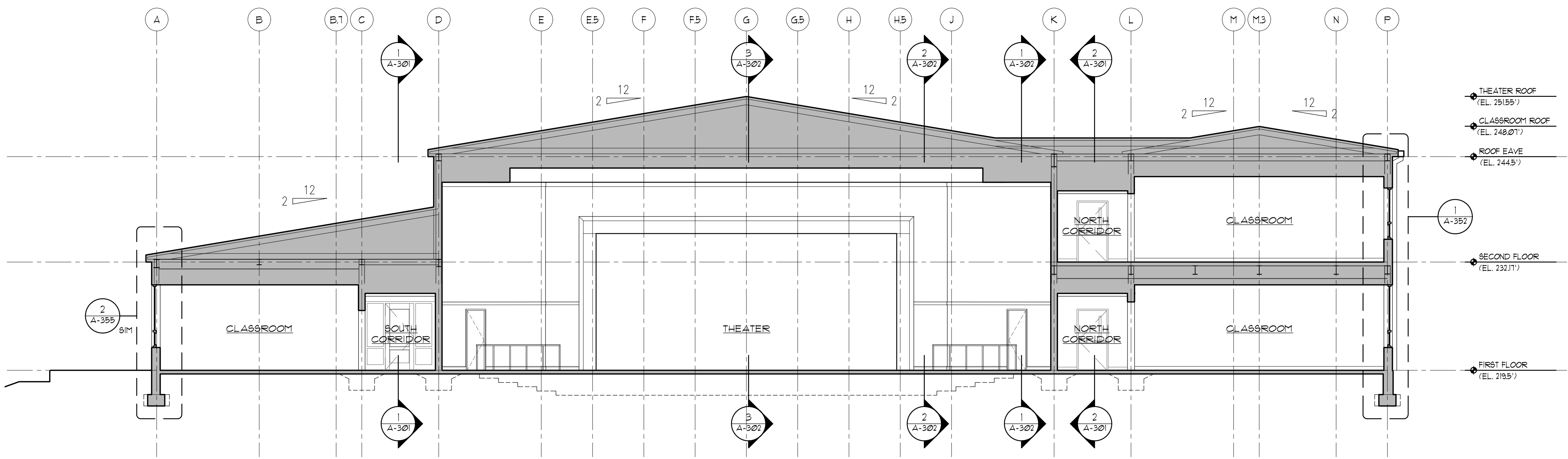
1 BUILDING SECTION BETWEEN COLUMN LINES 5 & 6 SCALE: 1/8"=1'-0"
