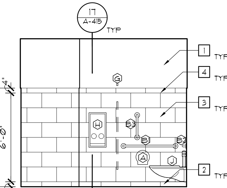
6 WOMEN'S RESTRM ELEV. SCALE: 1/4"=1'-0"
