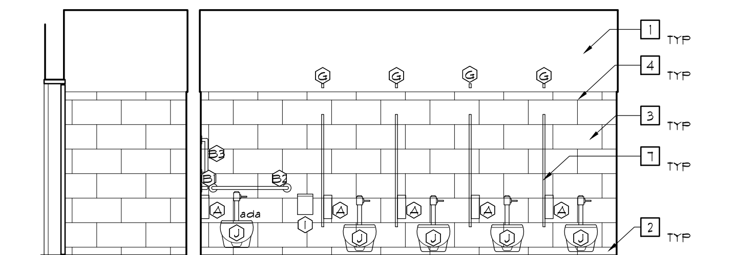
7 WOMEN'S RESTRM ELEV. SCALE: 1/4"=1'-0"
