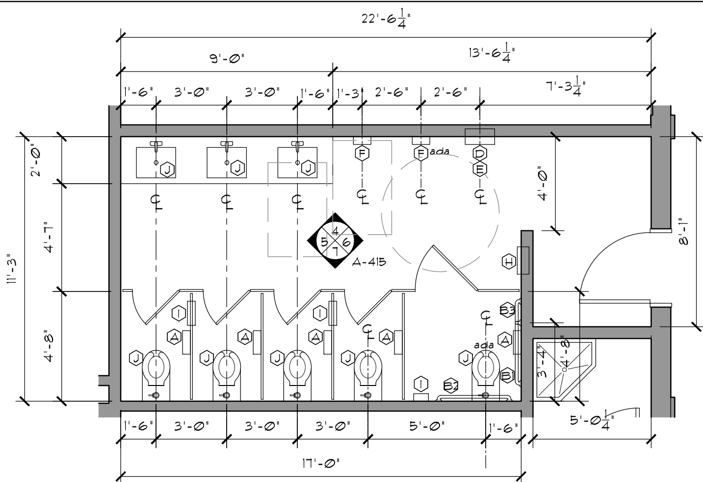
1 WOMEN'S RESTROOM (ROOM 128) PARTIAL PLAN SCALE: 1/4"=1'-0"
