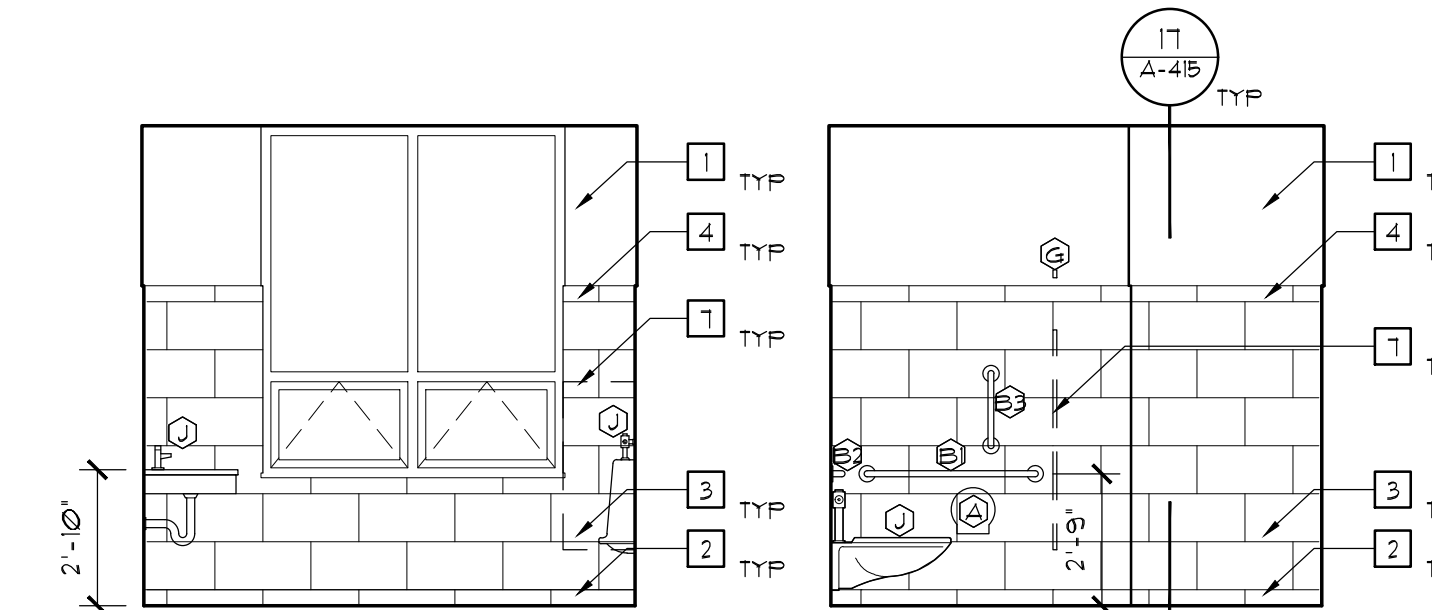
9 MEN'S RESTRM ELEV. SCALE: 1/4"=1'-0"
