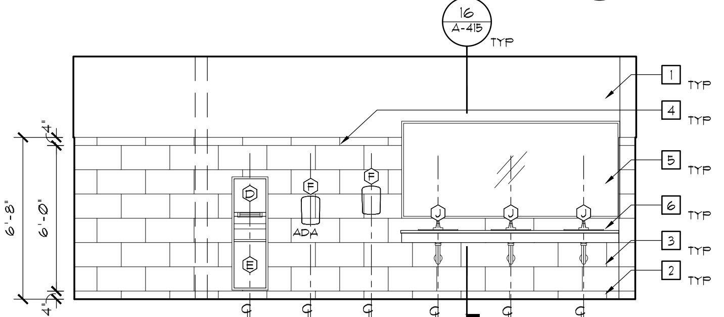
8 MEN'S RESTRM ELEV. SCALE: 1/4"=1'-0"
