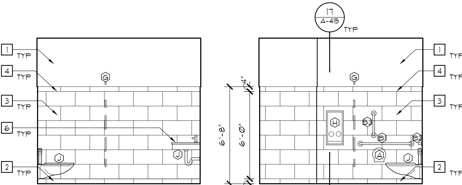
5 WOMEN'S RESTRM ELEV. SCALE: 1/4"=1'-0"
