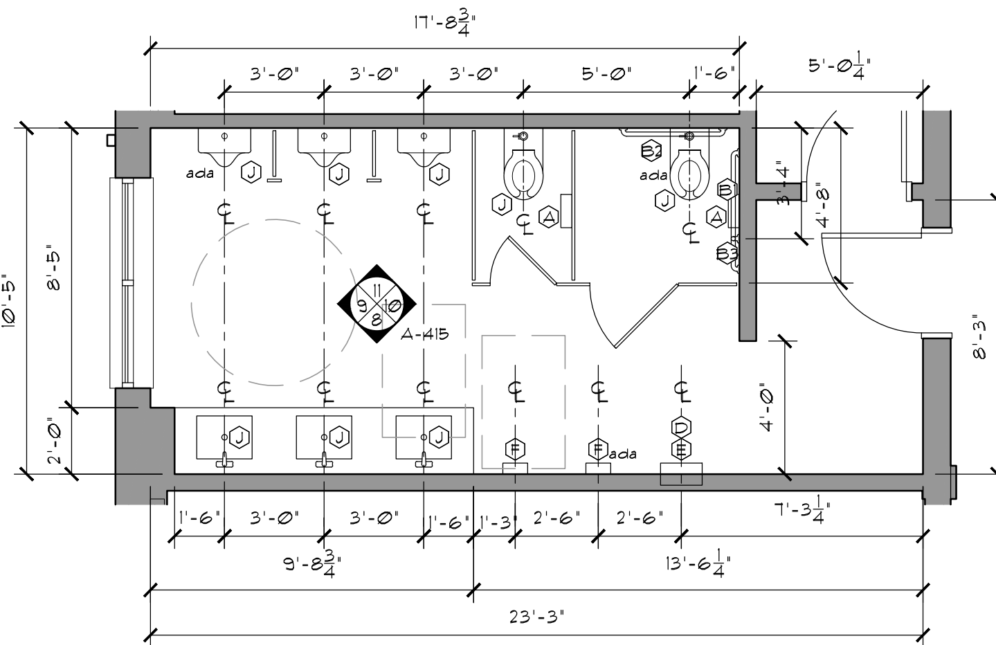
2 MEN'S RESTROOM (ROOM 131) PARTIAL PLAN SCALE: 1/4"=1'-0"
