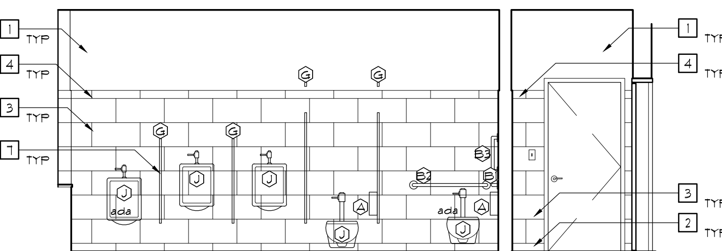
11 MEN'S RESTRM ELEV. SCALE: 1/4"=1'-0"
