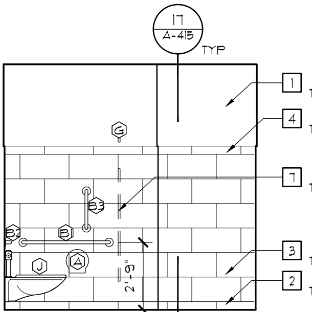
10 MEN'S RESTRM ELEV. SCALE: 1/4"=1'-0"
