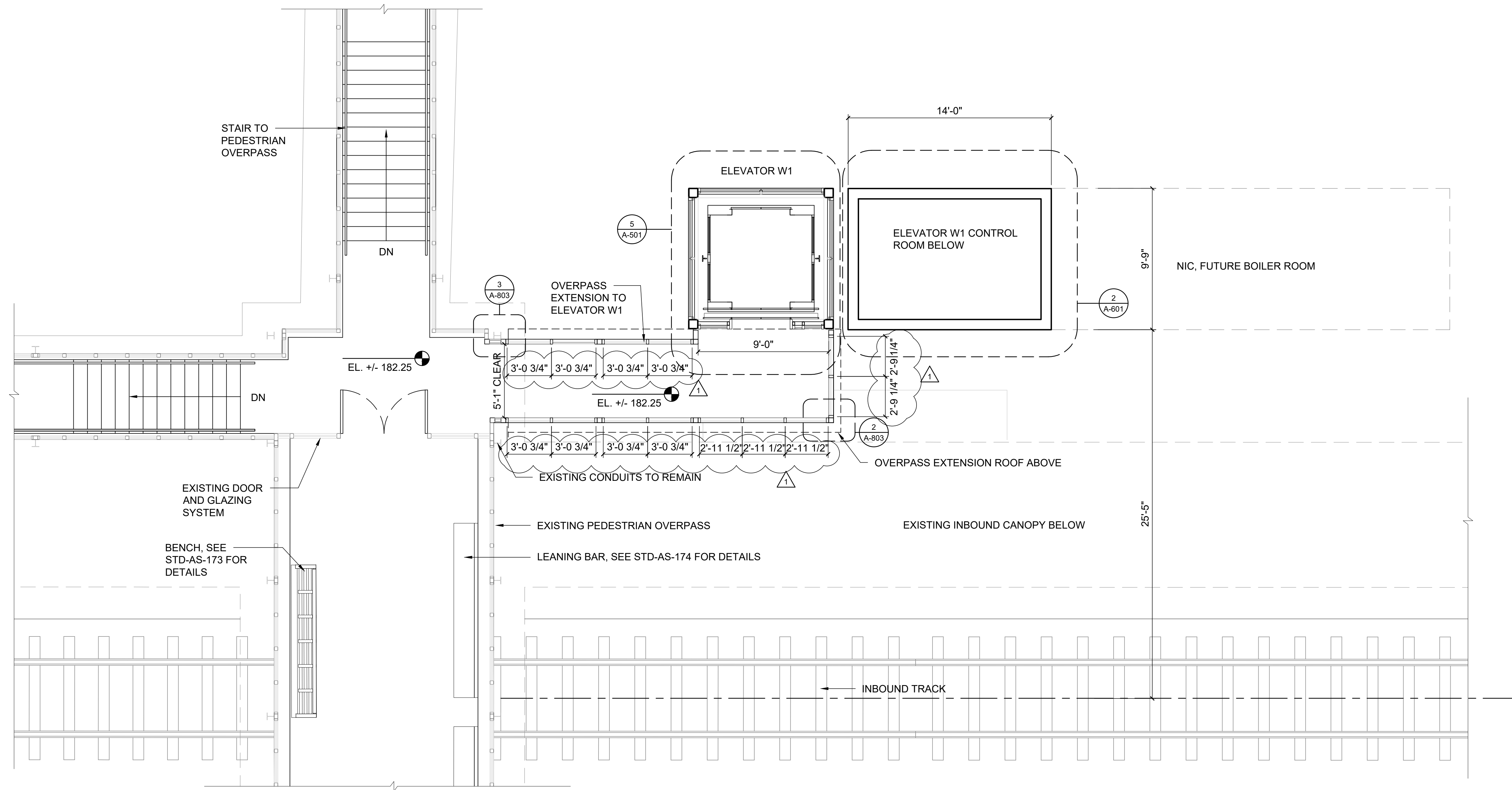
1 STATION ENLARGED INBOUND OVERPASS LEVEL PLAN A-101 1/4"=1'-0" 0 2' 4' 8'
