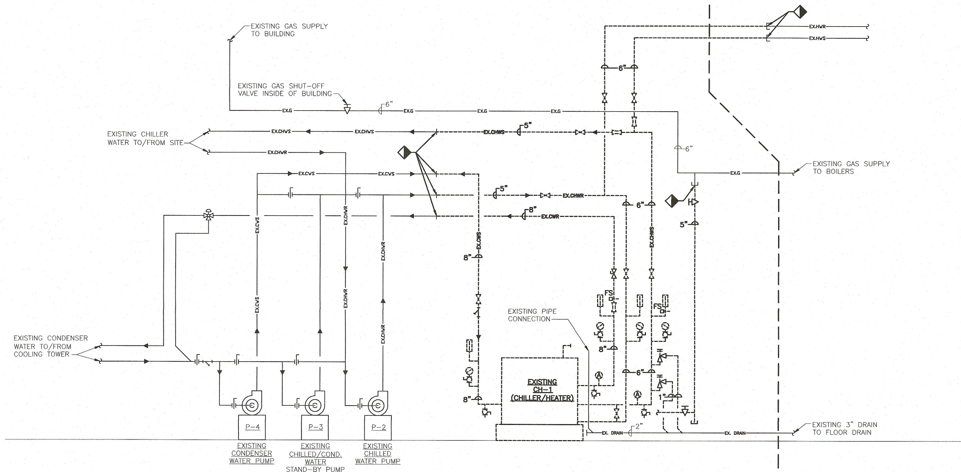
1 PARTIAL DEMOLITION FLOW DIAGRAM N.T.S.
