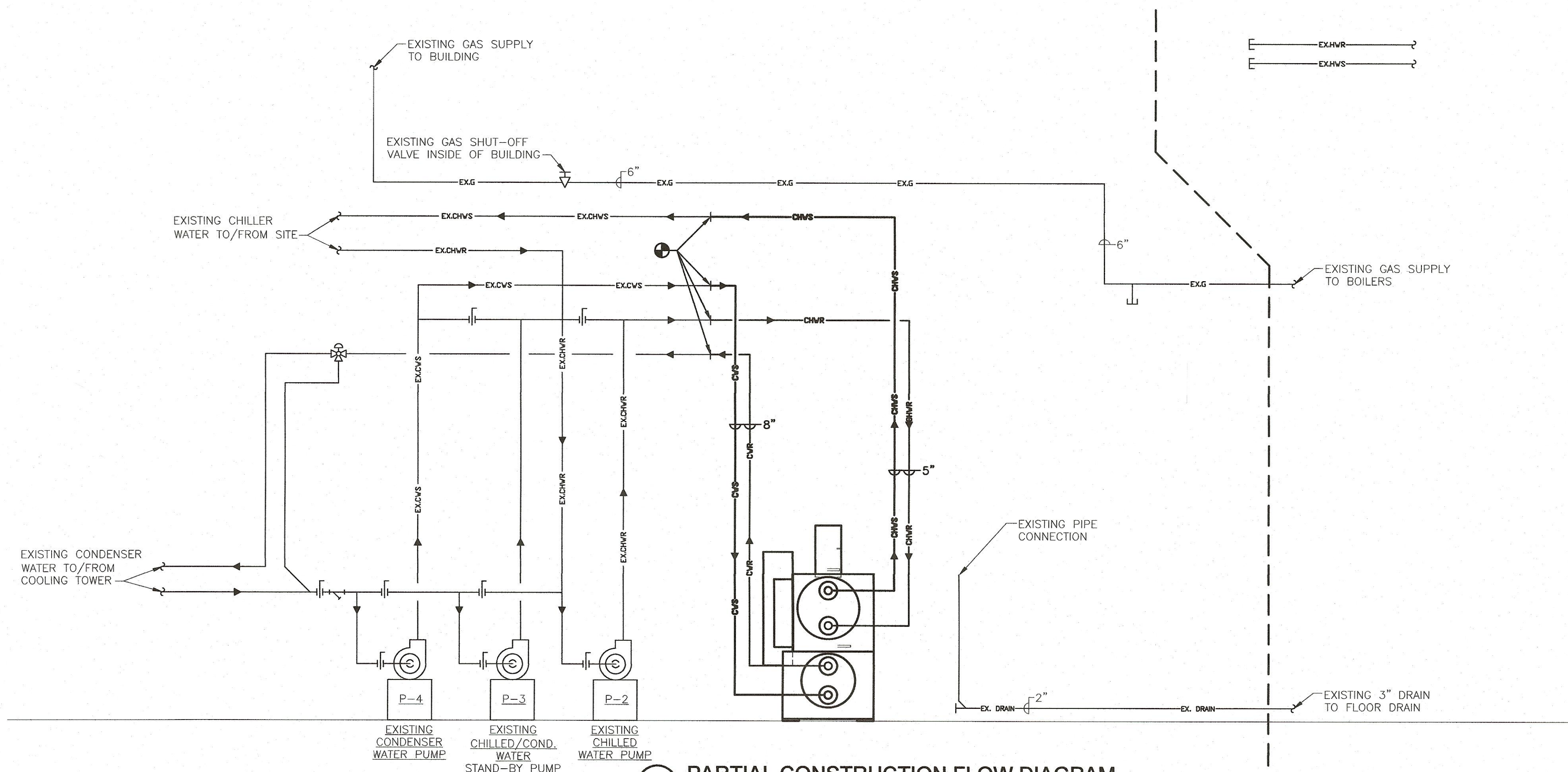
2 PARTIAL CONSTRUCTION FLOW DIAGRAM N.T.S.
