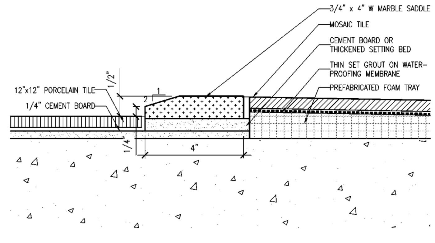
8 SHOWER EDGE DETAIL SCALE 1/2" = 1'-0"
