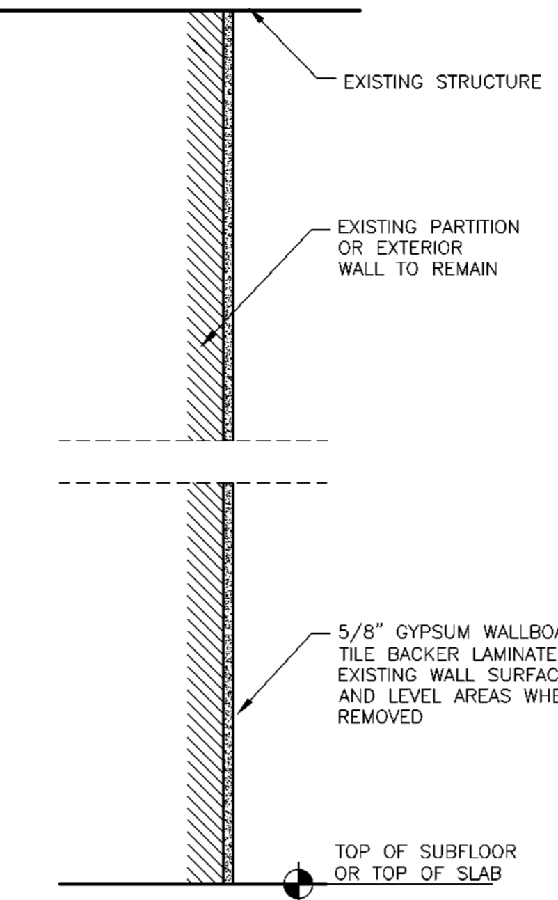
3 LAMINATED WALL FINISH DETAIL SCALE 1/2" = 1'-0"
