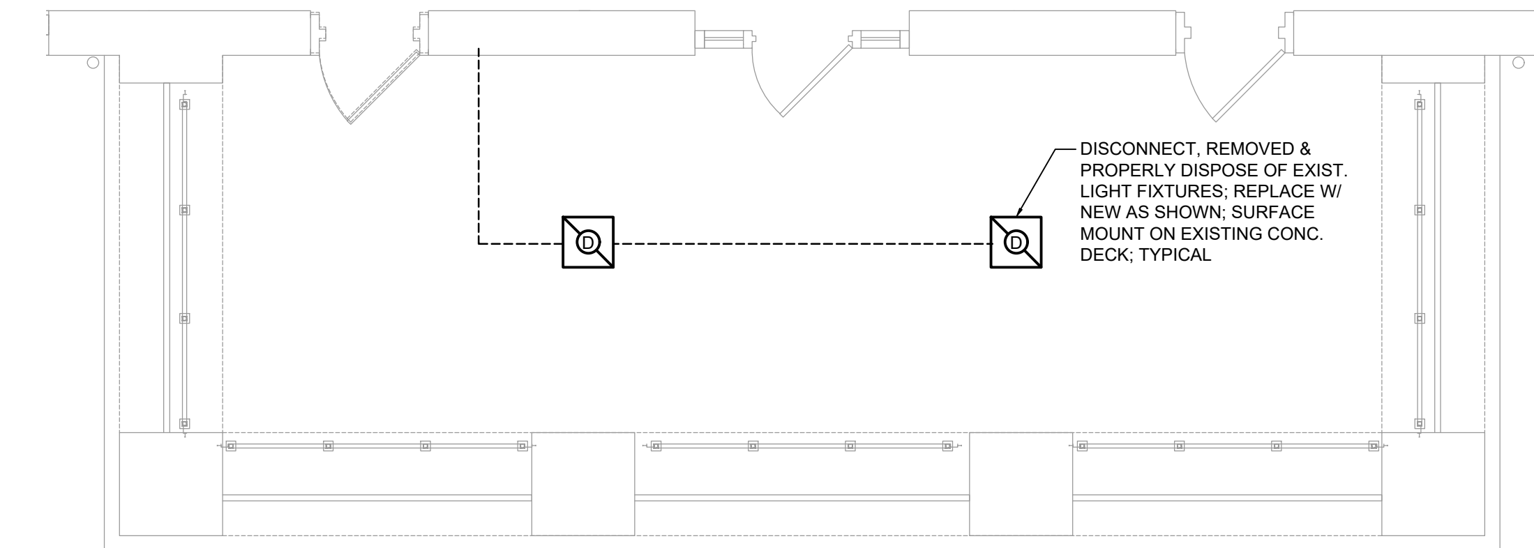
3 THIRD FLOOR PORTICO LIGHTING PLAN SCALE: 1/4" = 1'-0"
