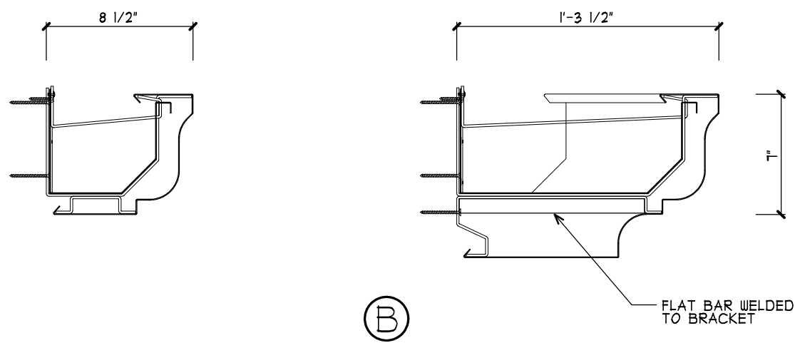
3 COLLECTION BOX DETAIL A-106 SCALE: 1-1/2" = 1'-0"
