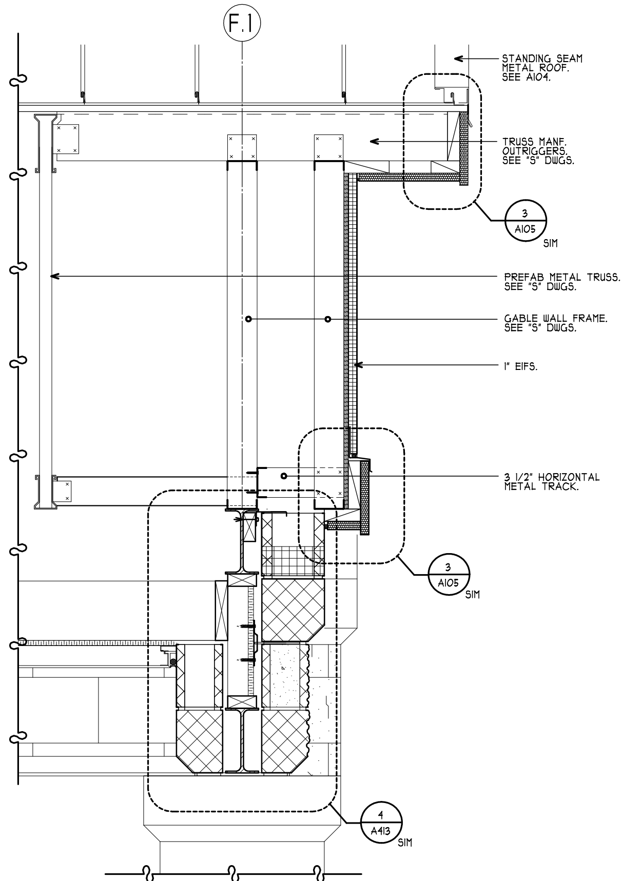
4 GABLE END WALL SECTION A106 SCALE: 1" = 1'-0" 1/A104
