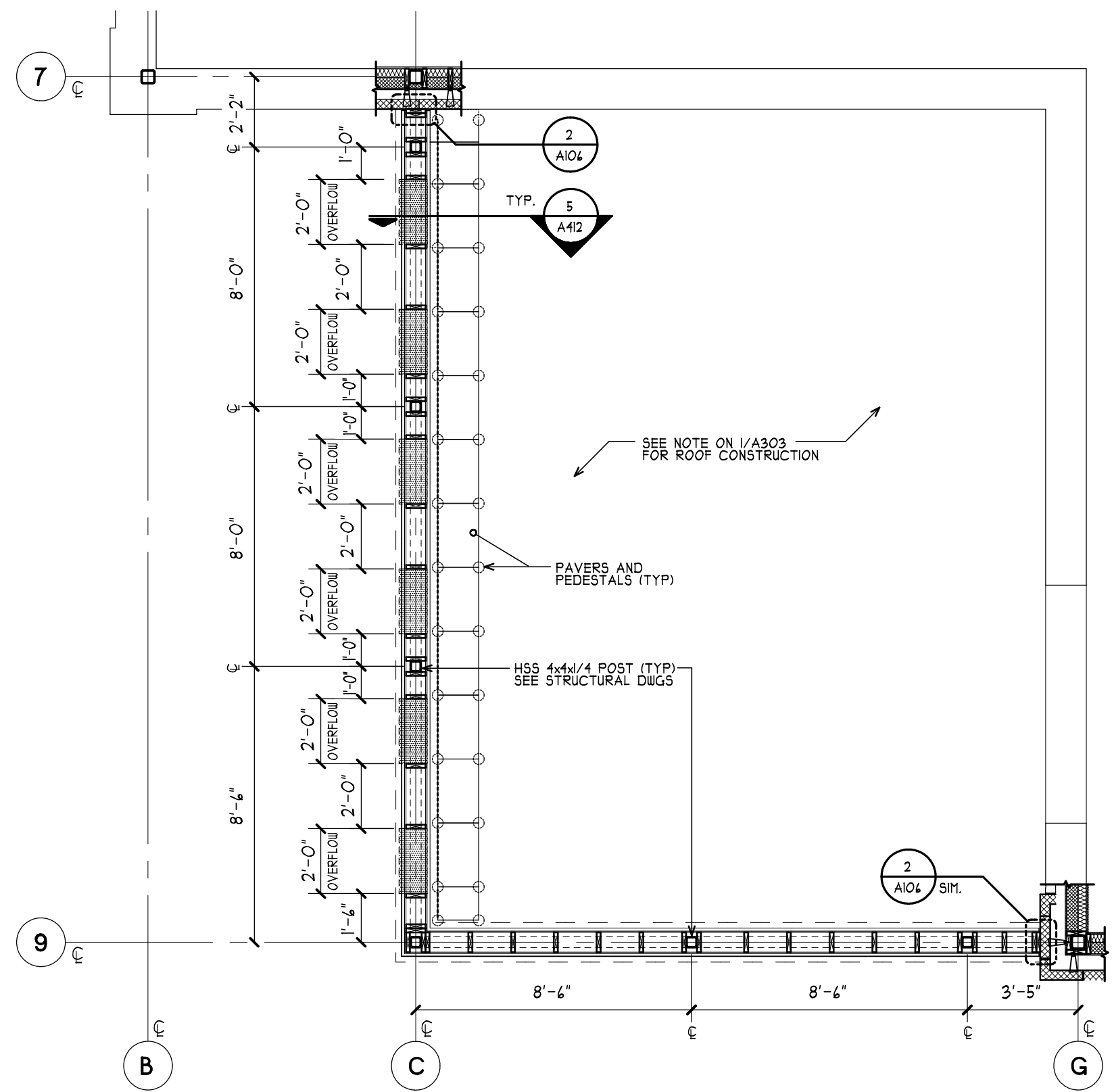
1 PATIO OVERFLOW SCUPPER FRAMING PLAN A106 SCALE: 1/4" = 1'-0"
