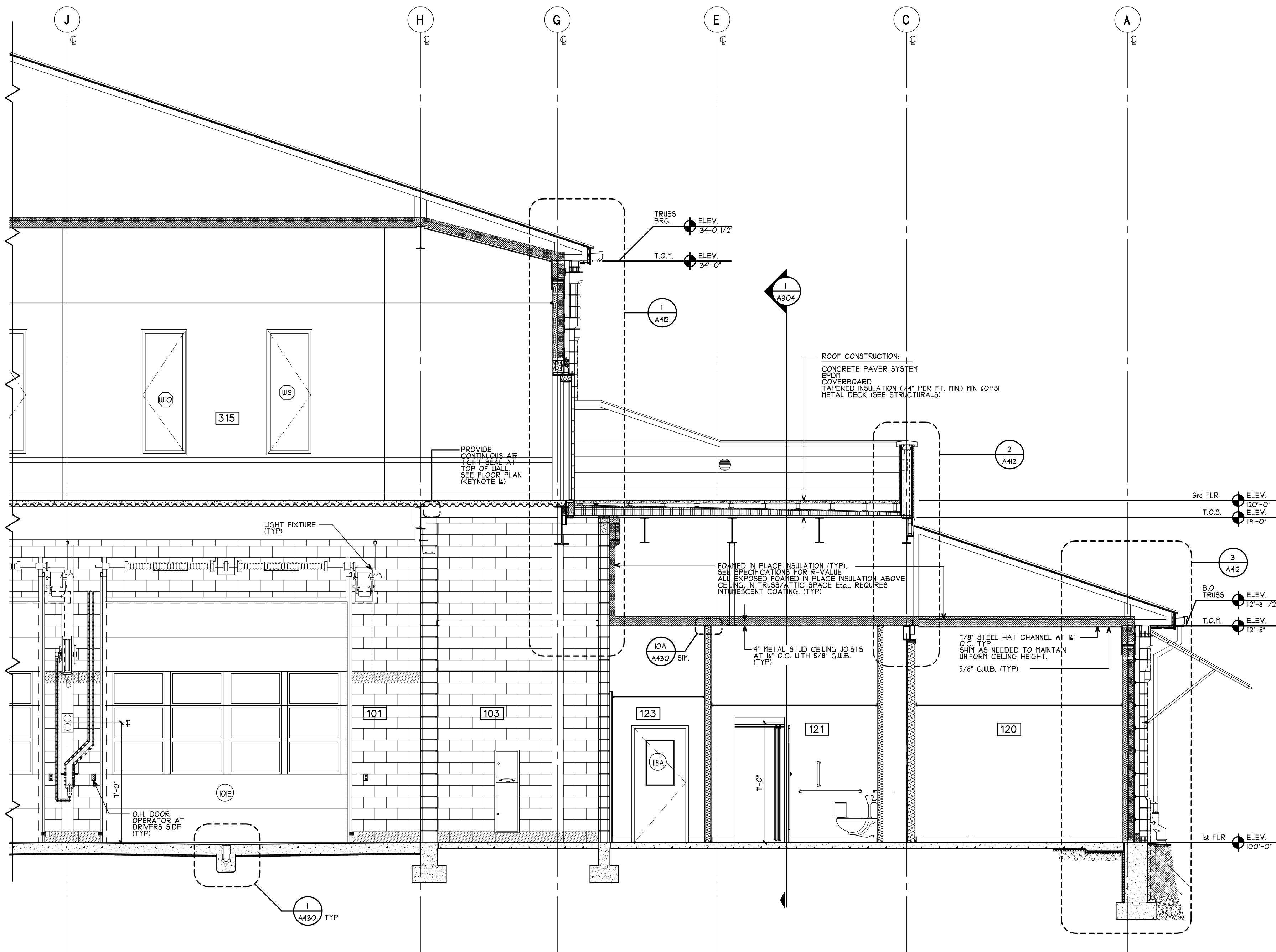
1 BUILDING SECTION A303 SCALE: 1/4" = 1'-0"
