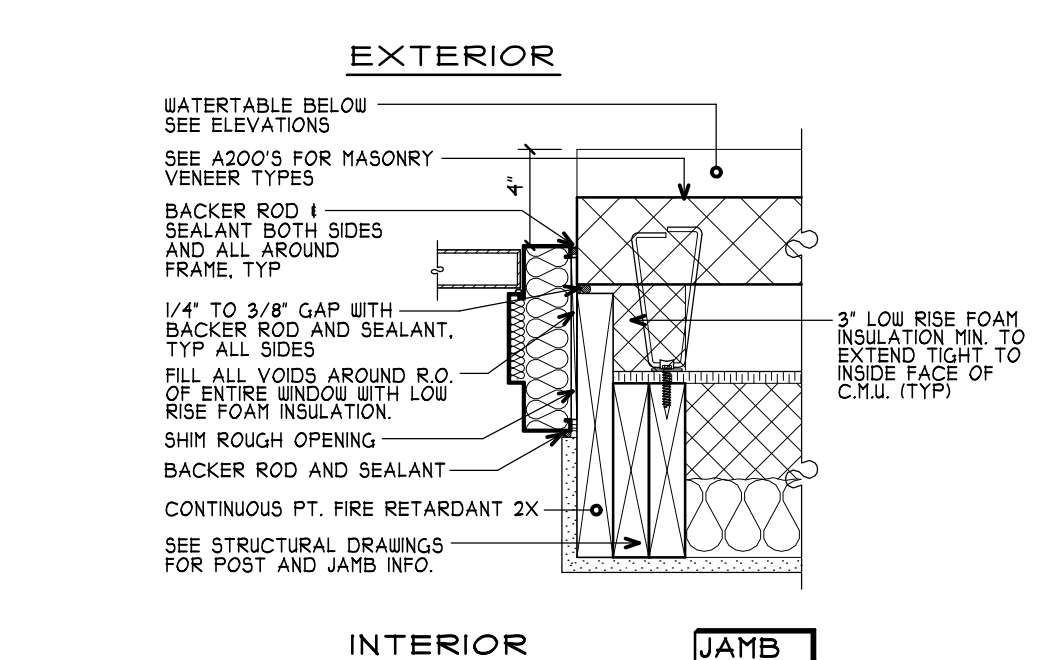
3 A500 TYP. H.M. DOOR FRAME AT EXT. STUD WALL W/ MASONRY VENEER SCALE: 1 1/2" = 1'-0"
