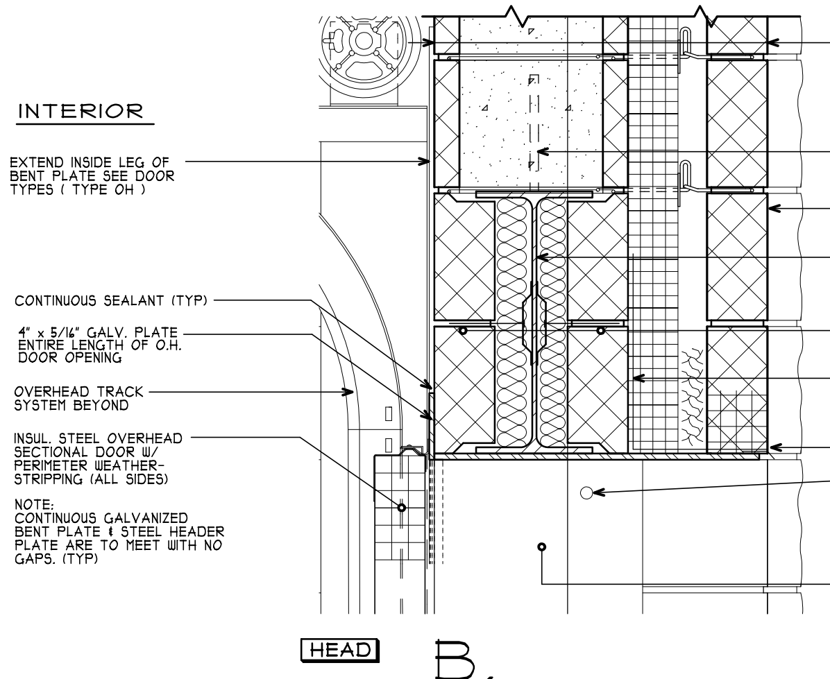
9 A500 TYP. H.M. DOOR FRAME AT EXTERIOR STUD WALL W/ MASONRY VENEER SCALE: 1 1/2" = 1'-0"
