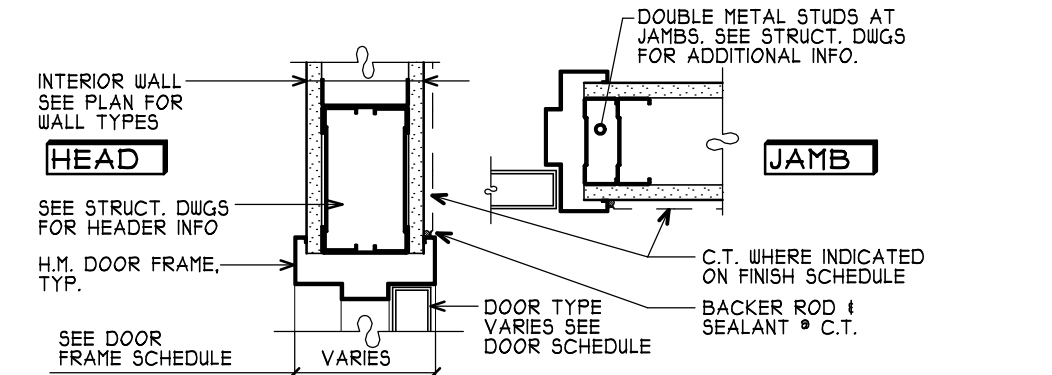
4 A500 TYP. H.M. DOOR FRAME AT INTERIOR STUD WALLS SCALE: 1 1/2" = 1'-0"
