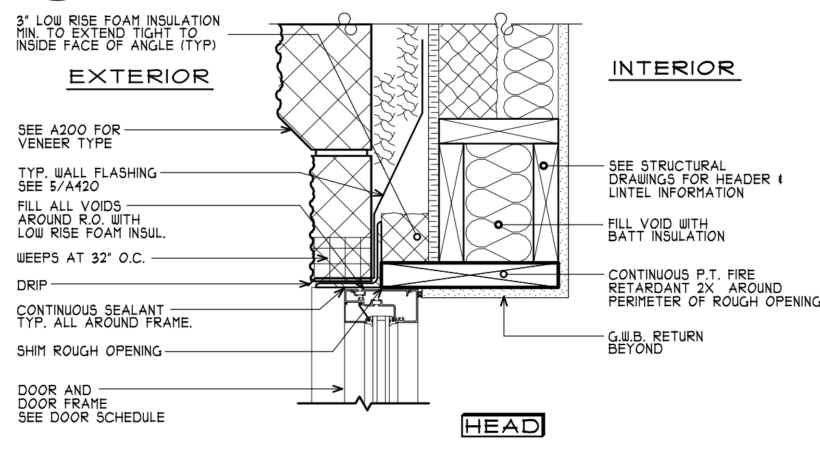
5 A500 TYP. H.M. DOOR FRAME AT EXTERIOR DOUBLE WYTHE MASONRY WALLS SCALE: 1 1/2" = 1'-0"
