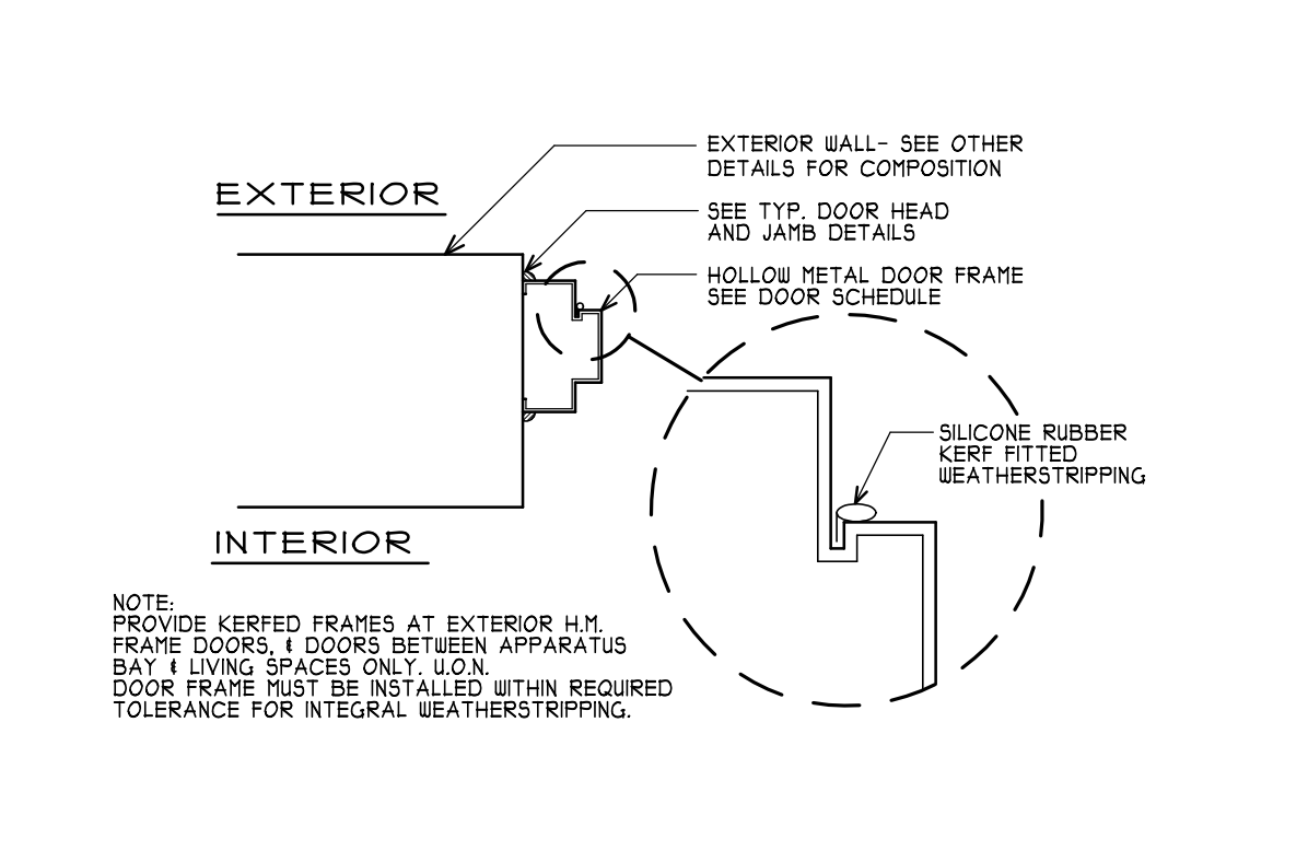
1 A500 TYP. KERF WEATHERSTRIPPING SCALE: 1 1/2" = 1'-0"
