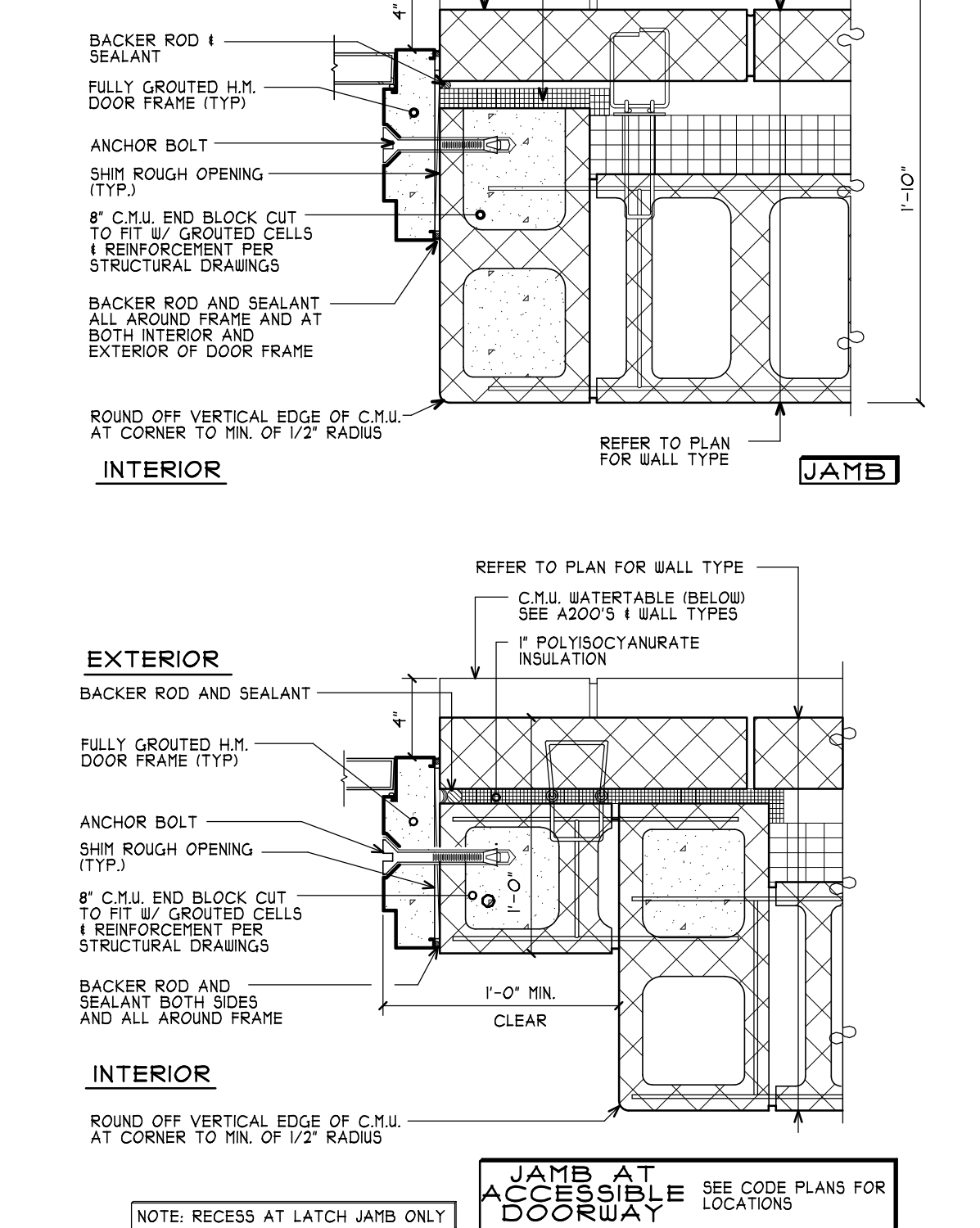
5 A500 TYP. H.M. DOOR FRAME AT EXTERIOR DOUBLE WYTHE MASONRY WALLS SCALE: 1 1/2" = 1'-0"
