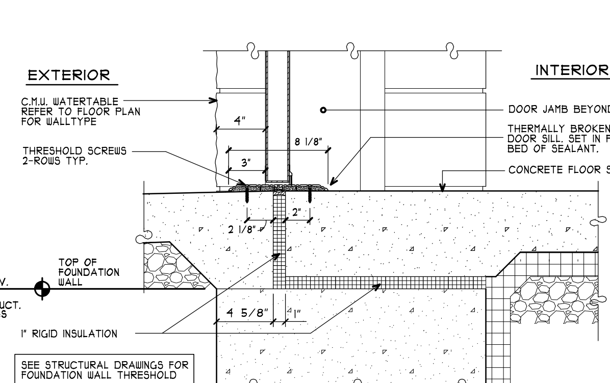
8A A500 TYP. H.M. DOOR FRAME AT EXTERIOR STUD WALL W/ MASONRY VENEER SCALE: 1 1/2" = 1'-0"
