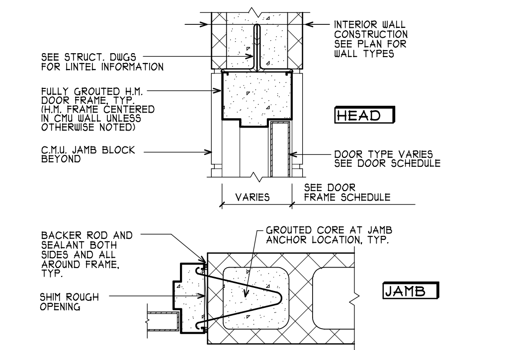
1 A500 TYP. H.M. DOOR FRAME AT INTERIOR MASONRY WALLS SCALE: 1 1/2" = 1'-0"
