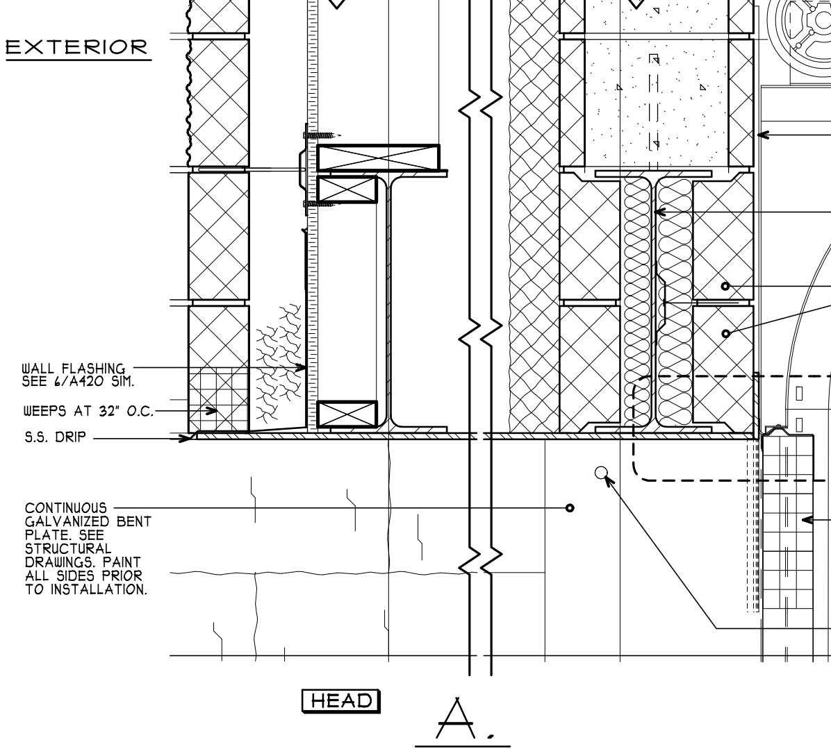
5 A500 TYP. H.M. DOOR FRAME AT EXTERIOR DOUBLE WYTHE MASONRY WALLS SCALE: 1 1/2" = 1'-0"
