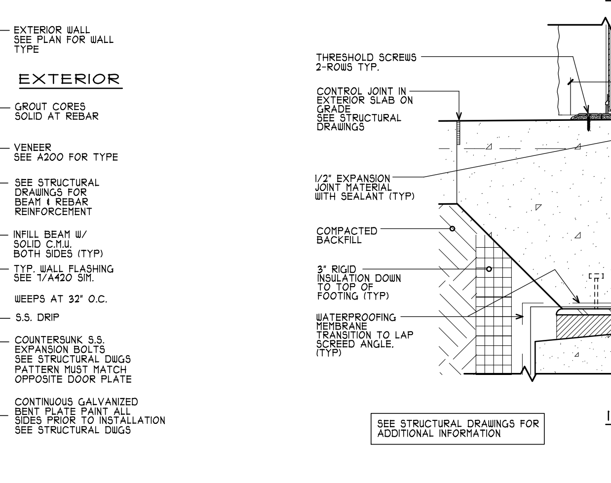
9 A500 TYP. H.M. DOOR FRAME AT EXTERIOR STUD WALL W/ MASONRY VENEER SCALE: 1 1/2" = 1'-0"
