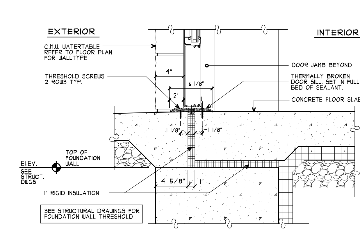
8B A500 TYP. H.M. DOOR FRAME AT EXTERIOR STUD WALL W/ MASONRY VENEER SCALE: 1 1/2" = 1'-0"
