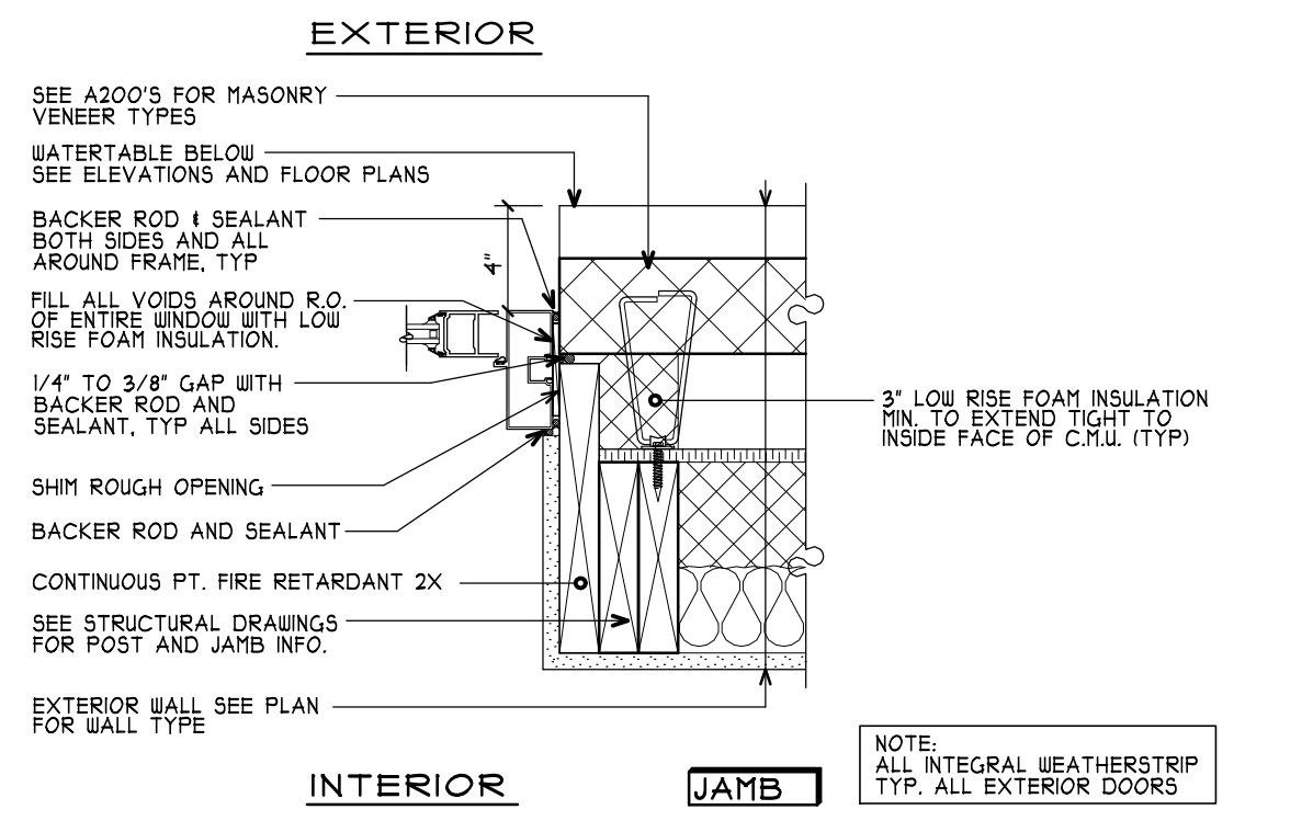
6 A500 TYP. ALUMINUM DOOR FRAME AT EXTERIOR STUD WALL W/ MASONRY VENEER SCALE: 1 1/2" = 1'-0"
