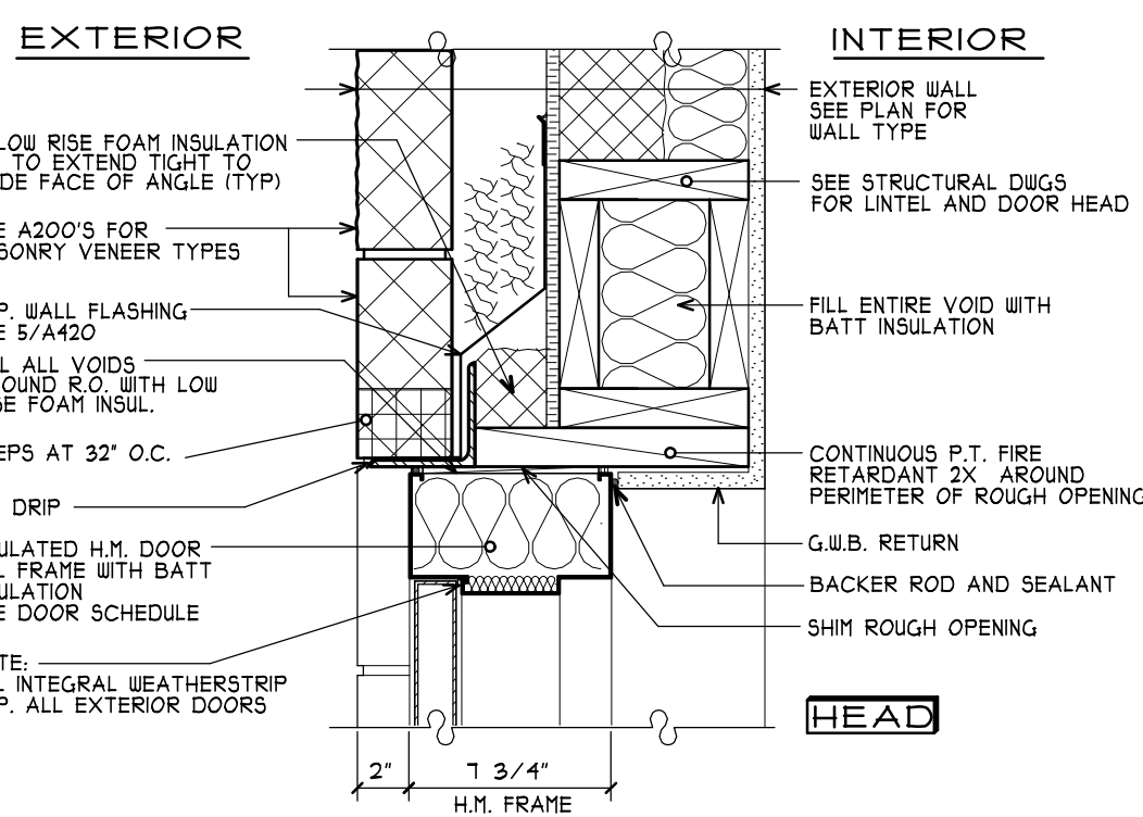
5 A500 TYP. H.M. DOOR FRAME AT EXTERIOR DOUBLE WYTHE MASONRY WALLS SCALE: 1 1/2" = 1'-0"
