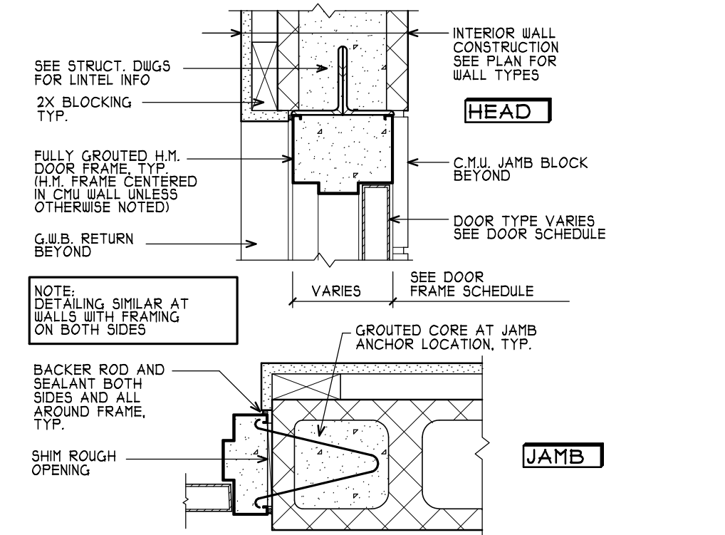
2 A500 TYP. H.M. DOOR AT INT. MASONRY WALLS W/ FURRING & G.W.B. ON SIDE SCALE: 1 1/2" = 1'-0"
