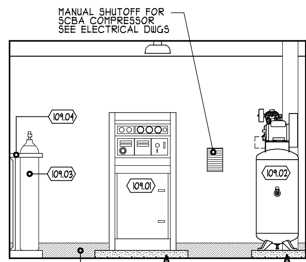
6 ELEVATIONS (ROOM 109) A711 SCALE: 1/4" = 1'-0"
