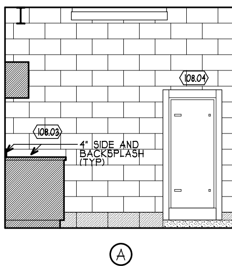
1 ELEVATIONS (ROOM 108) A711 SCALE: 1/4" = 1'-0"
