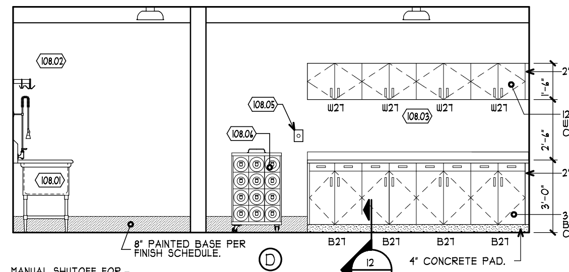
8A EXTRACTOR ELEVATION (ROOM 107) A711 SCALE: 1/4" = 1'-0"
