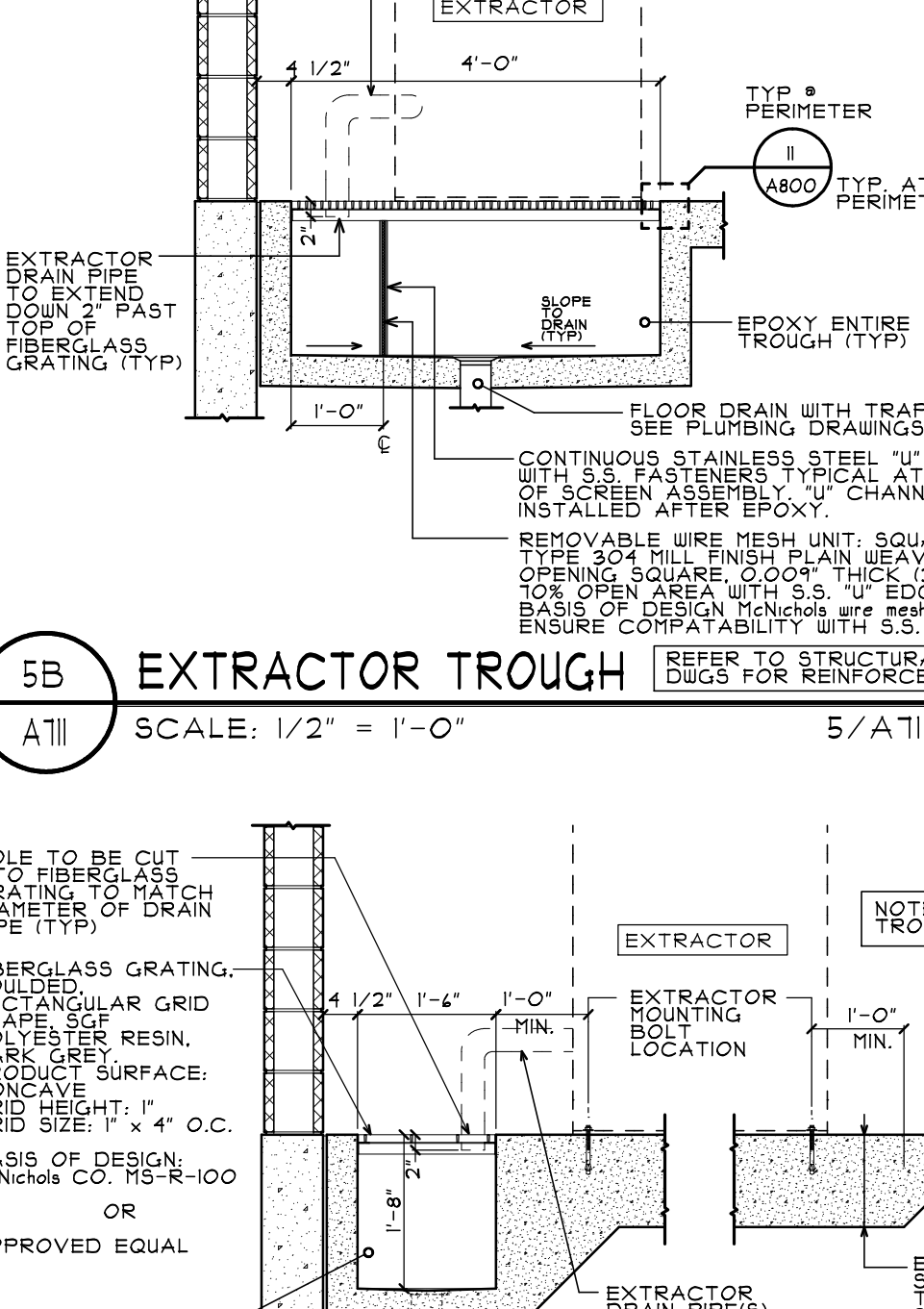
5A EXTRACTOR TROUGH A711 SCALE: 1/2" = 1'-0"
