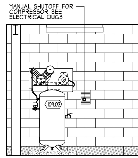
6 ELEVATIONS (ROOM 109) A711 SCALE: 1/4" = 1'-0"
