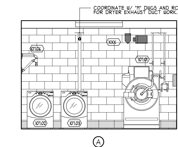
8 ELEVATIONS (ROOM 107) A711 SCALE: 1/4" = 1'-0"
