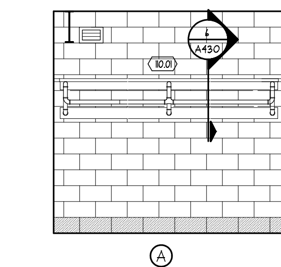
2 ELEVATIONS (ROOM 110) A711 SCALE: 1/4" = 1'-0"
