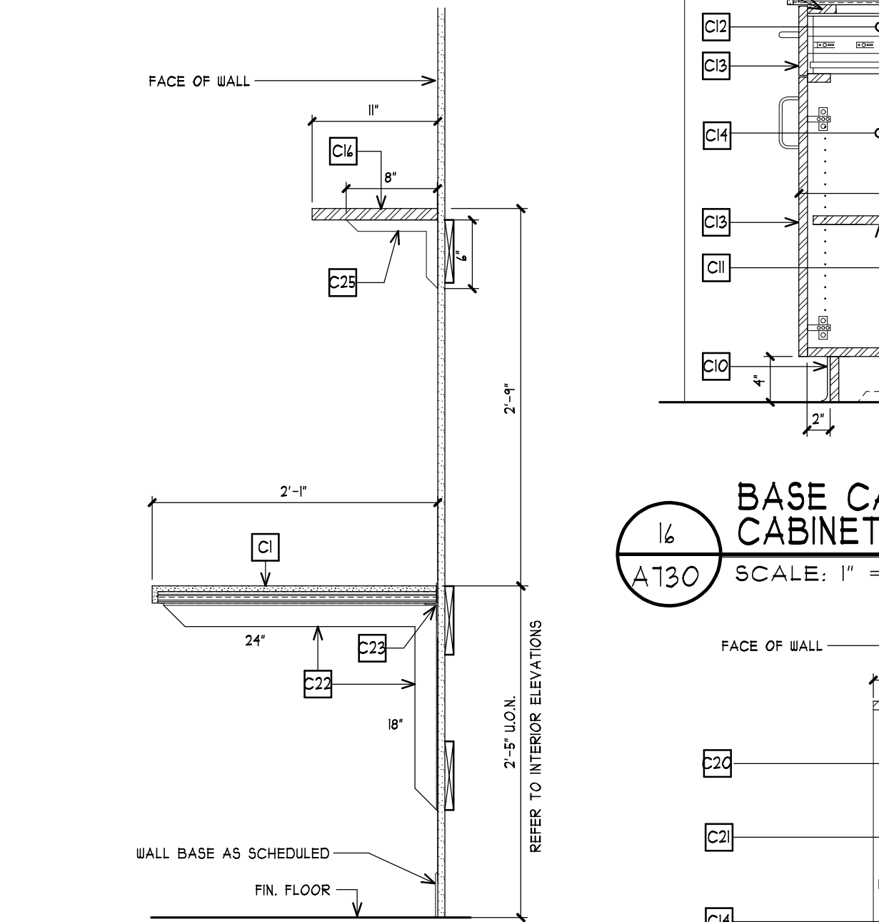
12 WORK SURFACE W/ SUPPORT BRACKET & OPEN SHELF A130 SCALE: 1" = 1'-0" 1/A102 ROOM 313
