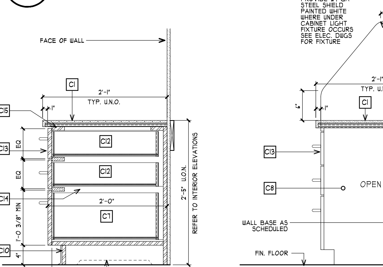
12 WORK SURFACE W/ SUPPORT BRACKET & OPEN SHELF A130 SCALE: 1" = 1'-0" 1/A102 ROOM 313
