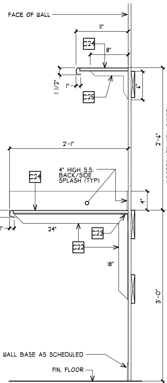
13 S.S. COUNTER W/ SHELF A130 SCALE: 1" = 1'-0" 3/A113, ROOM 309A
