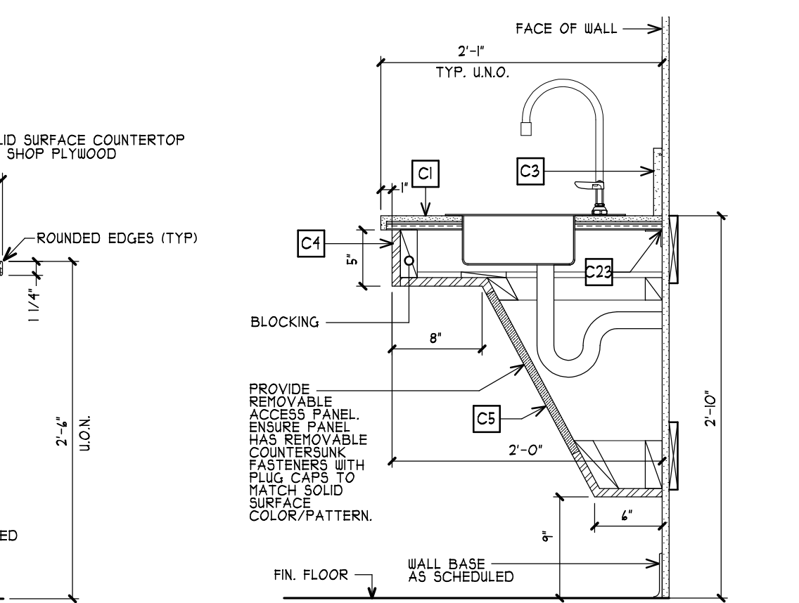
8 BASE CABINET AT ROLL UP COUNTER DOOR A130 SCALE: 1" = 1'-0" 3/A113 & 8/A112
