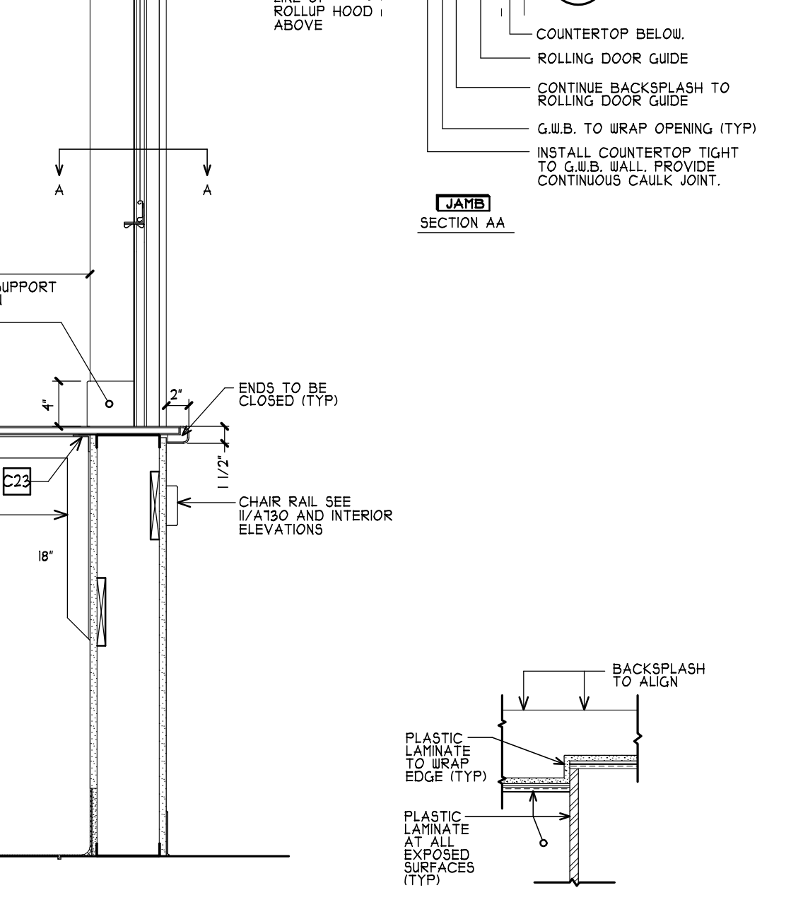
8 BASE CABINET AT ROLL UP COUNTER DOOR A130 SCALE: 1" = 1'-0" 3/A113 & 8/A112
