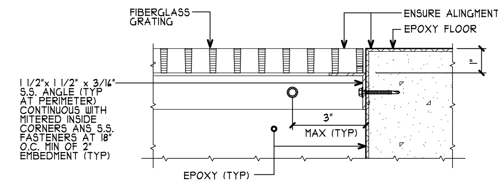
11 EPOXY TERMINATION DETAIL AT EXTRACTOR TROUGH SCALE: 3" = 1'-0"
