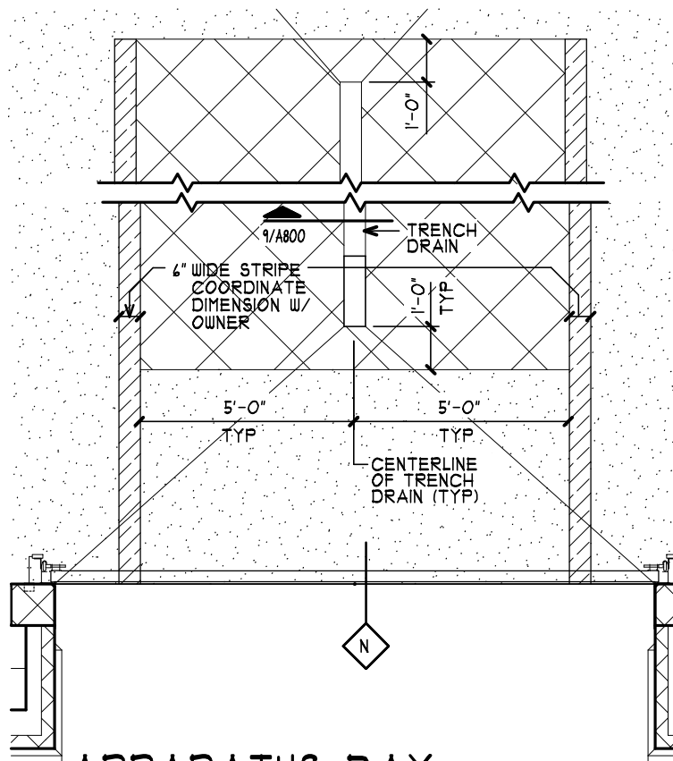
10 APPARATUS BAY EPOXY DETAILING SCALE: 1/4" = 1'-0"
