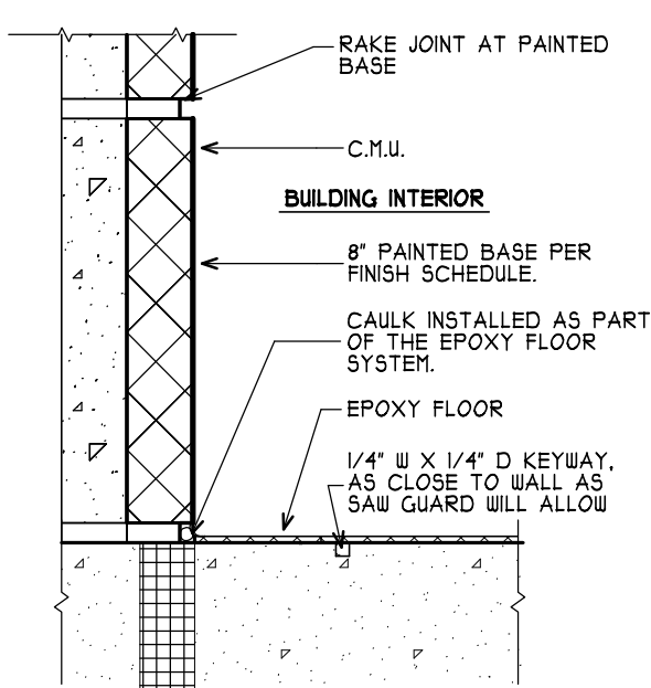
1 EPOXY @ EXTERIOR C.M.U. WALL SCALE: 3" = 1'-0"
