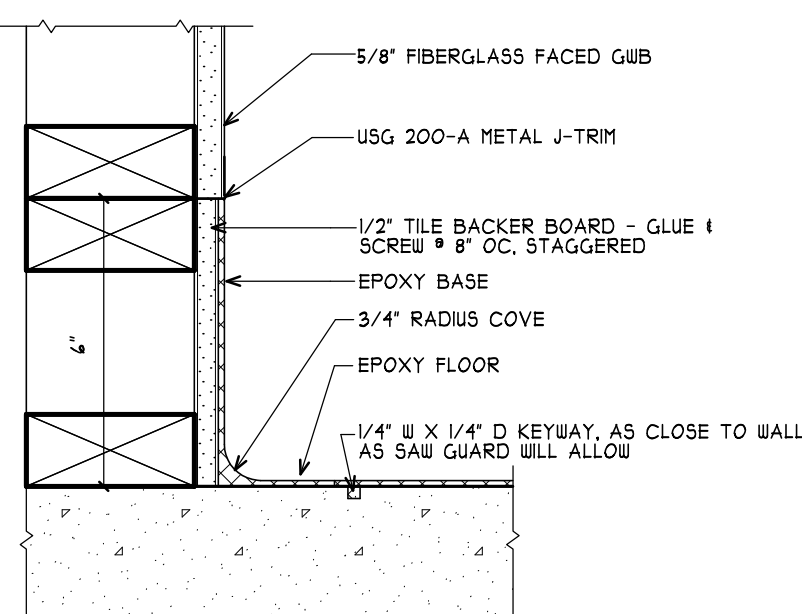
3 EPOXY COVE @ GWB SCALE: 3" = 1'-0"
