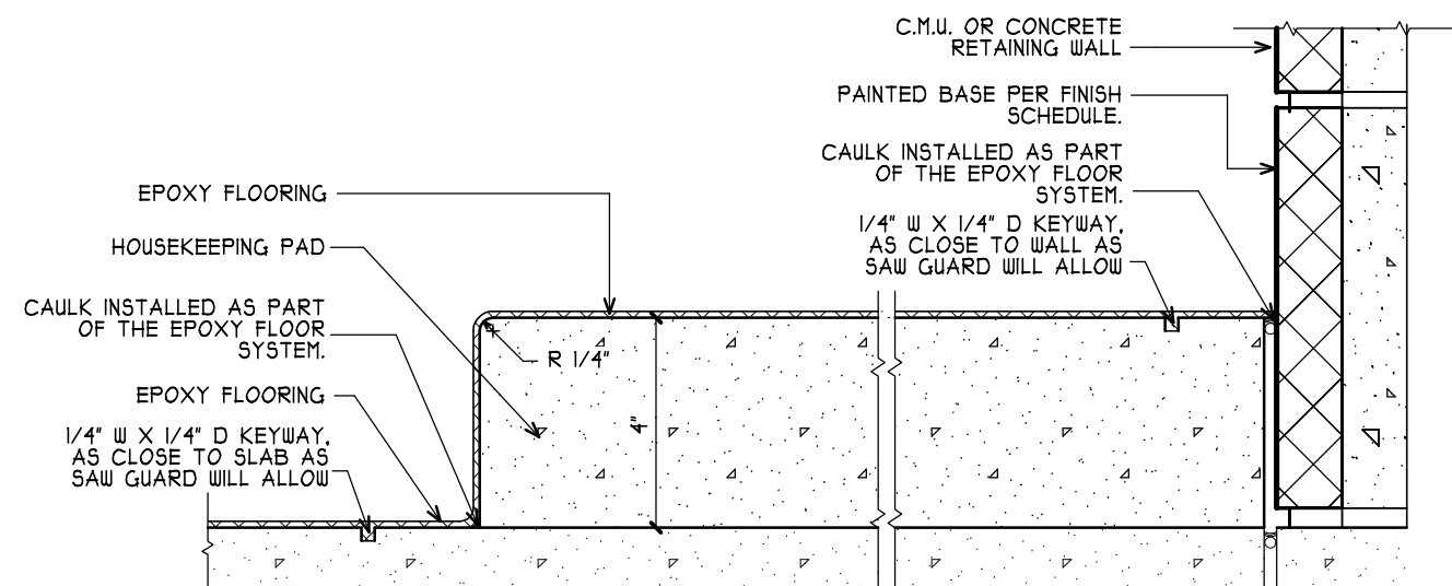
8 EPOXY @ HOUSEKEEPING PAD SCALE: 3" = 1'-0"
