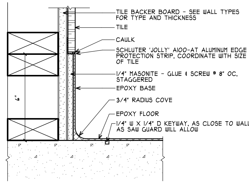
4 EPOXY COVE @ WALL TILE SCALE: 3" = 1'-0"
