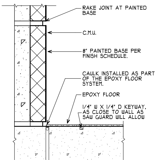
6 EPOXY @ CMU INTERIOR WALL SCALE: 3" = 1'-0"
