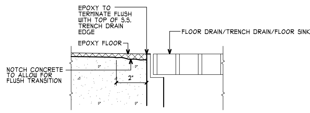
9 EPOXY TERMINATION DETAIL AT TRENCH DRAIN SCALE: 6" = 1'-0"
