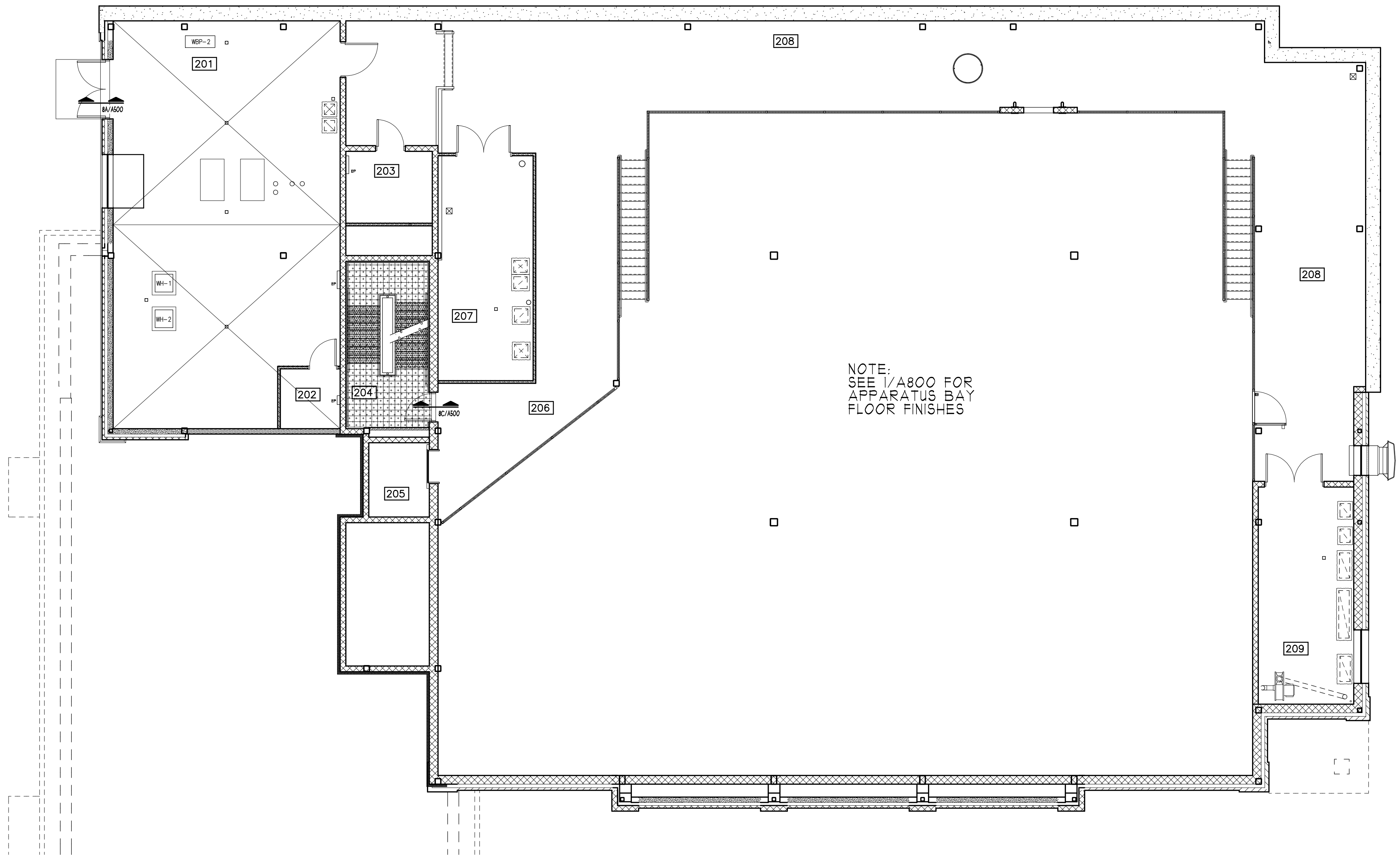
1 2nd FLOOR FINISH SCHEDULE PLAN SCALE: 1/8" = 1'-0"
