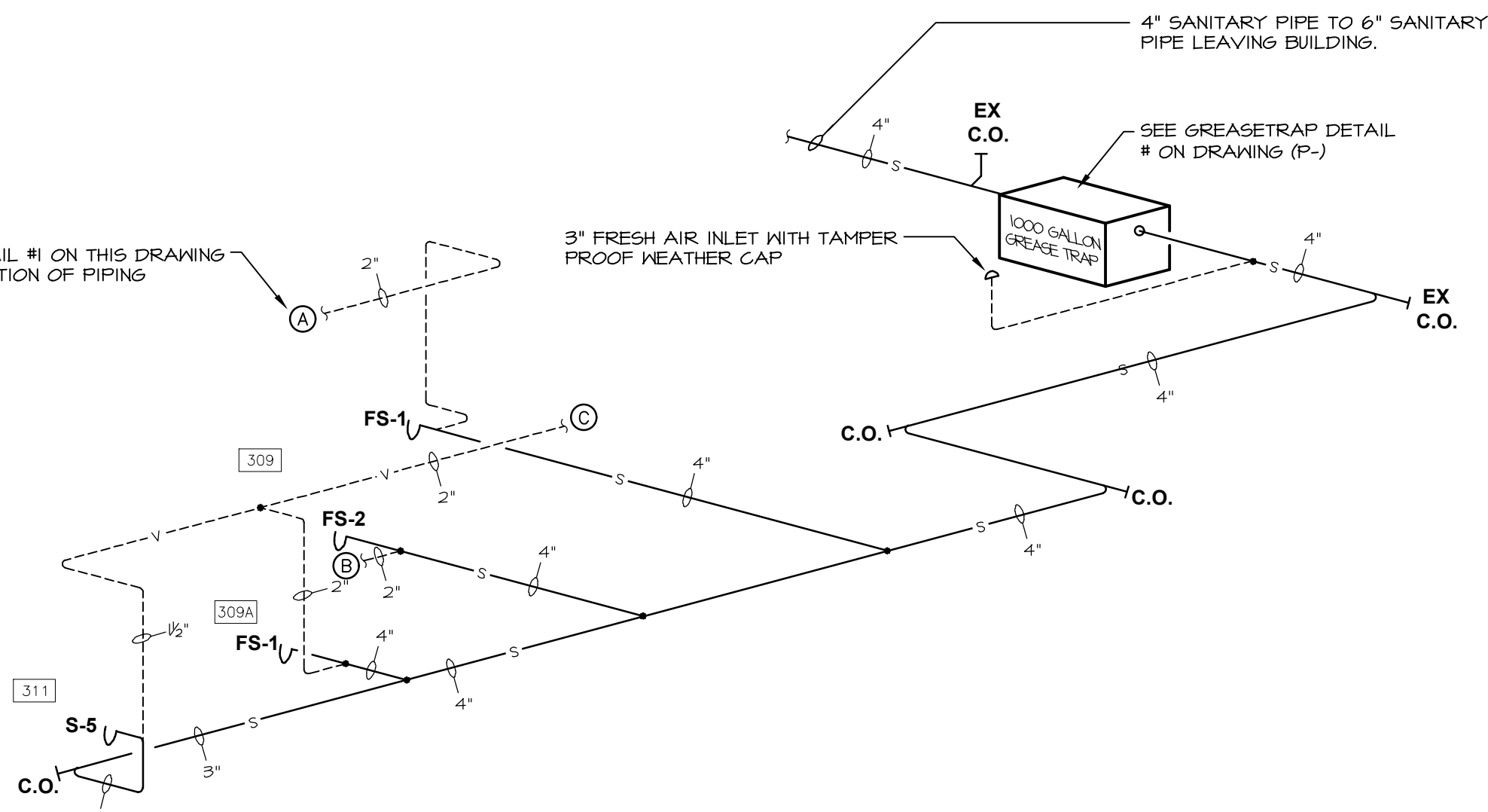
2 GREASE TRAP SANITARY/VENT PIPING ISOMETRIC P204 NOT TO SCALE
