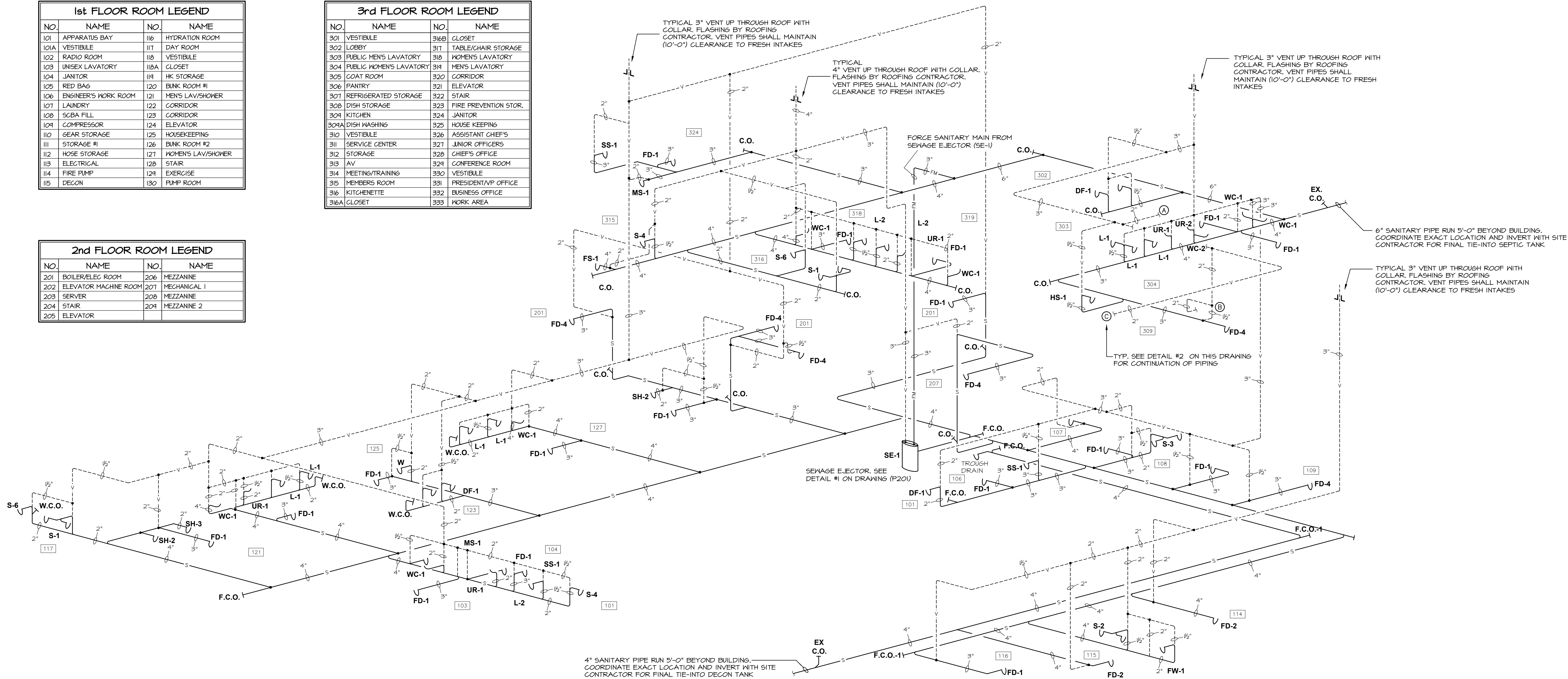
1 SANITARY/VENT PIPING ISOMETRIC P204 NOT TO SCALE
