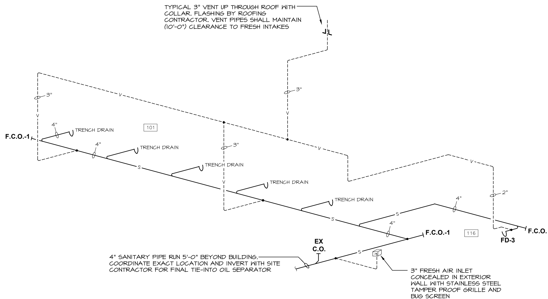
3 OIL SEPARATOR SANITARY/VENT PIPING ISOMETRIC P204 NOT TO SCALE
