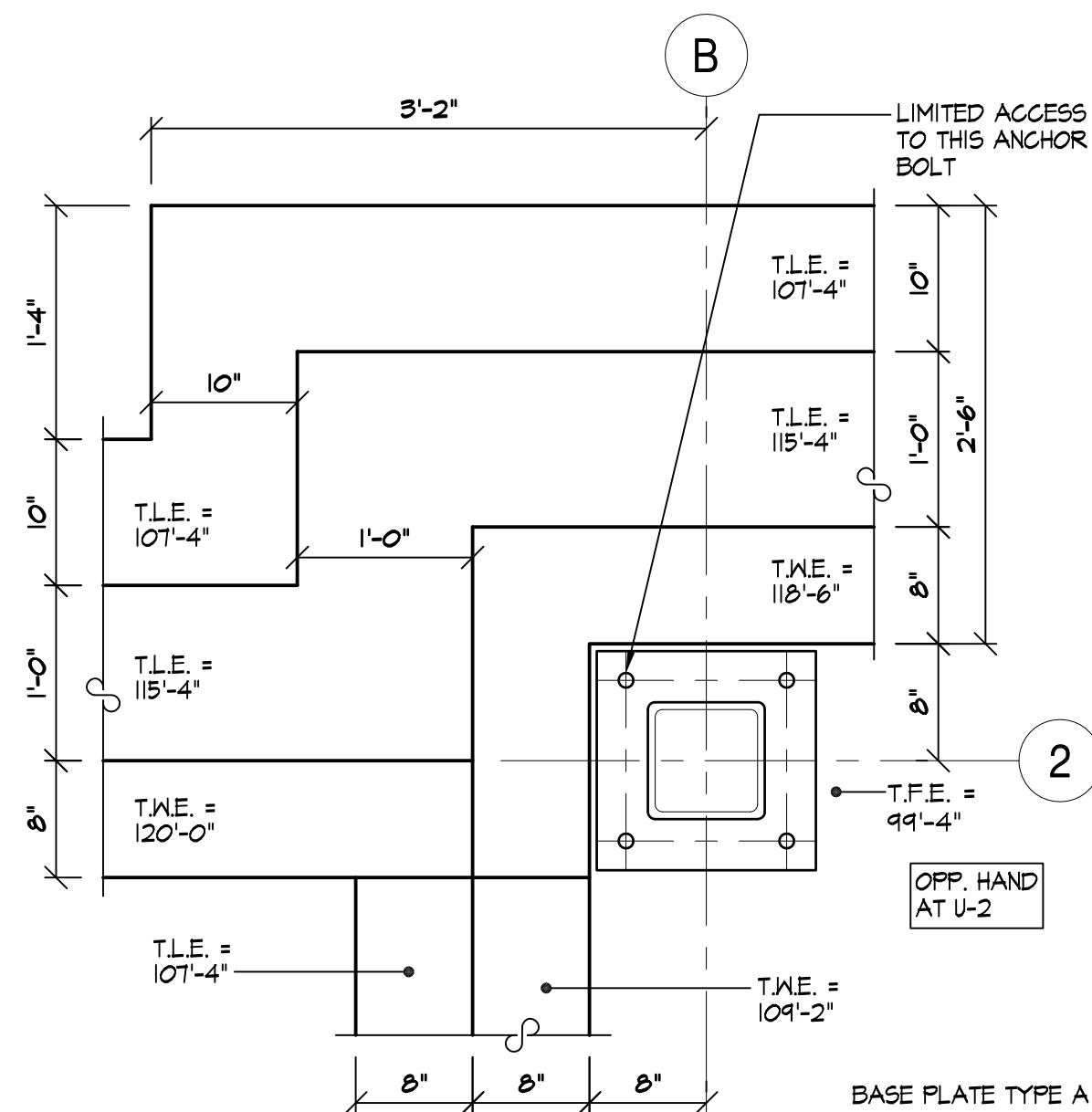
16 PLAN DETAIL - at COL B-2 S-106 SCALE: 1" = 1'-0"
