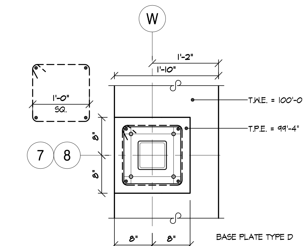
15 PLAN DETAIL - at COL. W-7 & W-8 S-106 SCALE: 1" = 1'-0"
