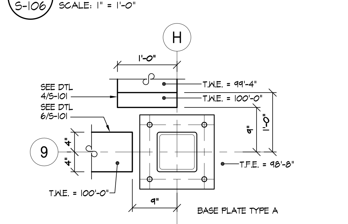
7 PLAN DETAIL - at COL. H-9 S-106 SCALE: 1" = 1'-0"
