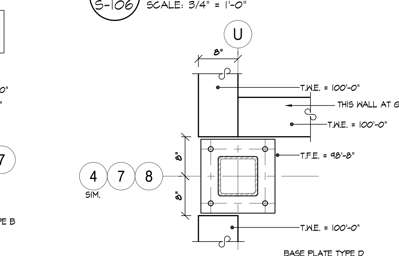
14 PLAN DETAIL - at COL. U-7 & U-8 S-106 SCALE: 1" = 1'-0"
