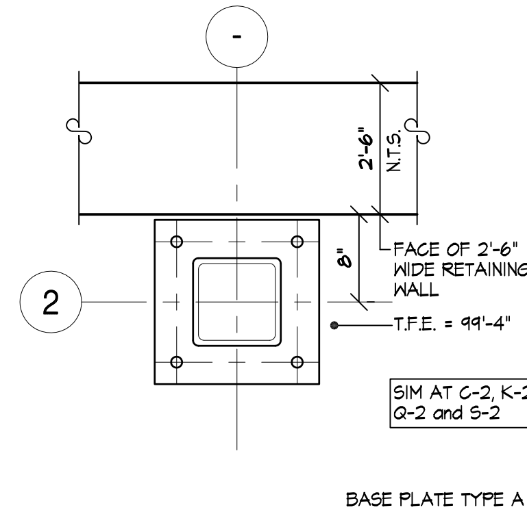
17 PLAN DETAIL - at COL H-2 S-106
