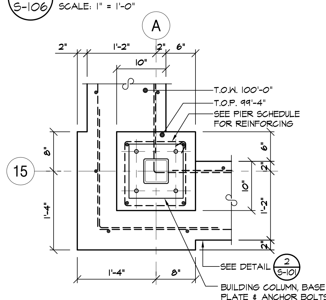
1 PLAN DETAIL - at COL. A-15 S-106 SCALE: 1" = 1'-0"
