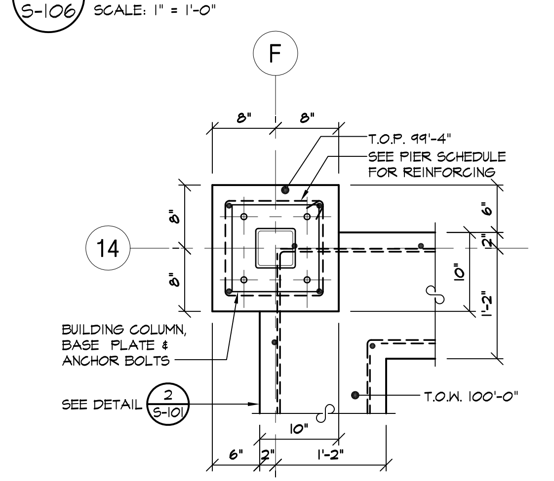
2 PLAN DETAIL - at COL. F-14 S-106 SCALE: 1" = 1'-0"
