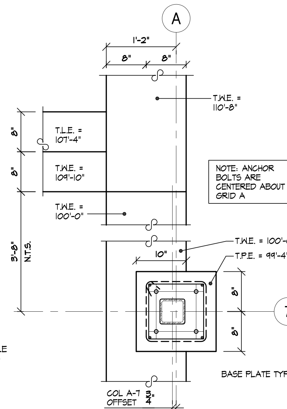
13 PLAN DETAIL - at COL. A-7 S-106 SCALE: 1" = 1'-0"
