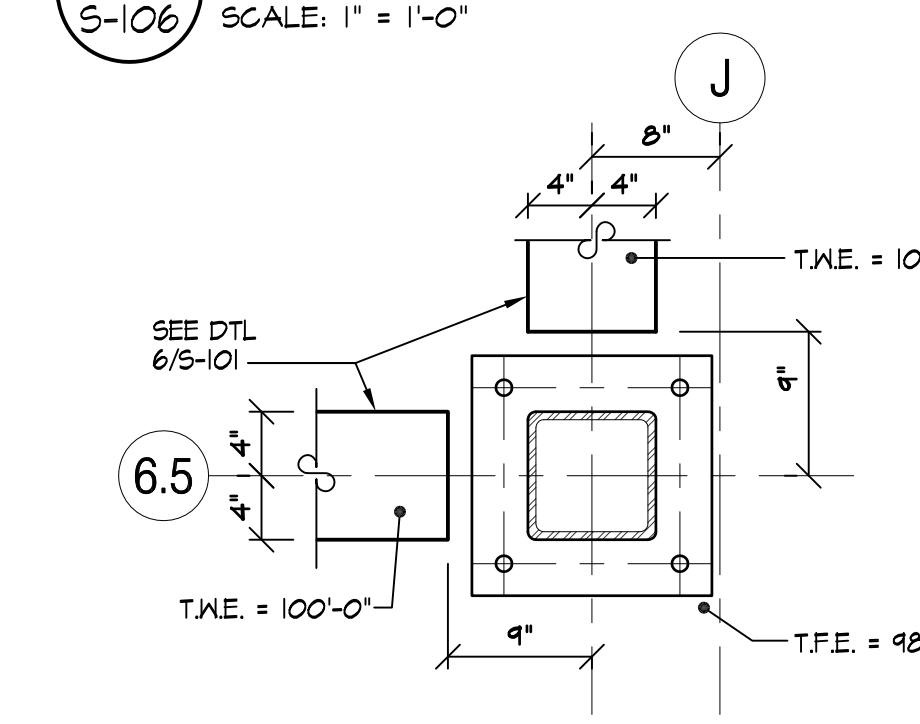
8 PLAN DETAIL - at COL. J-6.5 S-106 SCALE: 1" = 1'-0"
