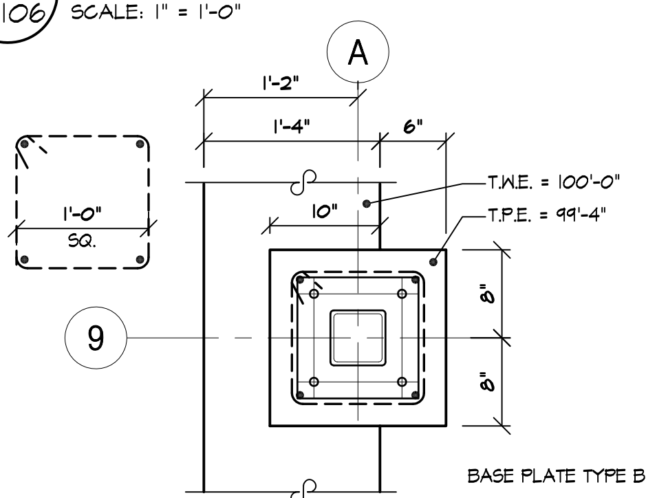
6 PLAN DETAIL - at COL. A-9 S-106 SCALE: 1" = 1'-0"
