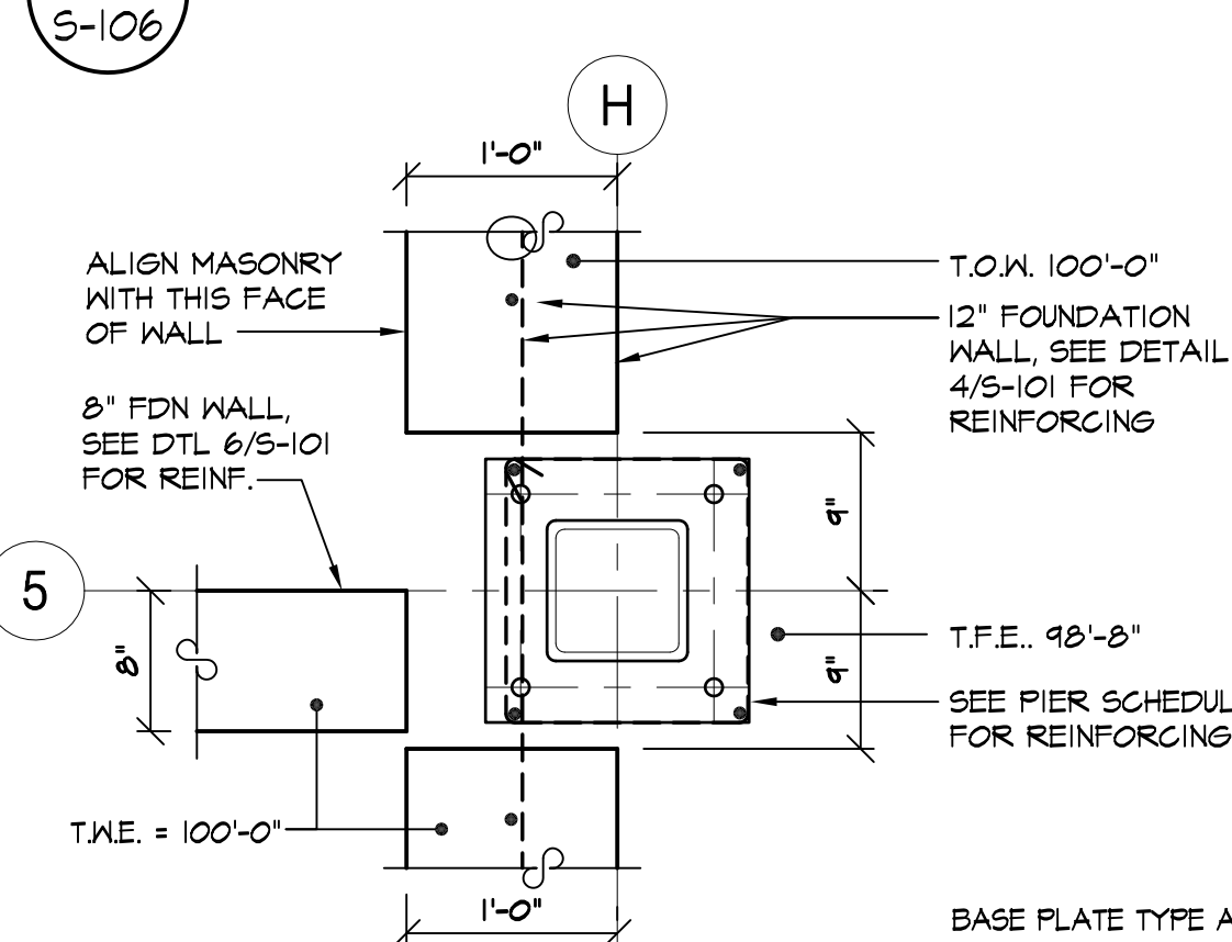
12 PLAN DETAIL - at COL. H-5 S-106 SCALE: 1" = 1'-0"
