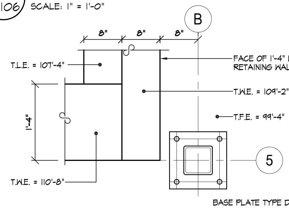
16 PLAN DETAIL - at COL B-2 S-106 SCALE: 1" = 1'-0"
