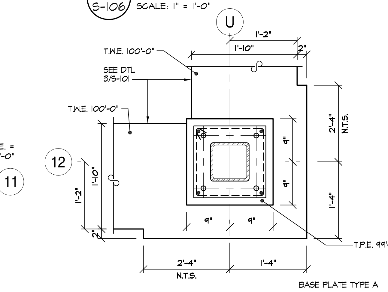
4 PLAN DETAIL - at COL. U-12 S-106 SCALE: 1" = 1'-0"
