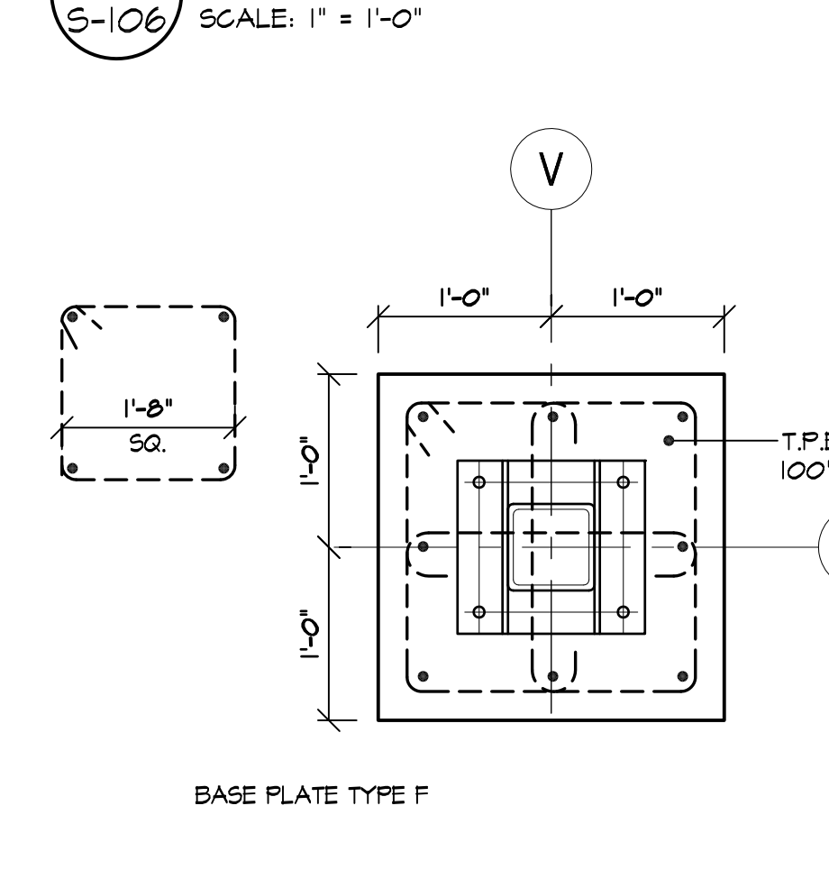
3 PLAN DETAIL - at COL. F.I-16 & V-11 S-106 SCALE: 1" = 1'-0"
