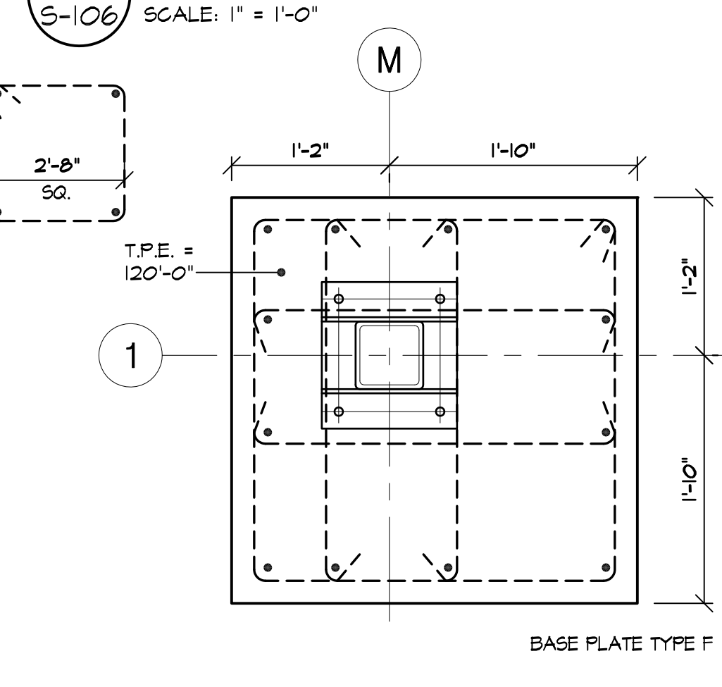
5 PLAN DETAIL - at COL. M-1 & P-1 S-106 SCALE: 1" = 1'-0"
