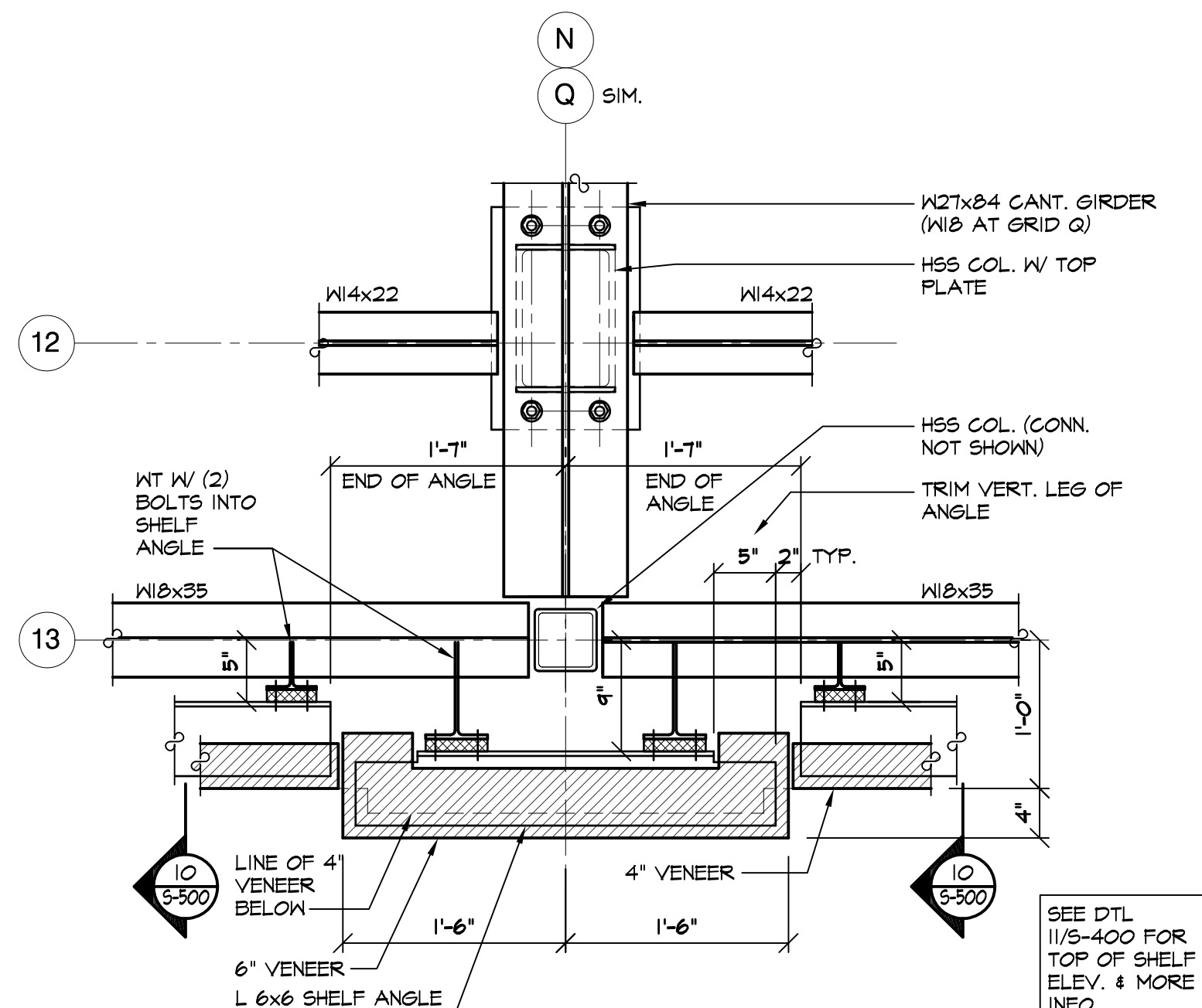
12 PLAN DETAIL - SHELF ANGLES S-400 SCALE: 1" = 1'-0"
