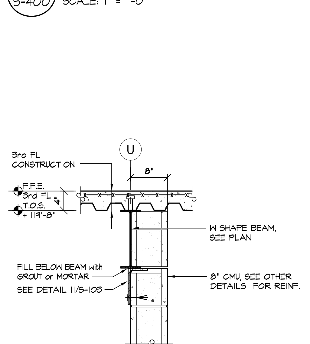
1 SECTION - 3rd FL FRAMING S-400 SCALE: 1" = 1'-0"
