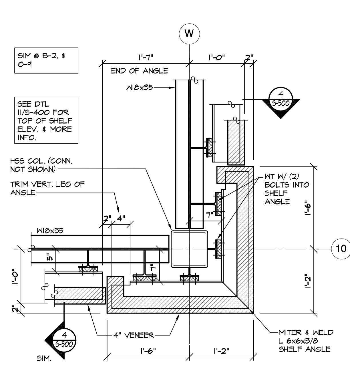
14 PLAN DETAIL - SHELF ANGLES S-400 SCALE: 1" = 1'-0"
