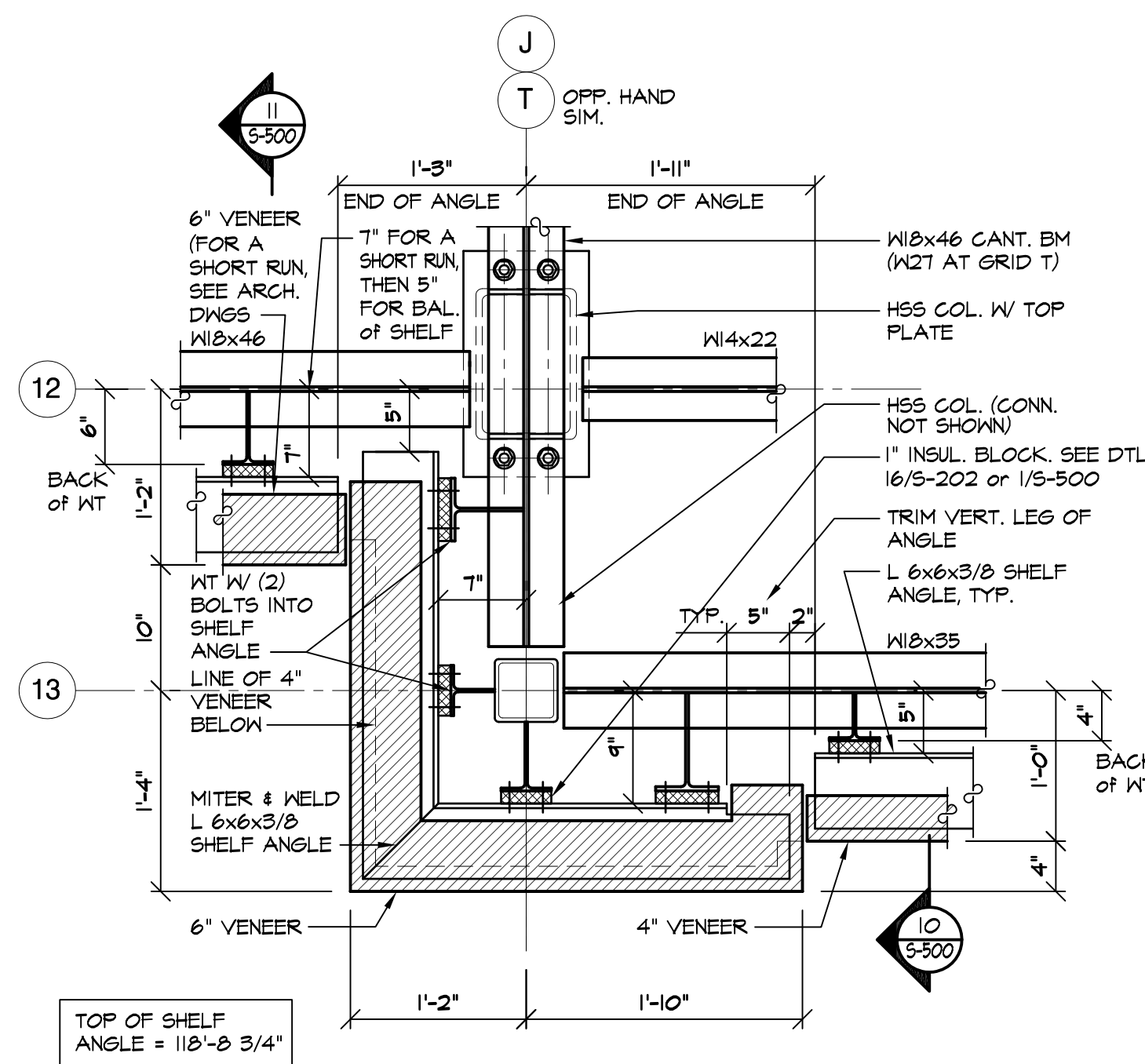
II PLAN DETAIL - SHELF ANGLES S-400 SCALE: 1" = 1'-0"
