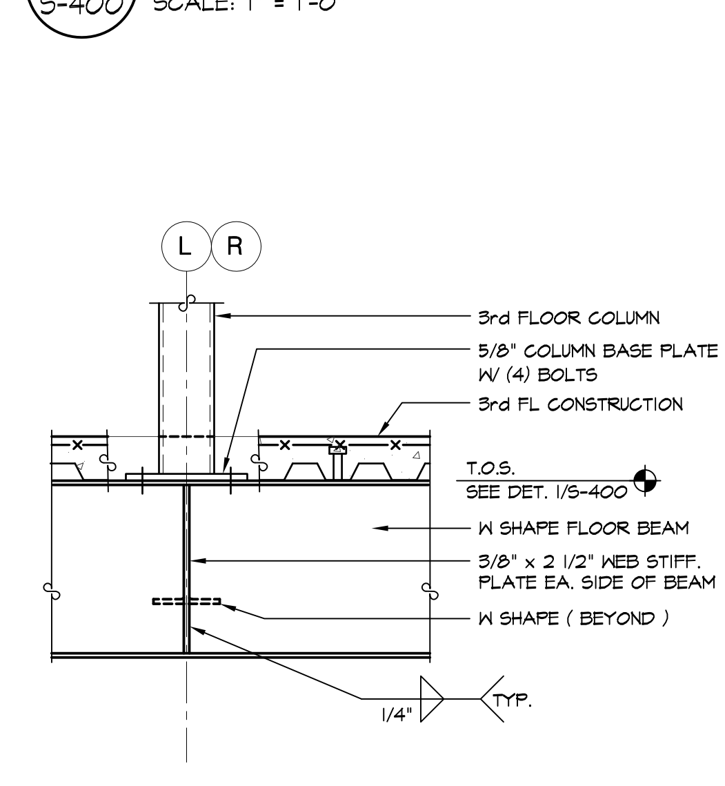
3 SECTION - COLUMN TRANSFER S-400 SCALE: 1" = 1'-0"
