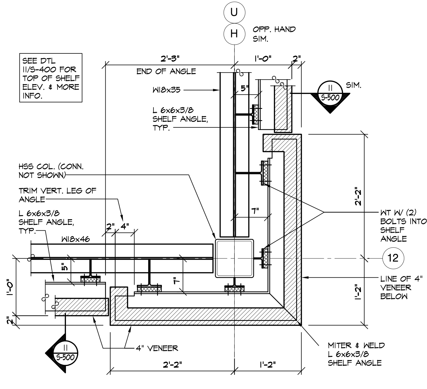
13 PLAN DETAIL - SHELF ANGLES S-400 SCALE: 1" = 1'-0"
