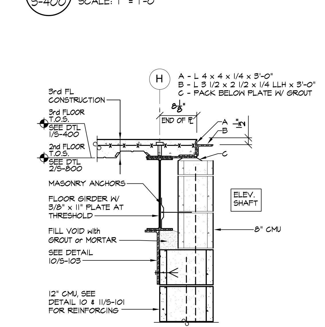
5 SECTION - FLOOR FRAMING at ELEVATOR DOOR S-400 SCALE: 1" = 1'-0"
