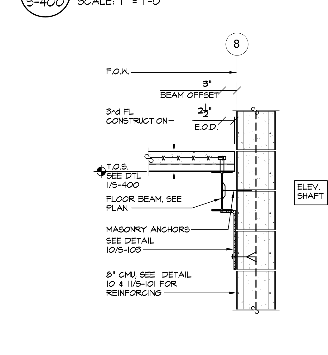
4 SECTION - 3rd FL FRAMING at ELEVATOR S-400 SCALE: 1" = 1'-0"
