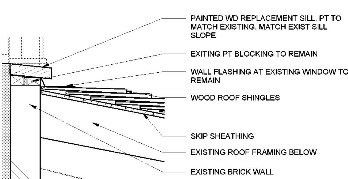
11 MANOR HALL EAST PORCH ROOF WINDOW TERMINATION 1 1/2" = 1'-0"
