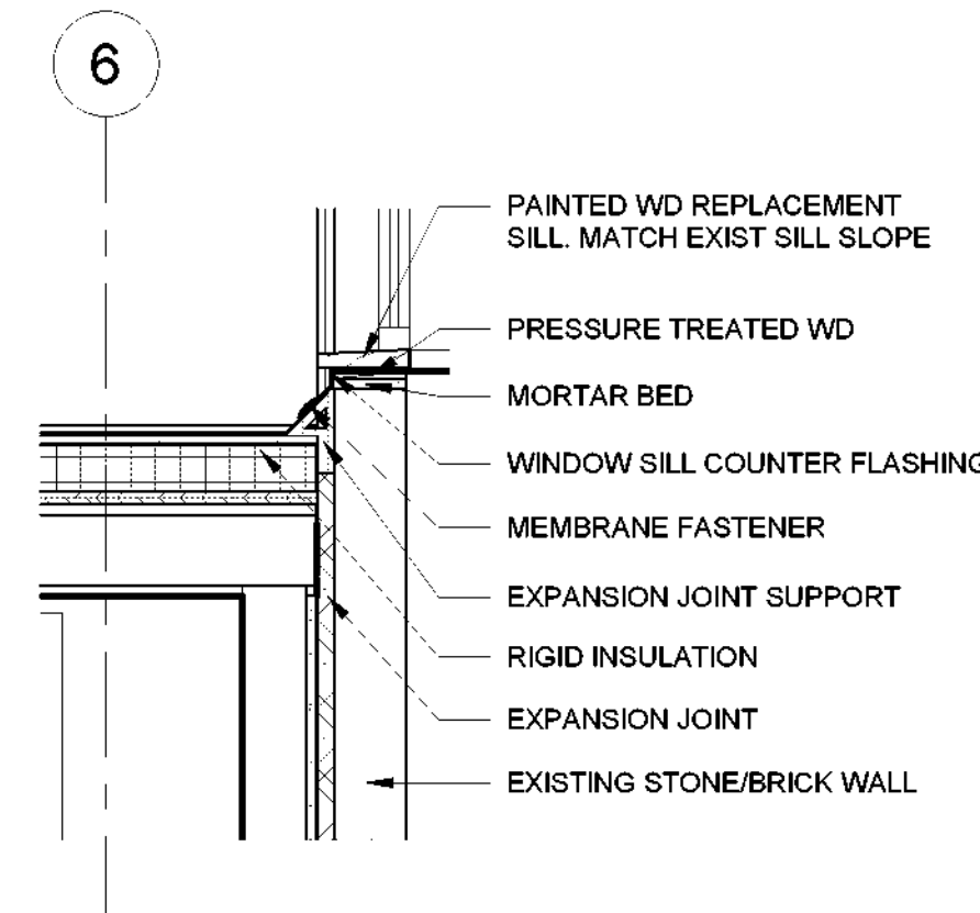
6 R4 ROOF TERMINATION AT MANOR HALL BELOW WINDOWS 1" = 1'-0"
