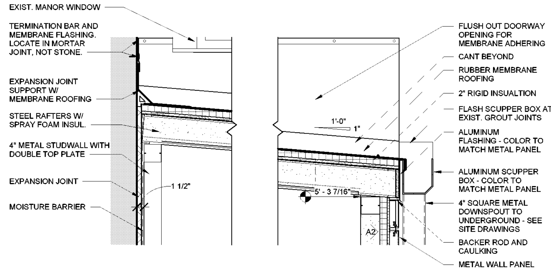
2 JANITOR ROOF GUTTER TROUGH DETAIL 1" = 1'-0"
