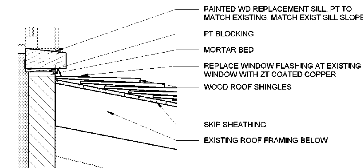
10 MANOR HALL SOUTH PORCH ROOF WINDOW TERMINATION 1 1/2" = 1'-0"
