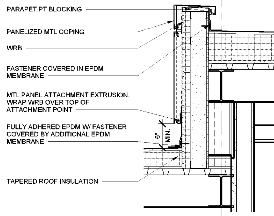
5 ROOF TRANSITION DETAIL AT PARAPET 1" = 1'-0"
