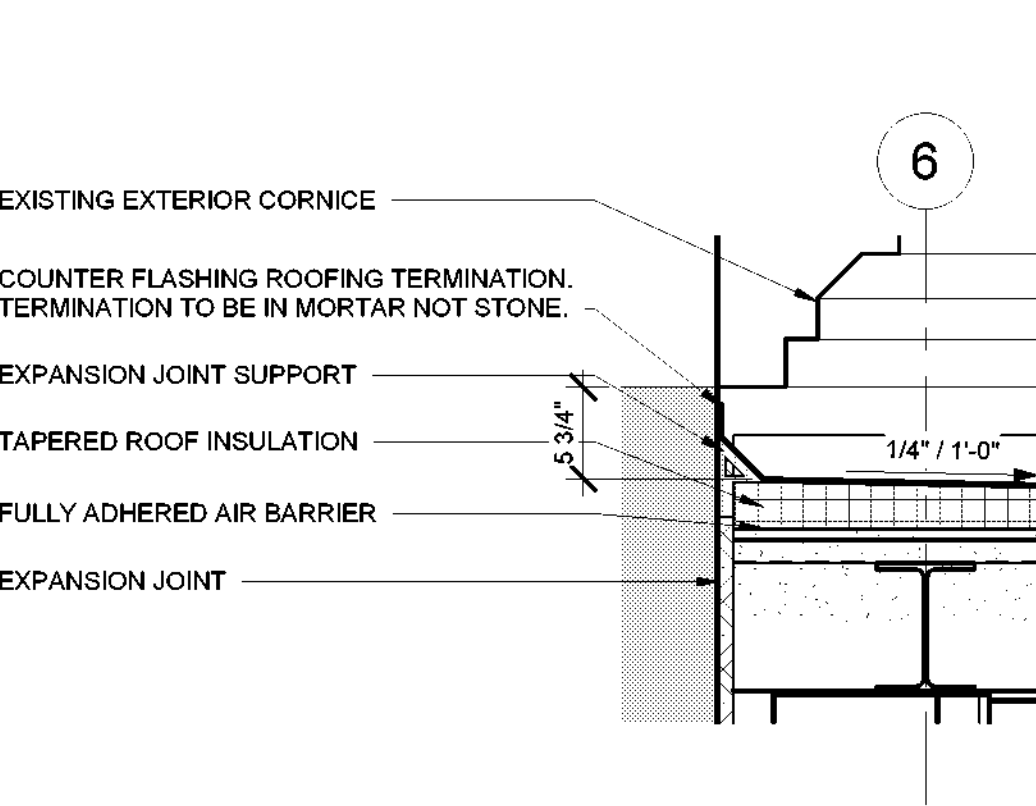
8 SECOND FLOOR ADDITION ROOF CONNECTION 1" = 1'-0"
