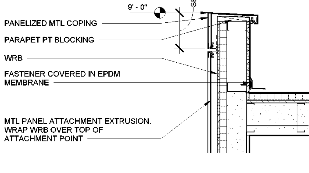
1 JANITOR CLOSET ROOF RAKE EDGE 1" = 1'-0"
