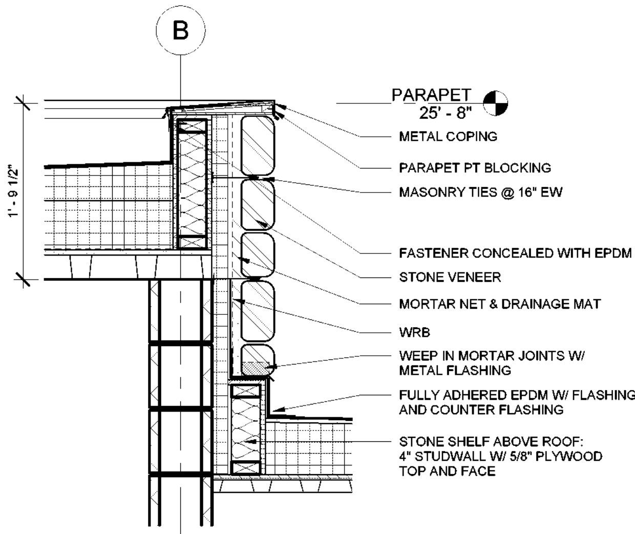
4 STONE PARAPET ROOF DETAIL 1" = 1'-0"
