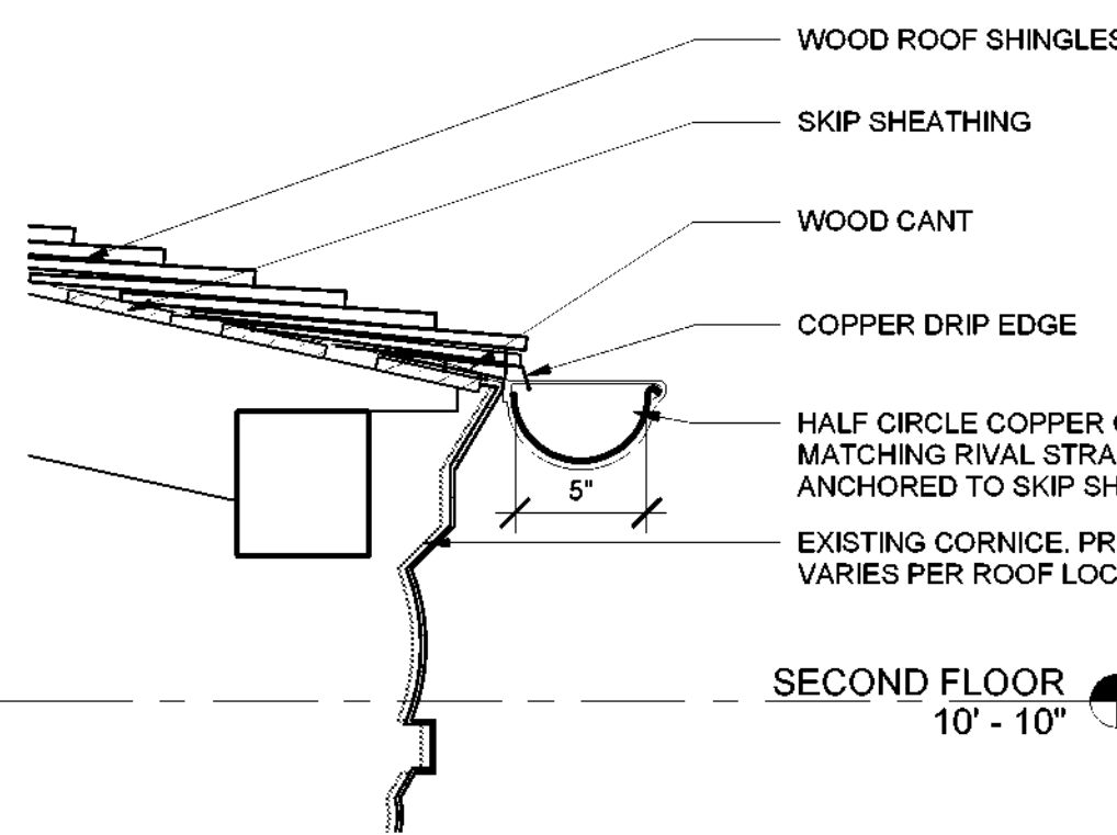
9 MANOR HALL ROOFS GUTTER DETAIL 1 1/2" = 1'-0"
