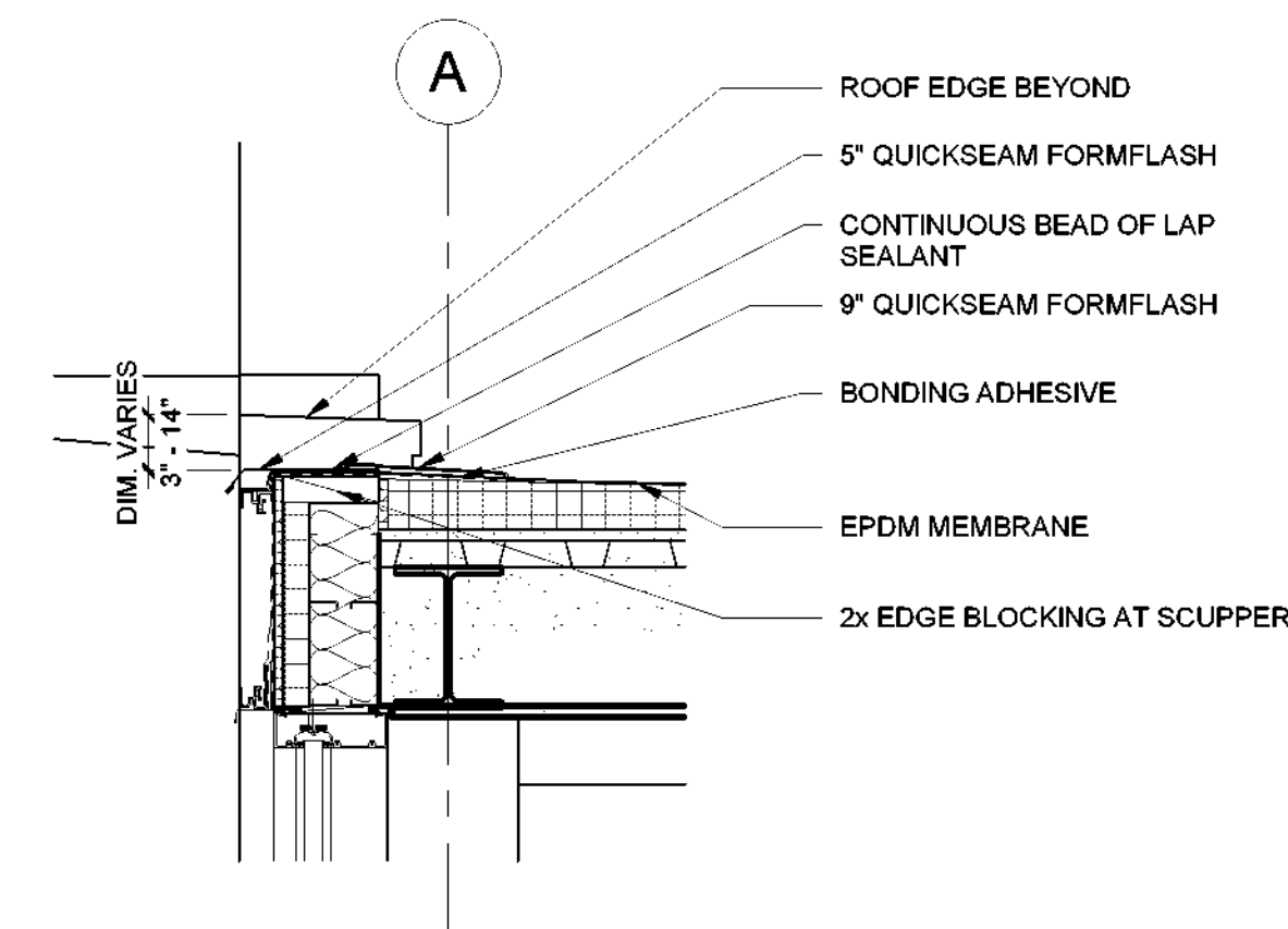
7 SCUPPER DETAIL - (TYP) 1" = 1'-0"
