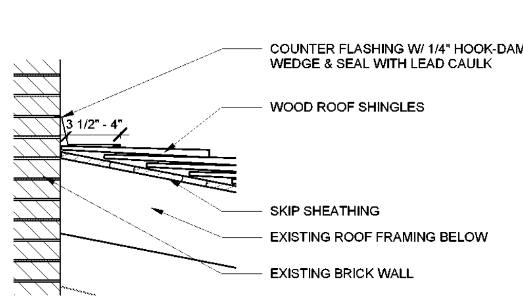
12 MANOR HALL PORCH ROOF WALL TERMINATION 1 1/2" = 1'-0"
