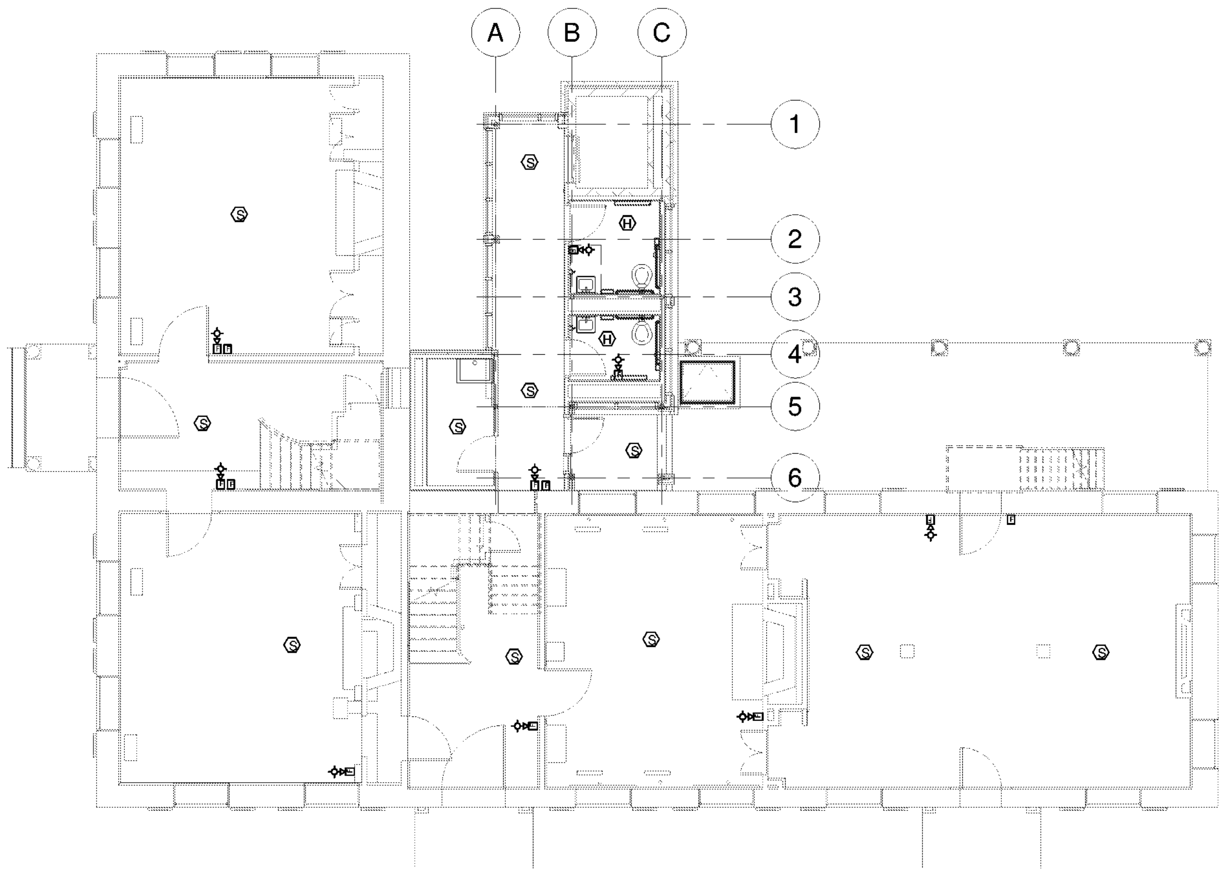
FIRST FLOOR FIRE ALARM PLAN SCALE: 1/8" = 1'-0"
