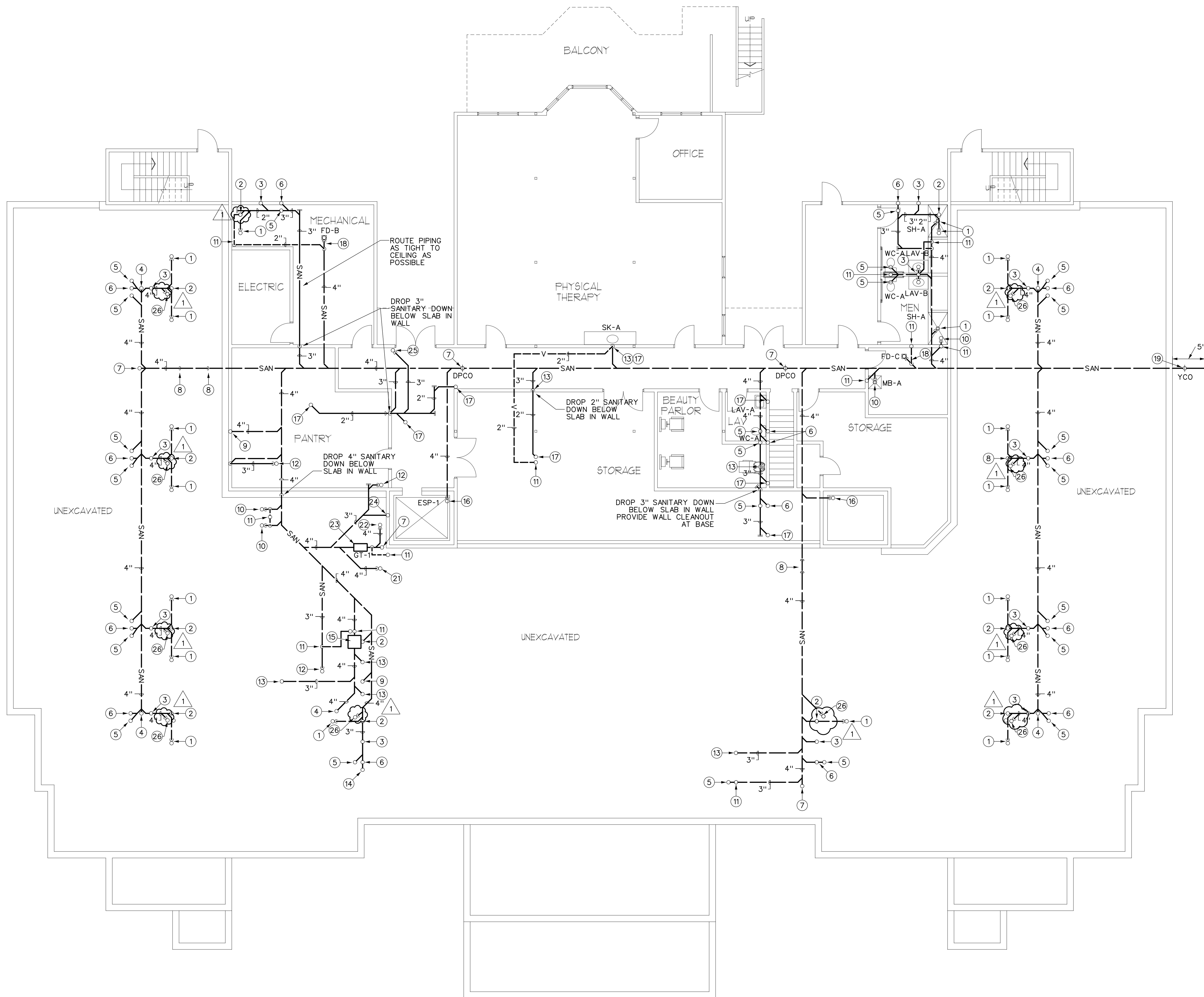
BASEMENT FLOOR PLAN SCALE: 1/8"=1'-0"
