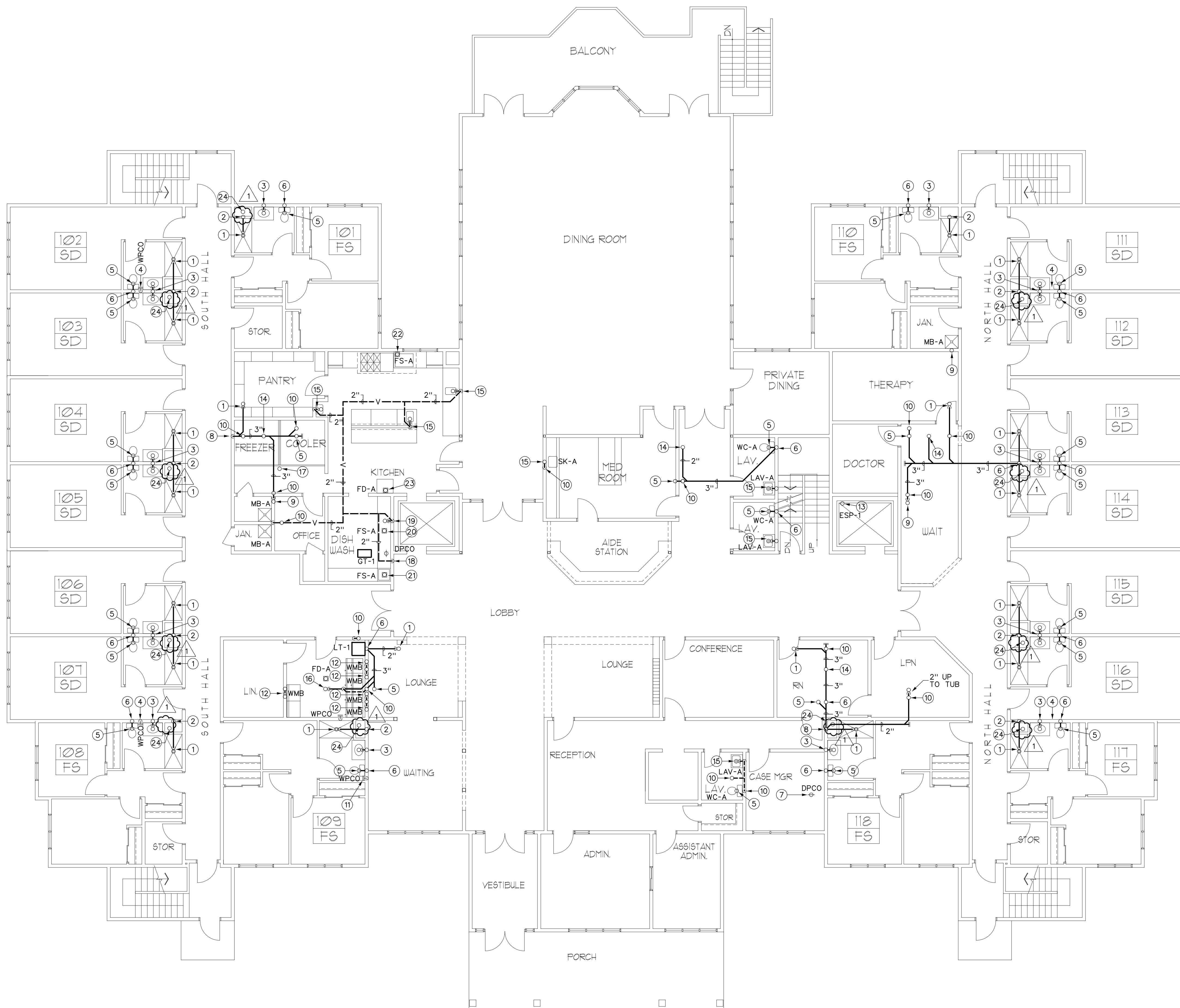
1 FIRST FLOOR PLAN SCALE: 1/8"=1'-0" NORTH
