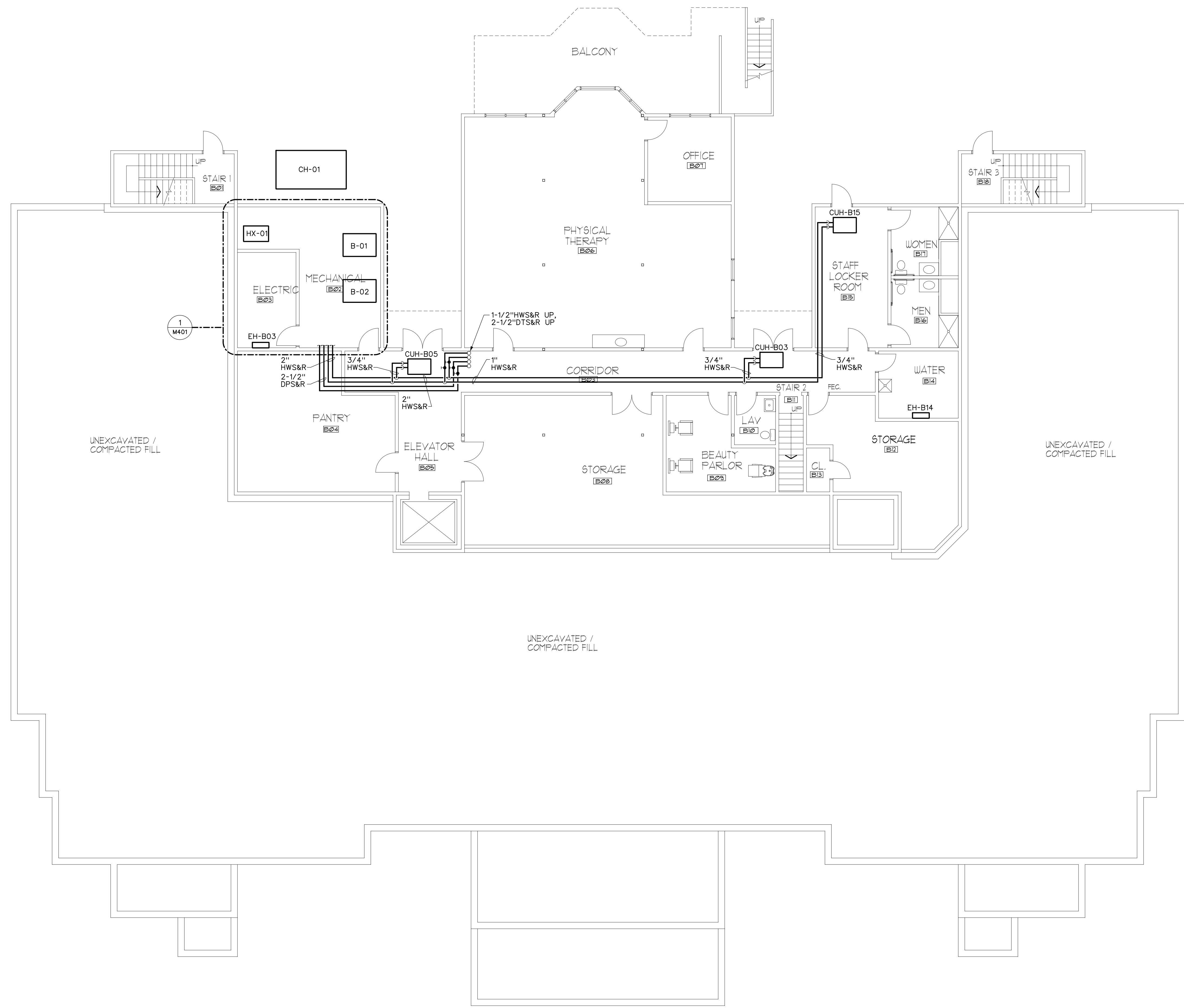
1 BASEMENT MECHANICAL PIPING PLAN M201 SCALE: 1/8"=1'-0"
