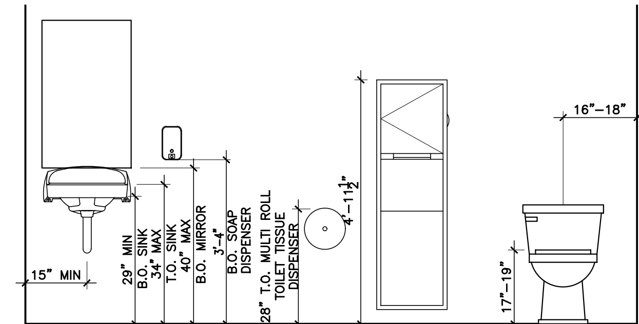
5 ADA MOUNTING HEIGHTS 1/4" = 1'-0"
