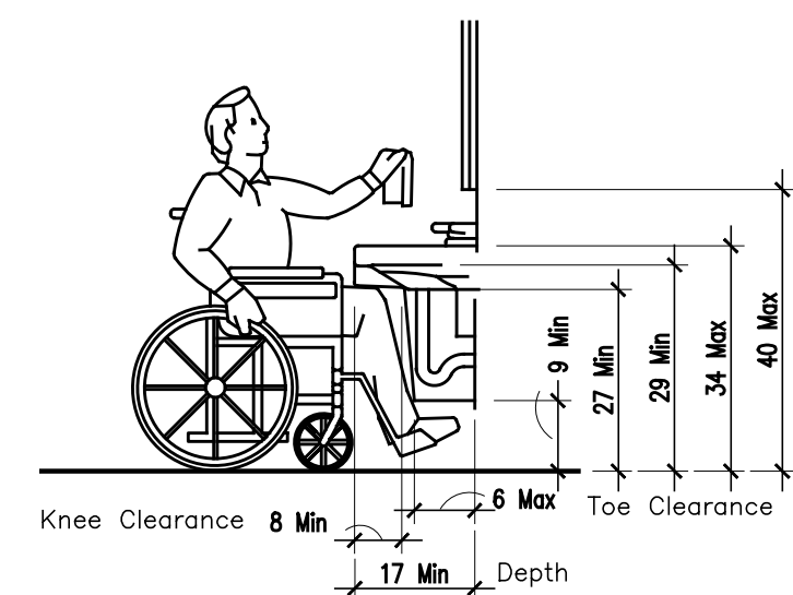
6 ADA CLEARANCES AT LAVS N.T.S.
