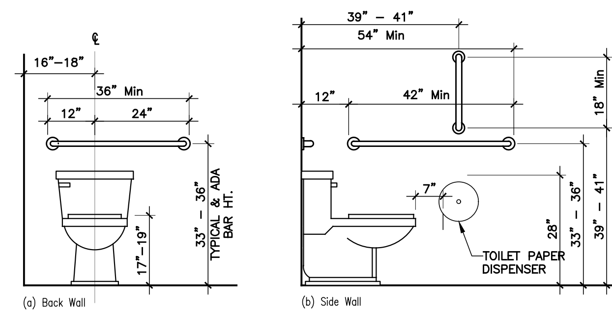
4 TOILET HEIGHT 1/4" = 1'-0"
