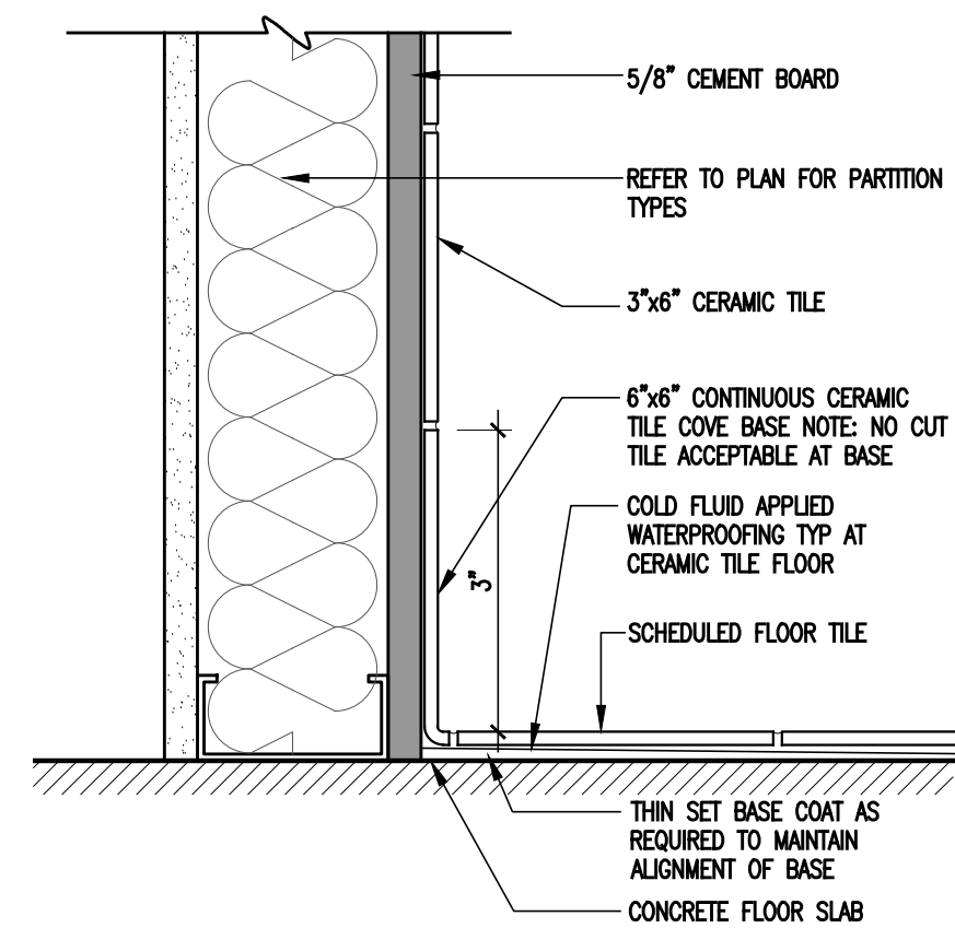
7 TYP. CERAMIC TILE DETAIL 3" = 1'-0"
