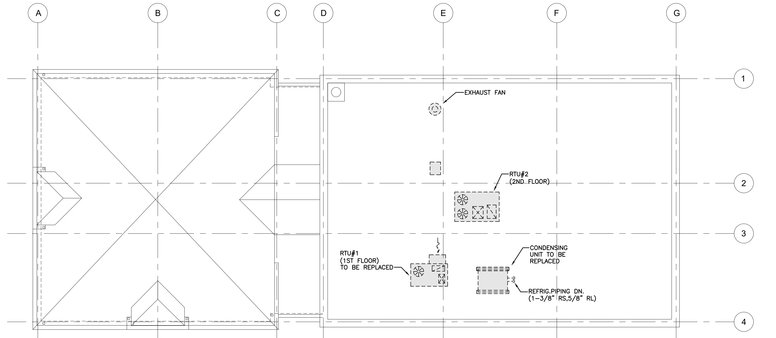
4 ROOF PLAN - EXISTING ME-1 SCALE: 1/8" = 1'-0"
