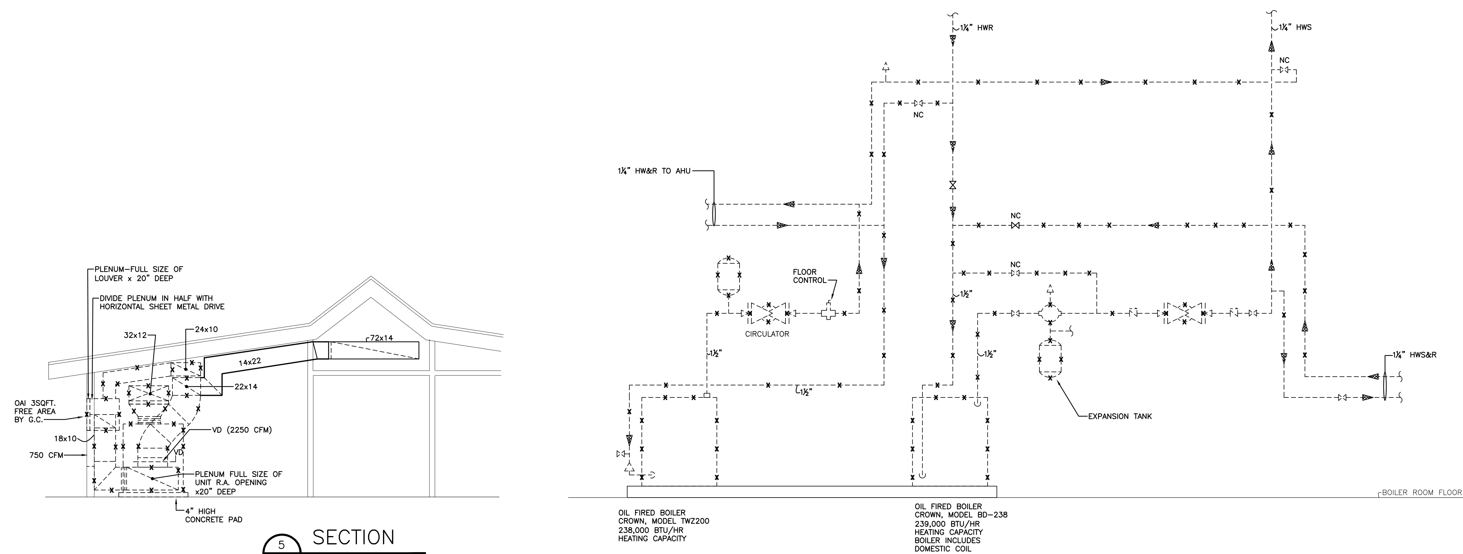
6 BOILER ROOM HOT WATER PIPING SCHEMATIC-REMOVAL ME-1 NOT TO SCALE
