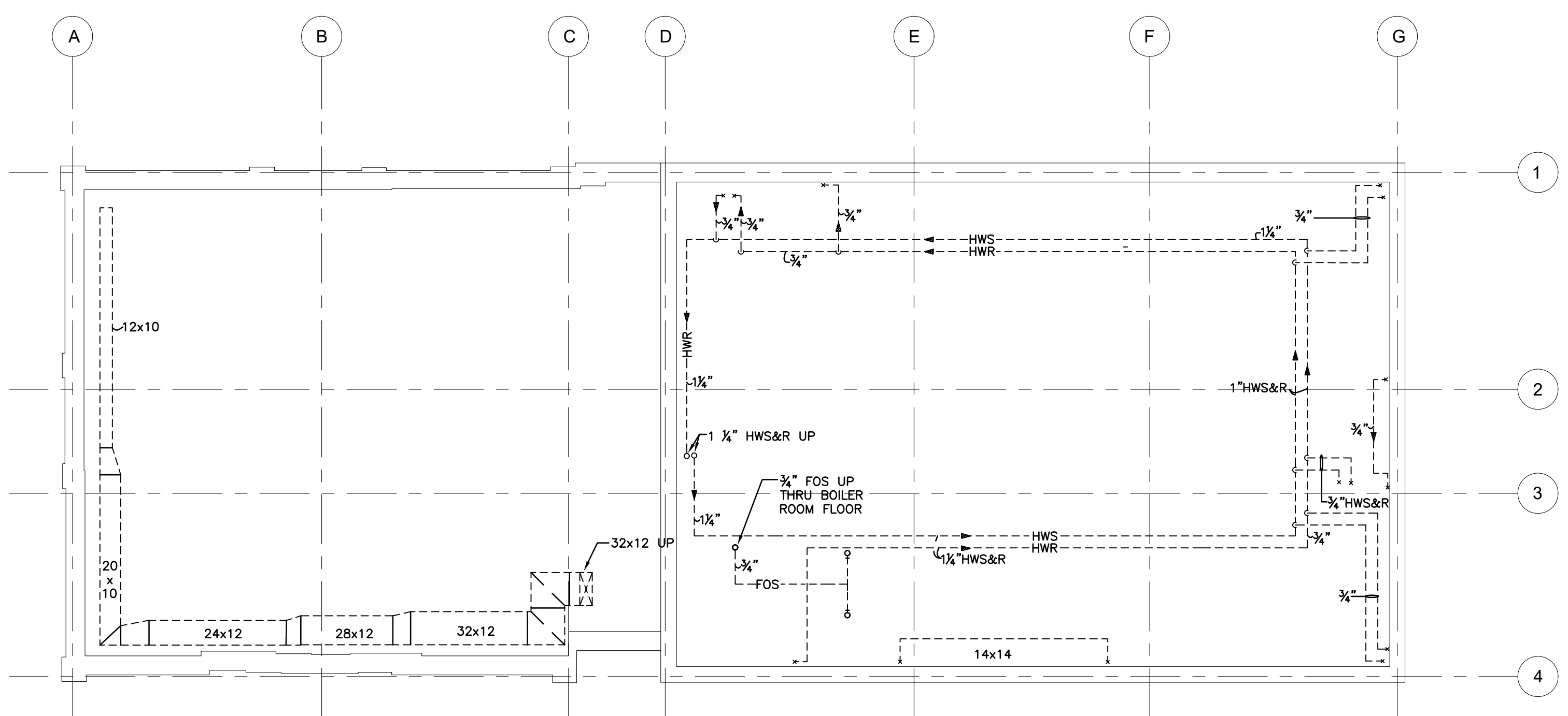
1 CRAWL SPACE PLAN - EXISTING ME-1 SCALE: 1/8" = 1'-0"
