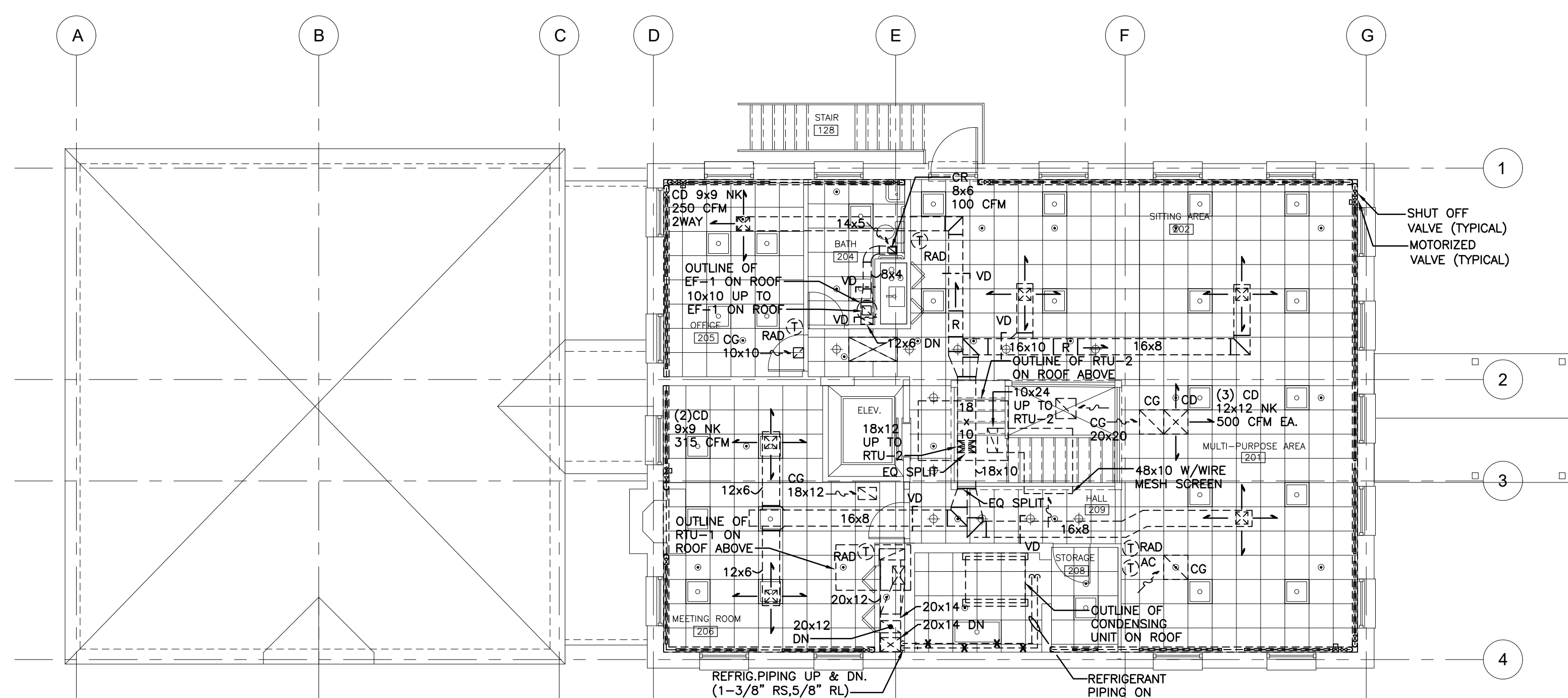
2 SECOND FLOOR PLAN - EXISTING ME-1 SCALE: 1/8" = 1'-0"
