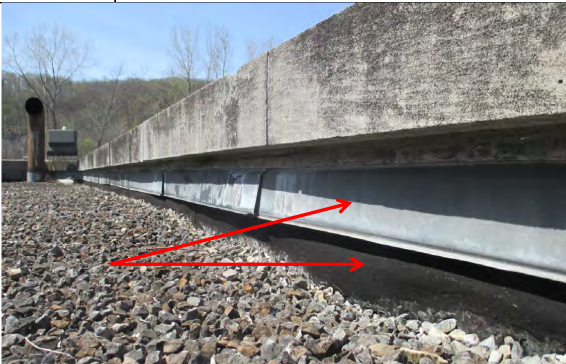
Photo #6 - View of the northeast perimeter on the lower level of the Blower building roof. The upper red arrow shows the lead-containing metal flashing and the lower red arrow shows the asbestos-containing flashing tar.
