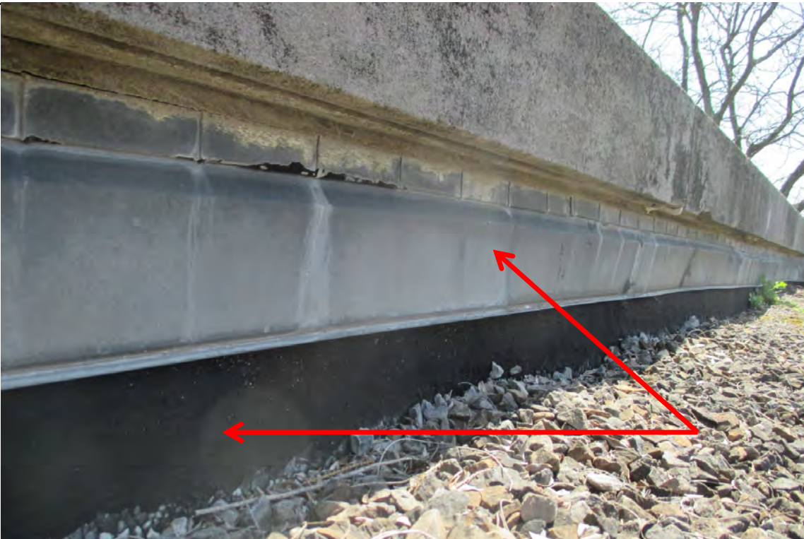
Photo #3 - View of the perimeter of the Administration building roof. The top red arrow shows the lead-containing metal flashing edge. The bottom red arrow shows the area along the perimeter of the roof that has the asbestos-containing roof flashing tar.
