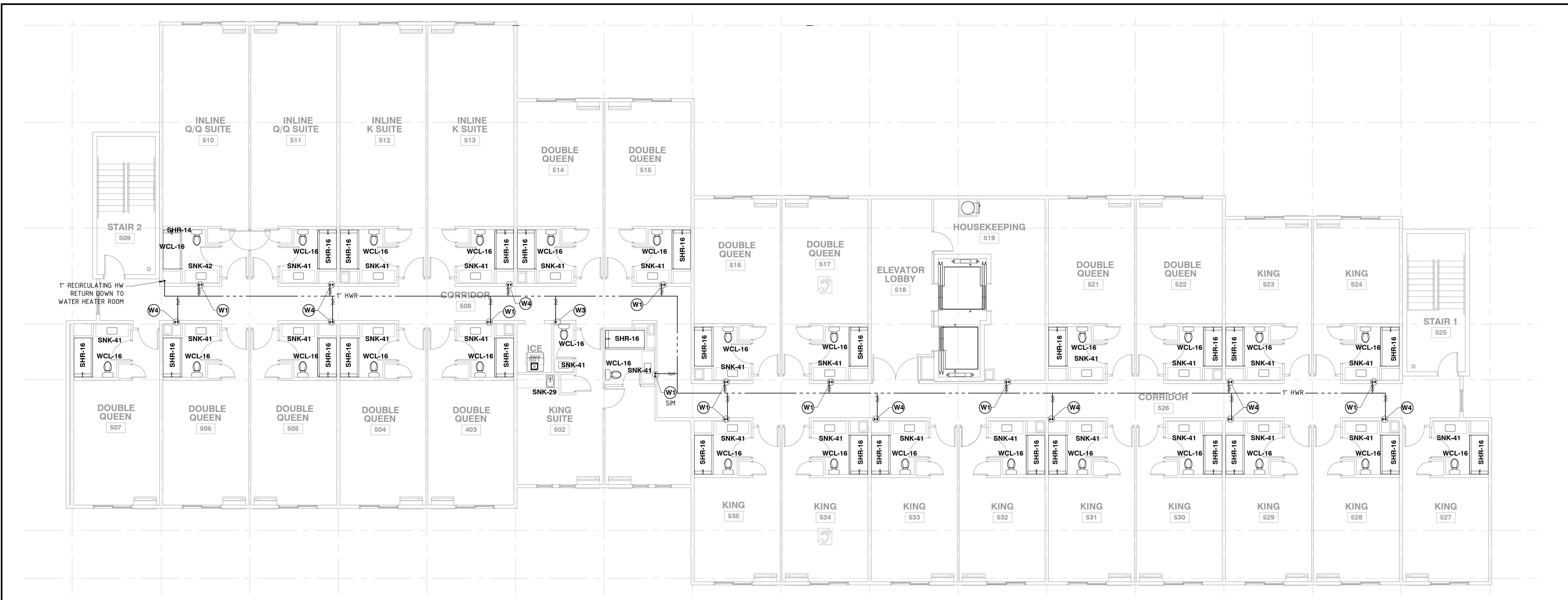
14 FIFTH FLOOR WATER & FUEL GAS PLAN P203 1/8" = 1'-0"
