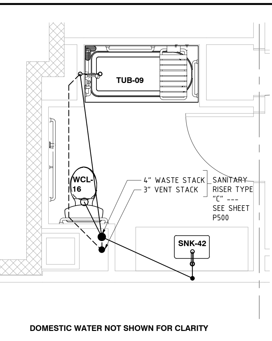
32 ADA DOUBLE QUEEN GUEST BATHROOM P301 3/8" = 1'-0"
