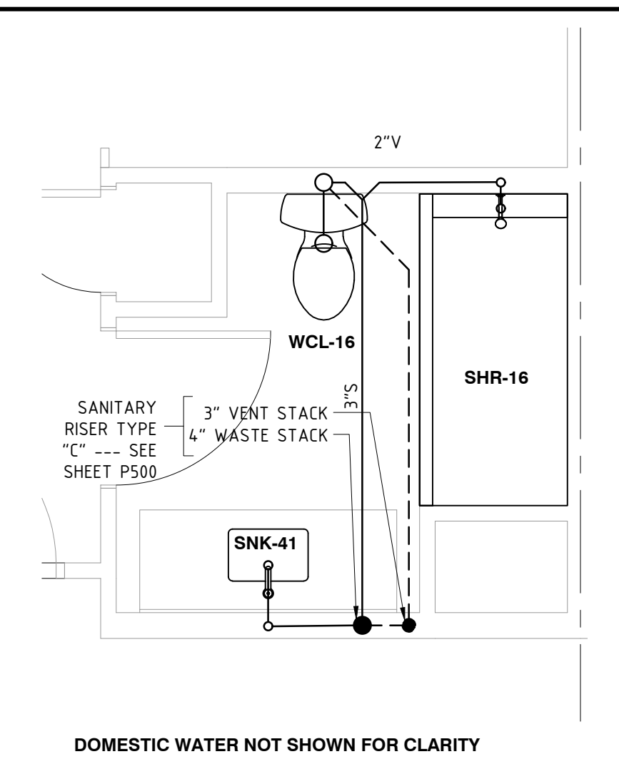
42 TYPICAL GUEST BATHROOM - PLUMBING PLAN P301 3/8" = 1'-0"
