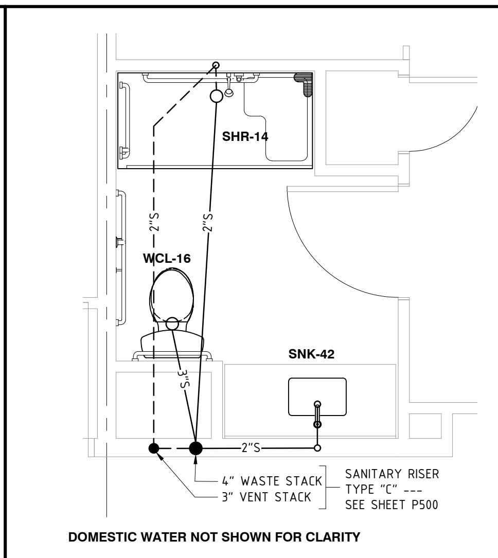
22 TYPICAL ADA GUEST BATHROOM - PLUMBING PLAN P301 3/8" = 1'-0"
