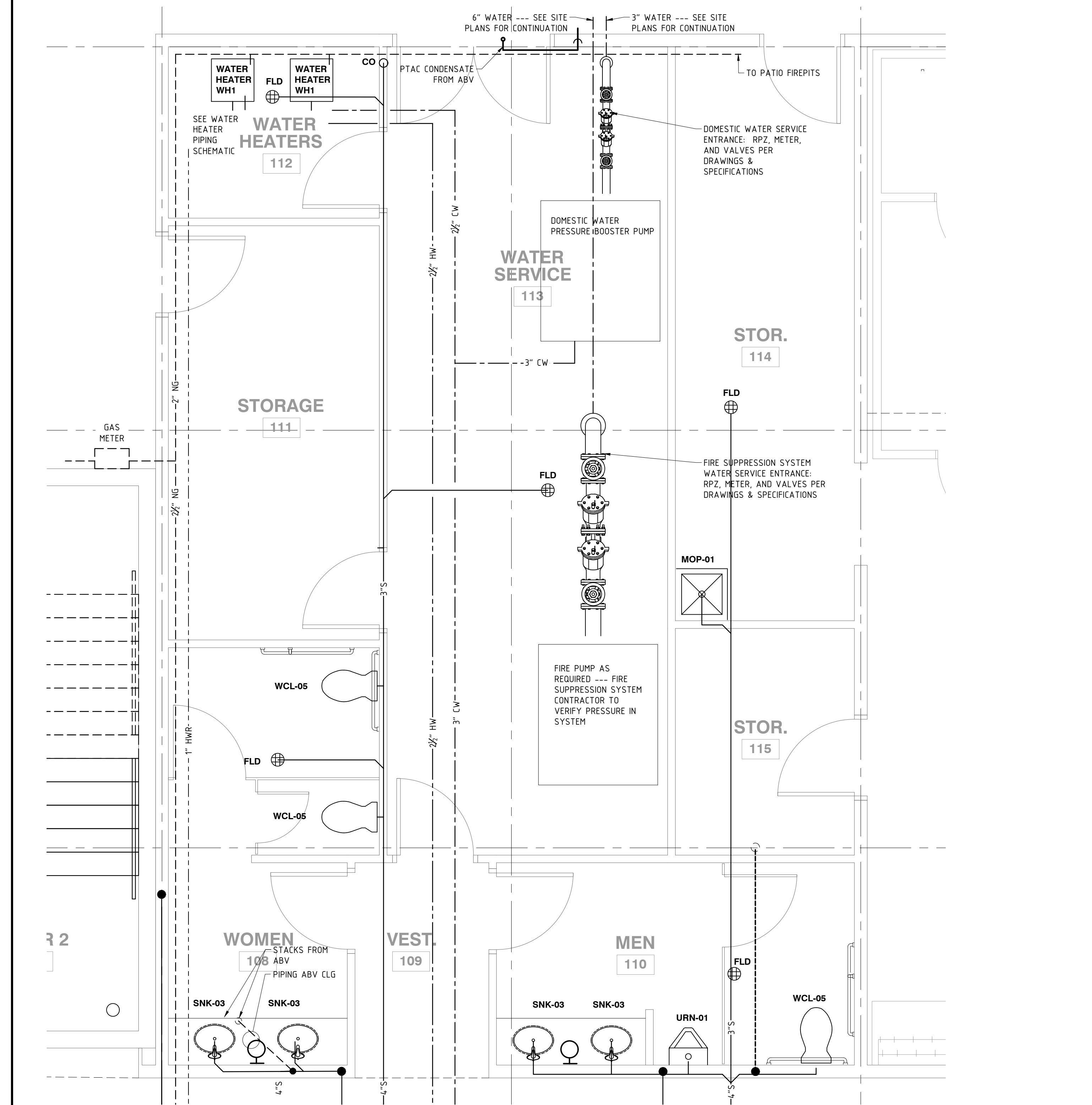
14 UTILITY ROOM & PUBLIC RESTROOMS - PLUMBING PLAN P301 3/8" = 1'-0"
