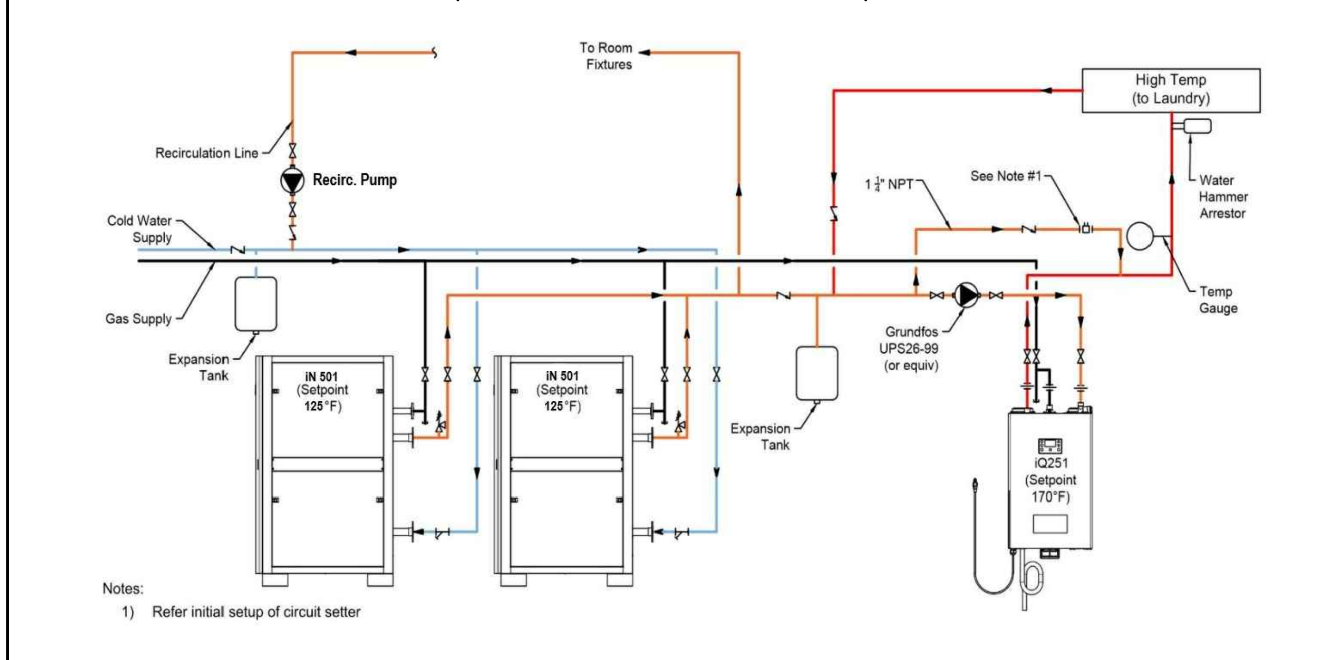
43 WATER HEATER DIAGRAM - SCHEMATIC P301
