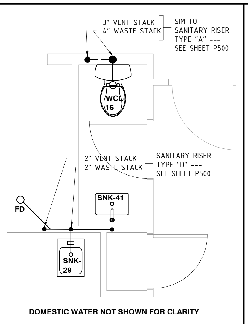
42 KING SUITE BATHROOM - PLUMBING PLAN P301 3/8" = 1'-0"
