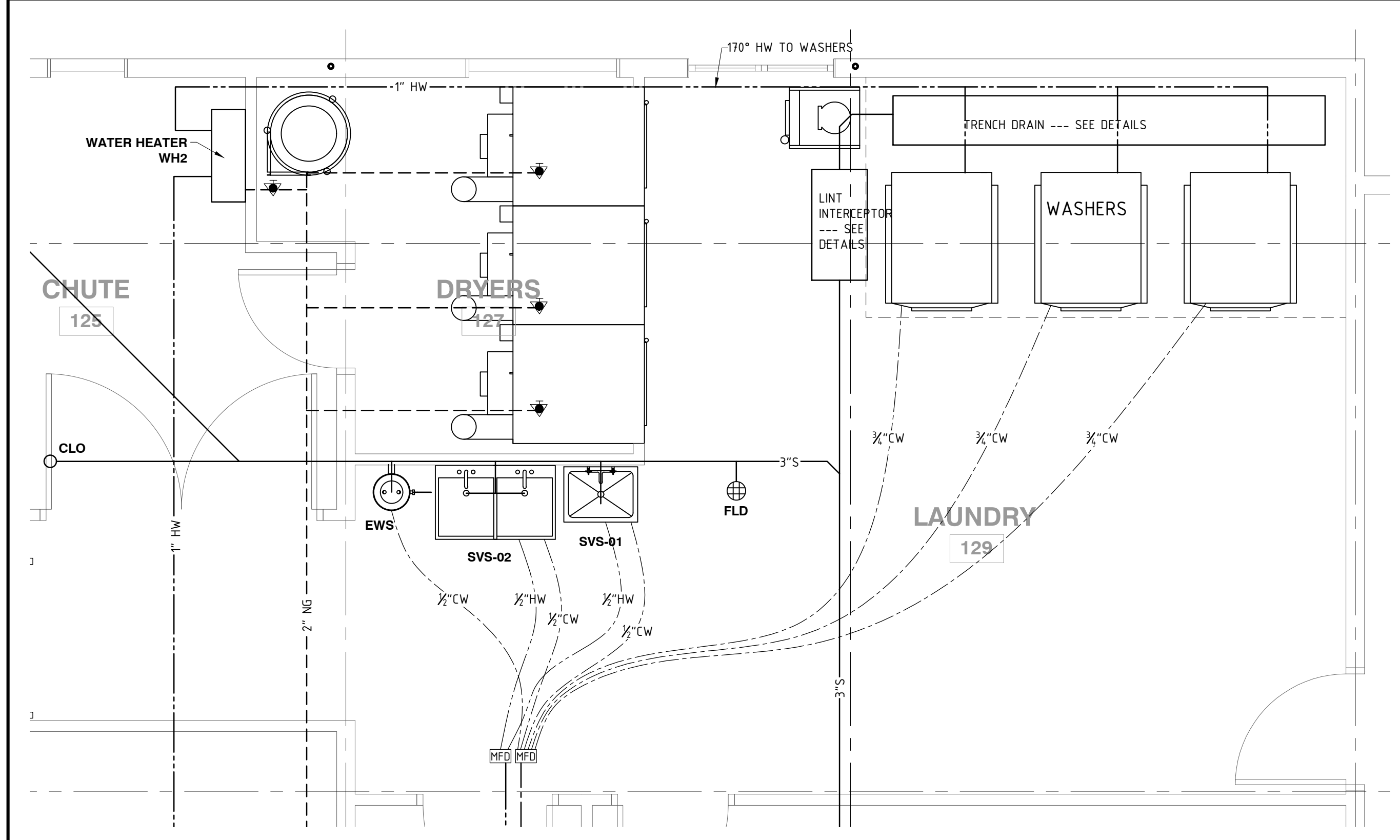
44 LAUNDRY ROOM - PLUMBING PLAN P301 3/8" = 1'-0"
