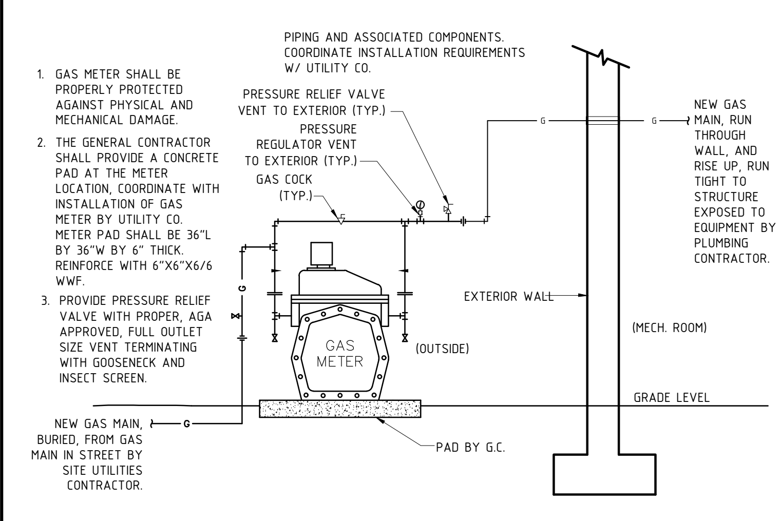
34 FUEL GAS METER INSTALLATION --- VERIFY WITH AHJ
