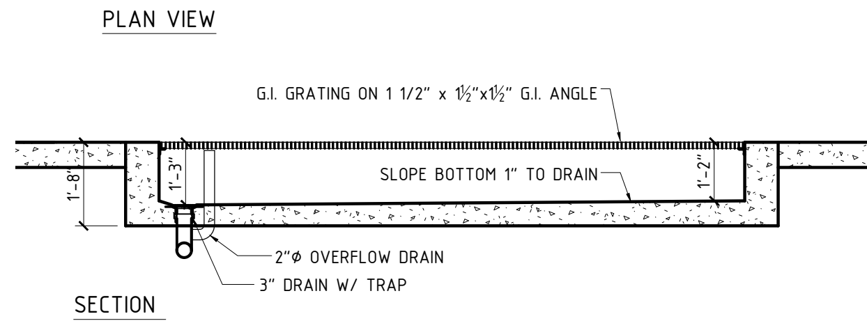
31 LINT INTERCEPTOR DETAIL
