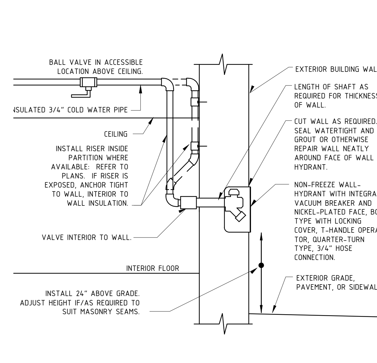
34 EXTERIOR WALL HOSE BIBB
