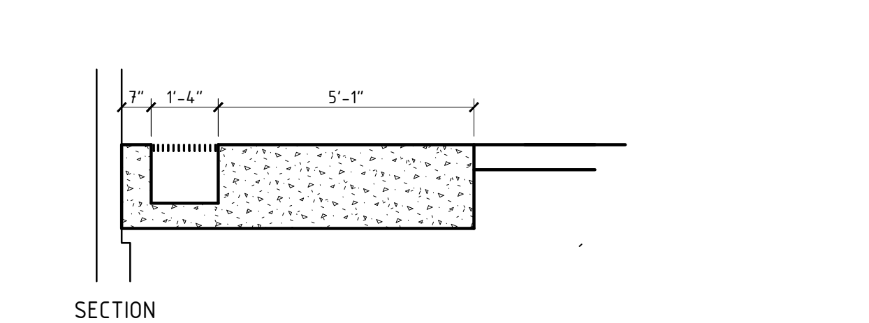
22 LAUNDRY TRENCH DRAIN DETAILS
