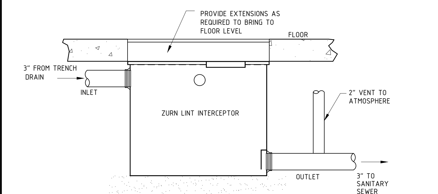
31 LINT INTERCEPTOR DETAIL
