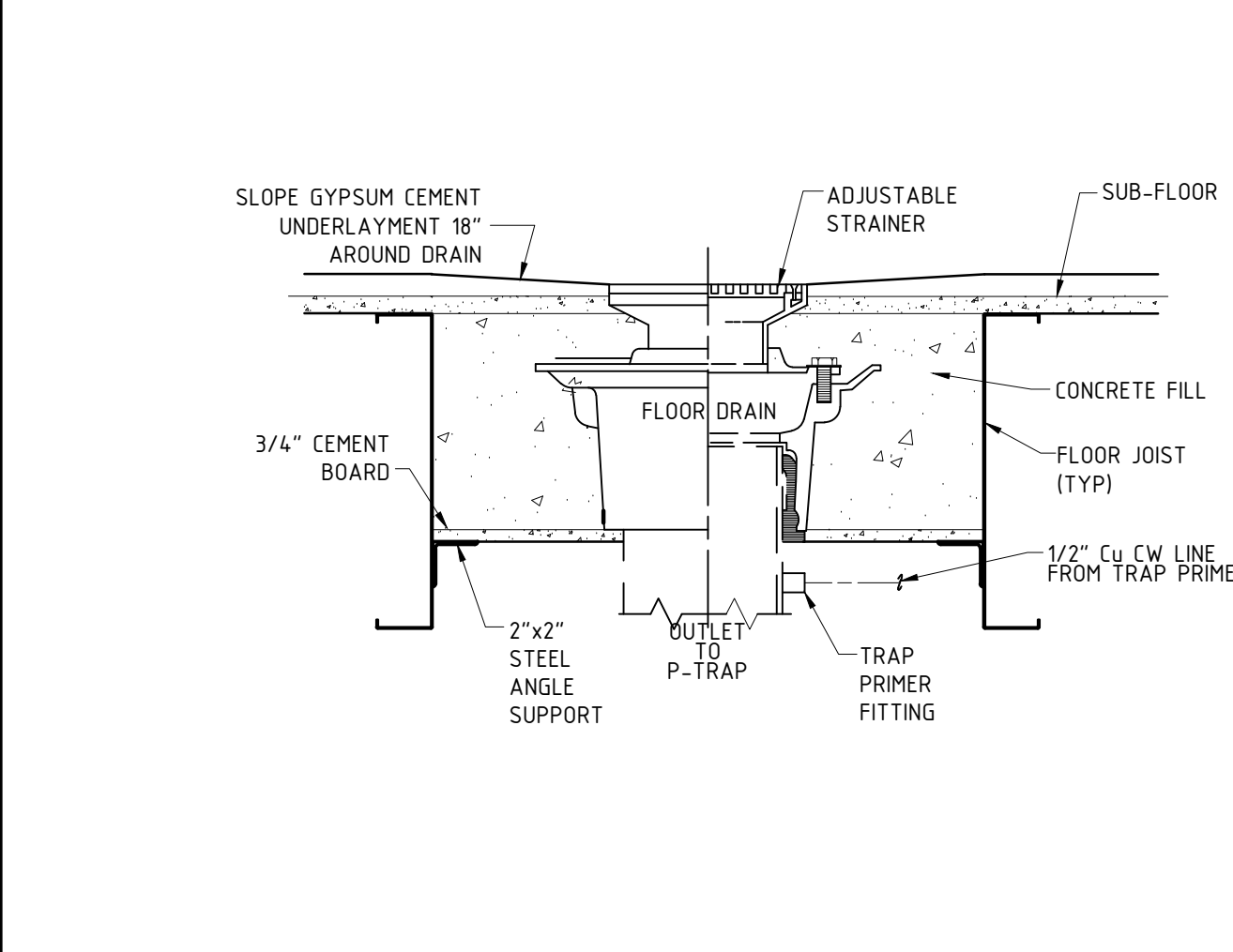
14 FLOOR DRAIN DETAIL
