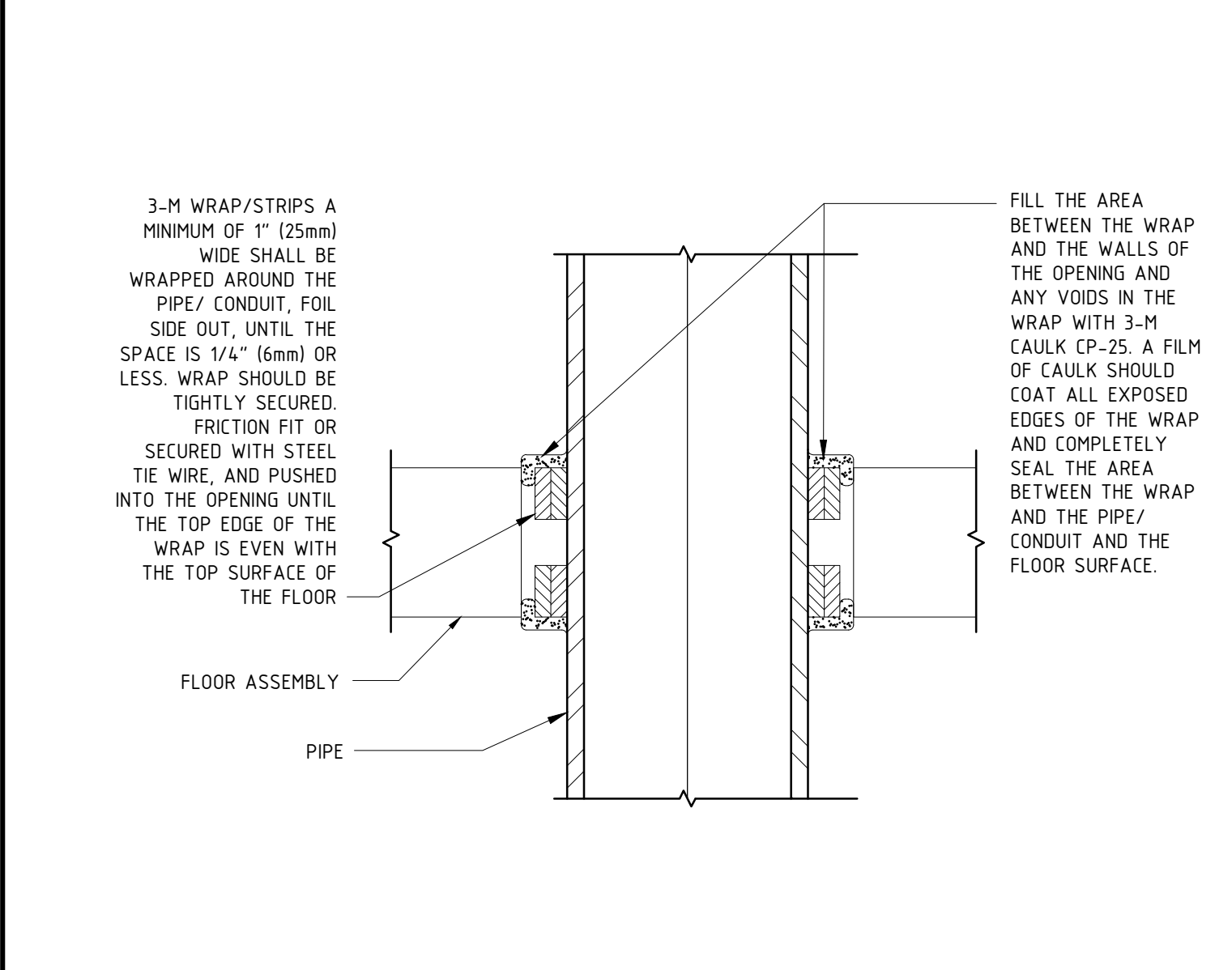
34 RPZ DIAGRAM
