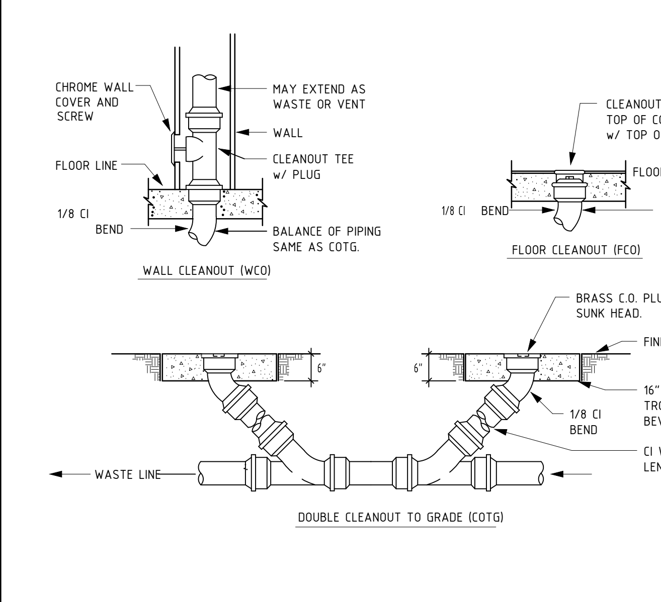
12 CLEANOUT DETAILS
