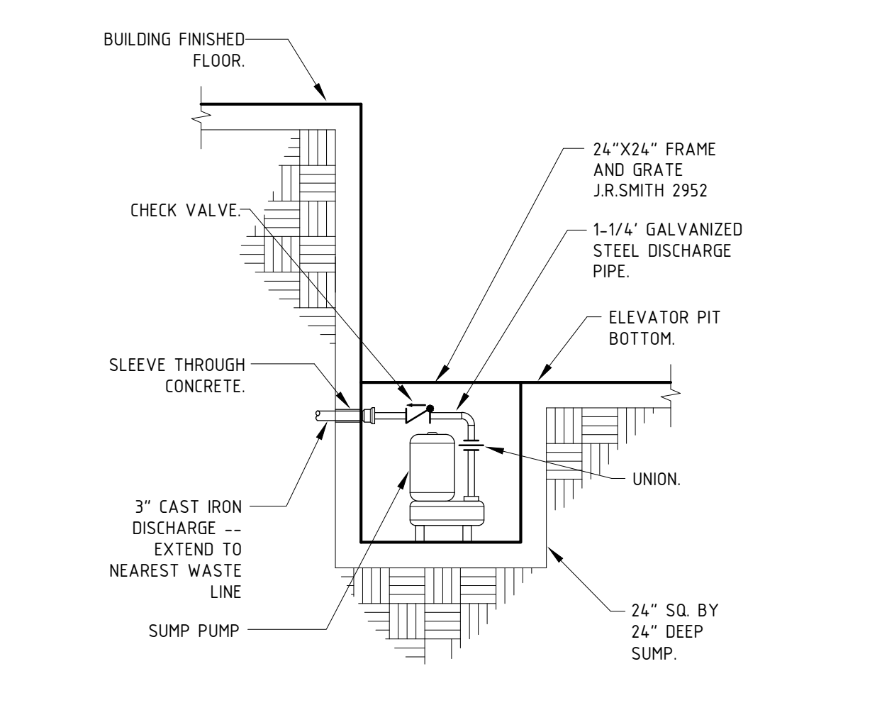
24 ELEVATOR SUMP PUMP
