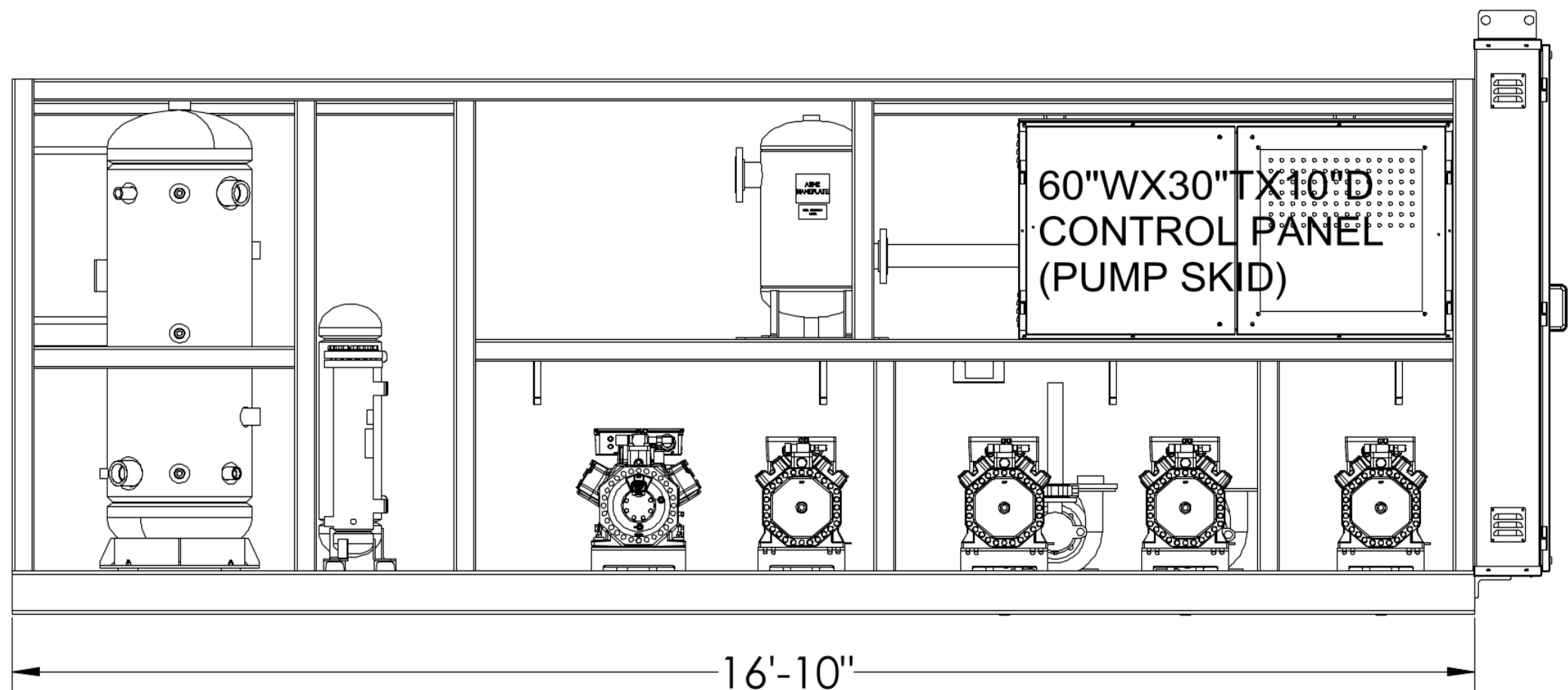
FRONT ELEVATION
