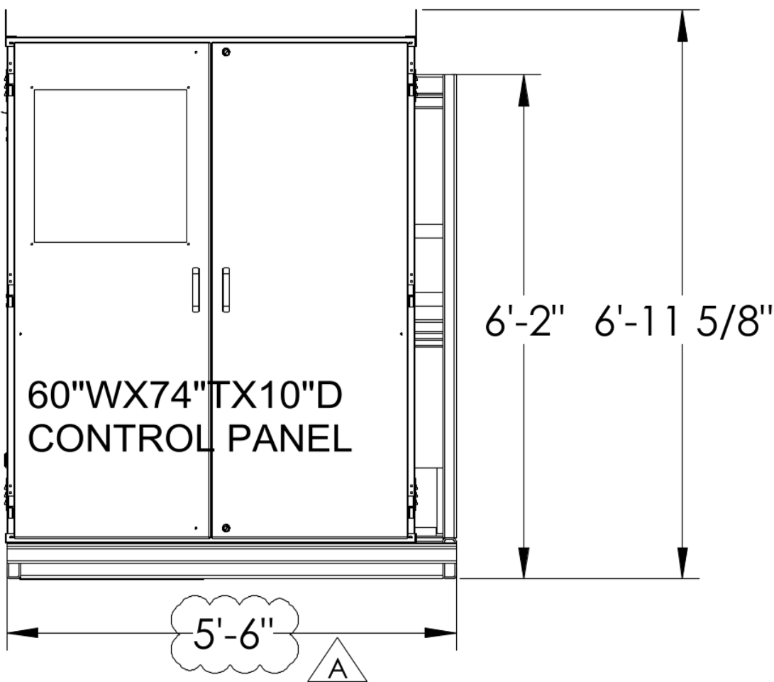
SIDE ELEVATION
