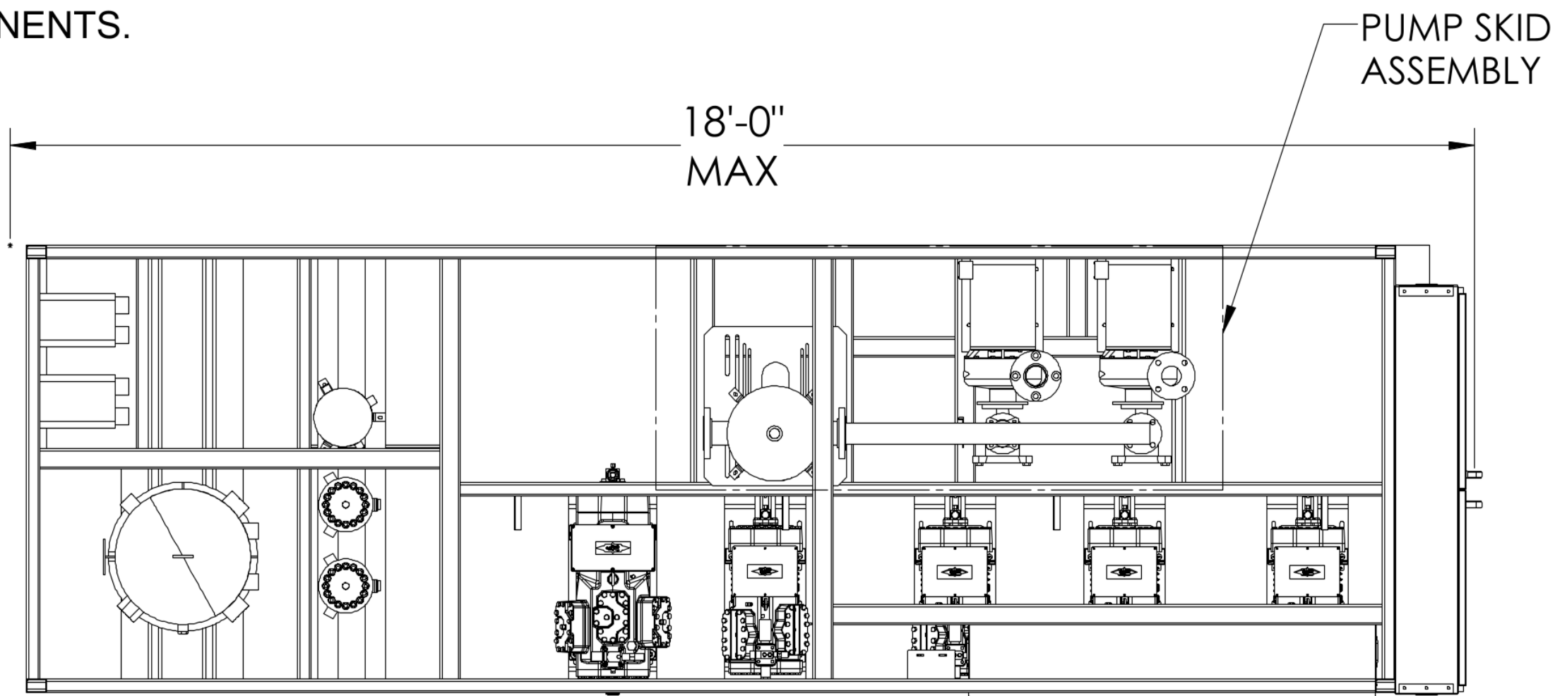
TOP VIEW
