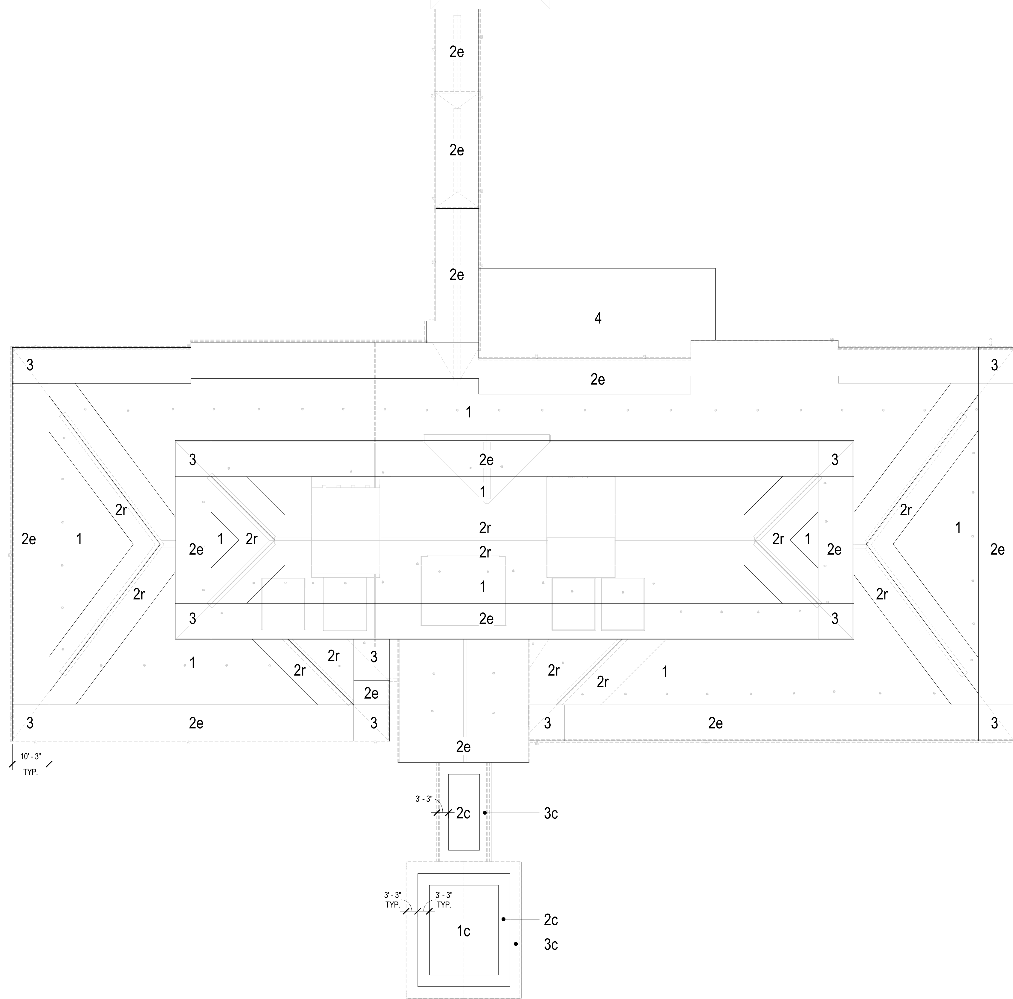
WIND UPLIFT DIAGRAM 1/16" = 1'-0"
