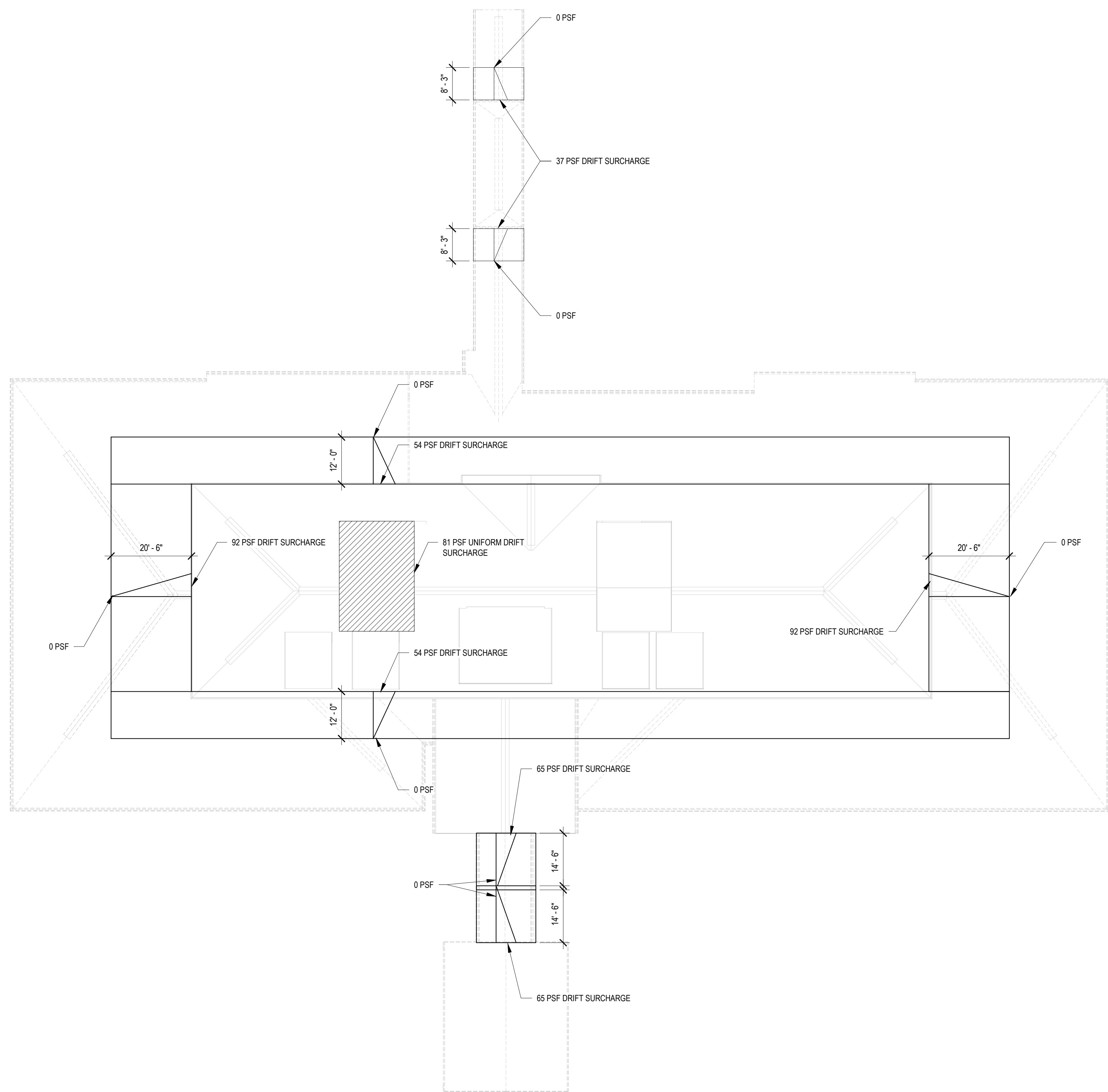
SNOW DRIFT DIAGRAM 1/16" = 1'-0"
