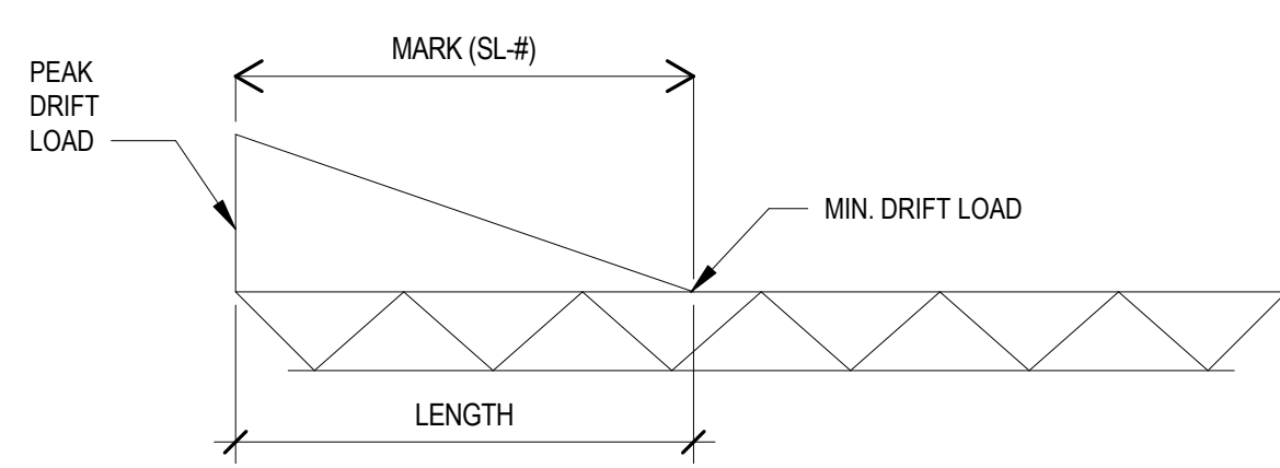
SNOW DRIFT DIAGRAM 1/16" = 1'-0"
