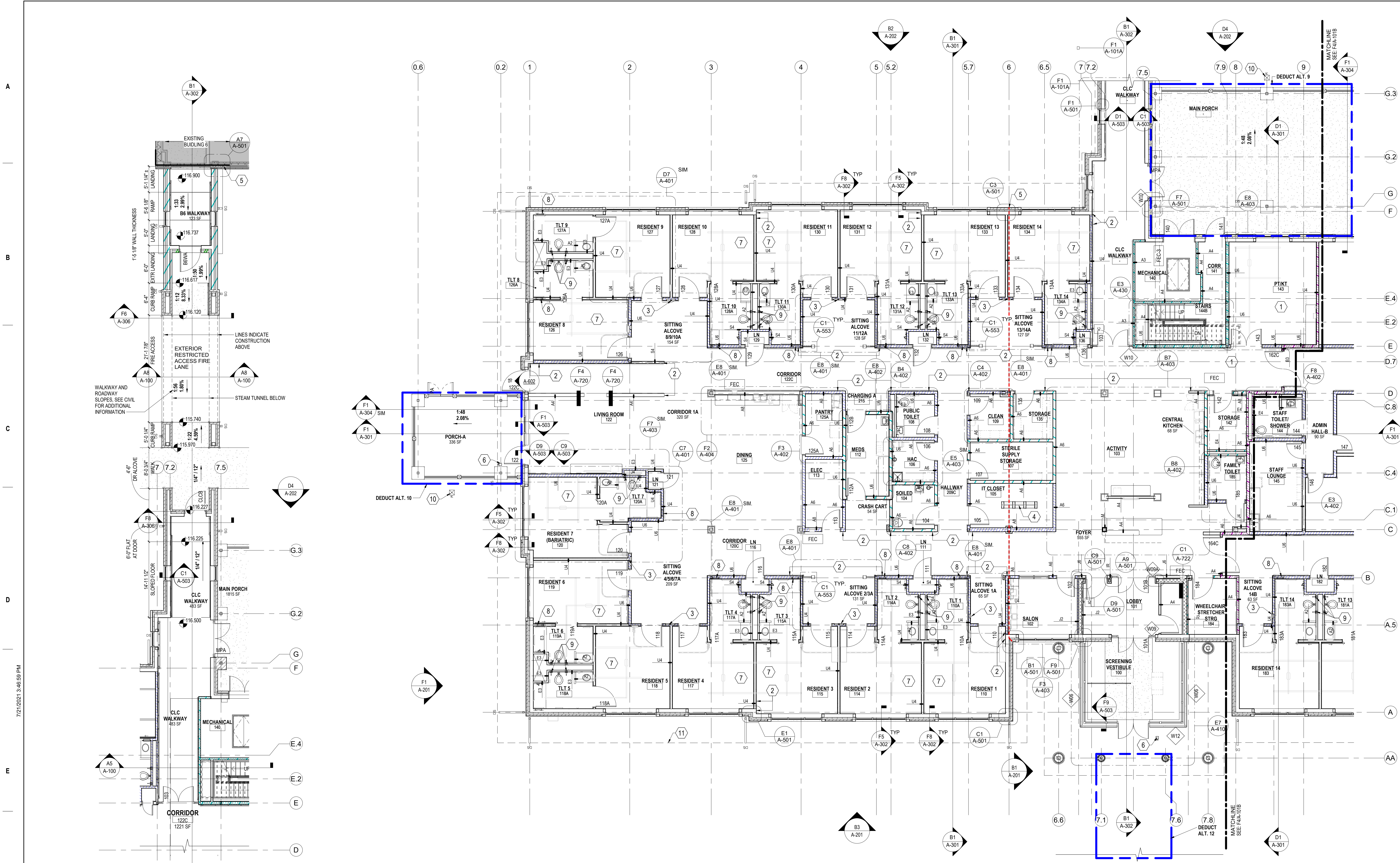
F1 ARCHITECTURAL PLAN - ENLARGED COVERED WALKWAY 1/8" = 1'-0" F3 ARCHITECTURAL FLOOR PLAN - LEVEL 1 - AREA A 1/8" = 1'-0"
