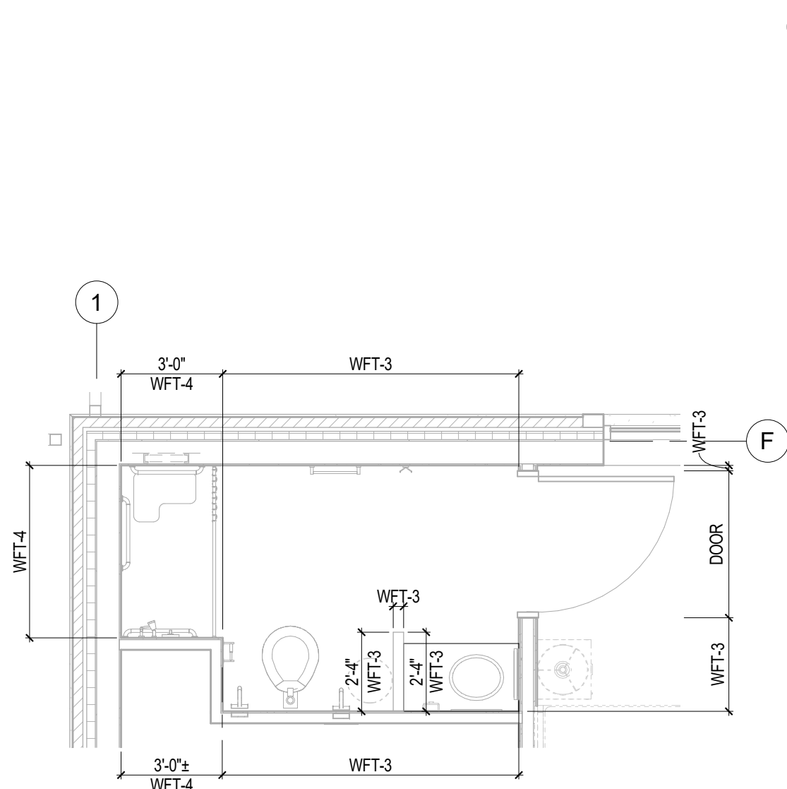
B1 TYPICAL TOILET WALL FINISHES 1/4" = 1'-0"
