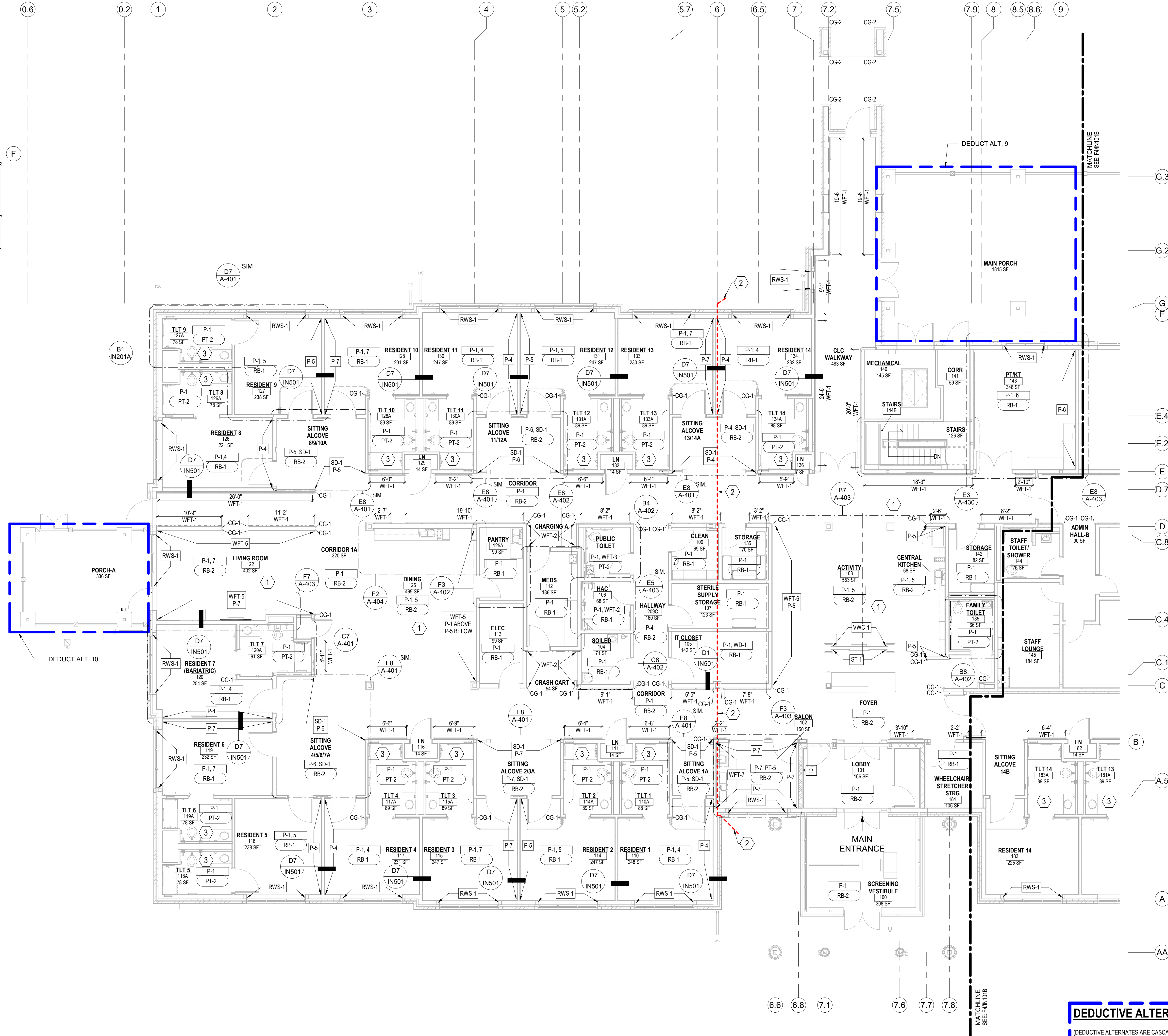
F2 INTERIOR WALL FINISH PLAN - LEVEL 1 - AREA A 1/8" = 1'-0"
