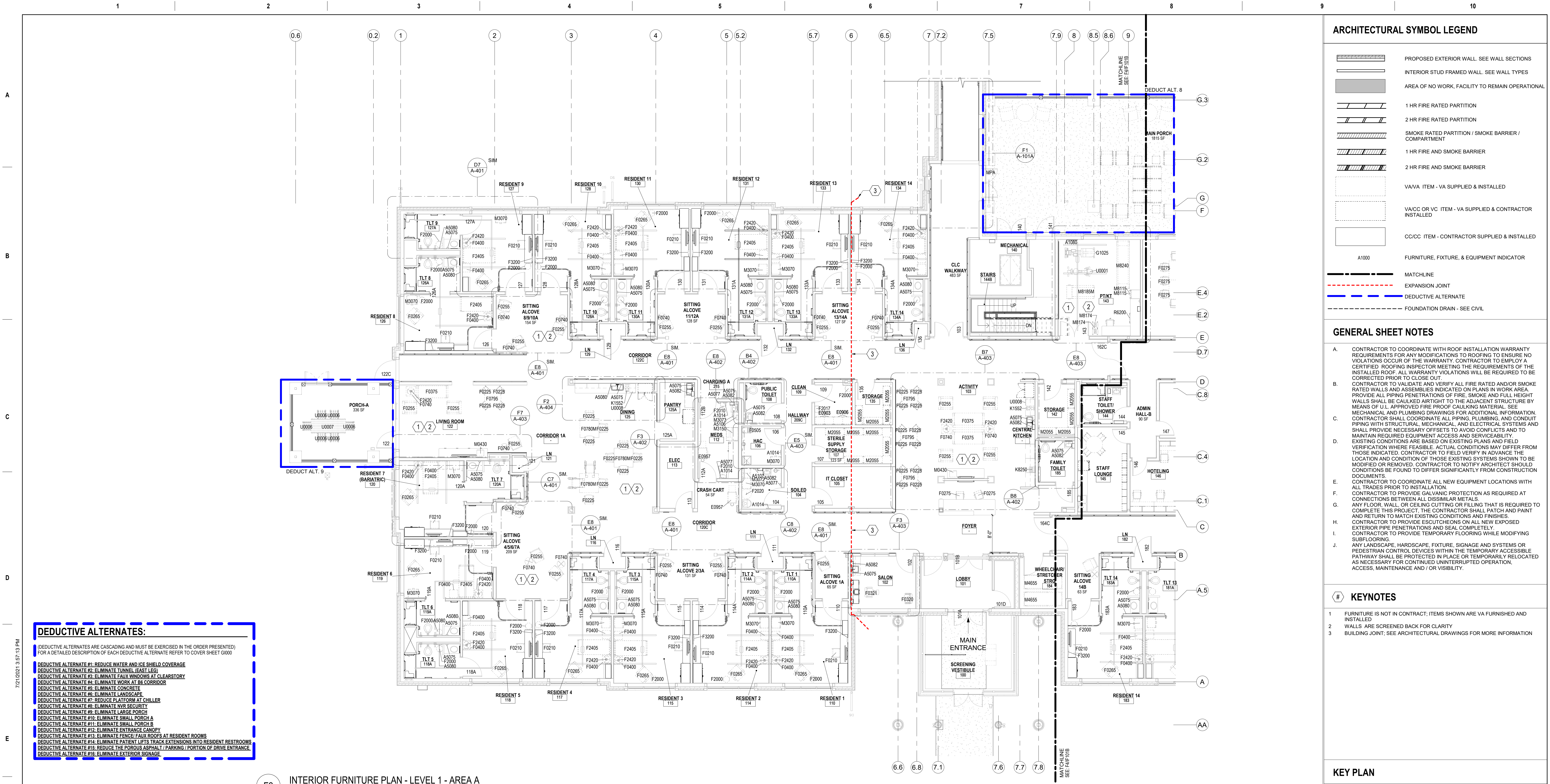
F2 INTERIOR FURNITURE PLAN - LEVEL 1 - AREA A 1/8" = 1'-0"
