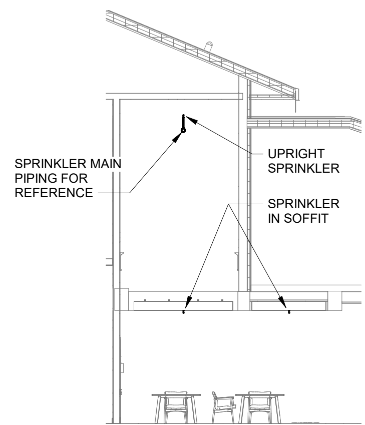
2 DINING 168 SECTION 1/8" = 1'-0"
