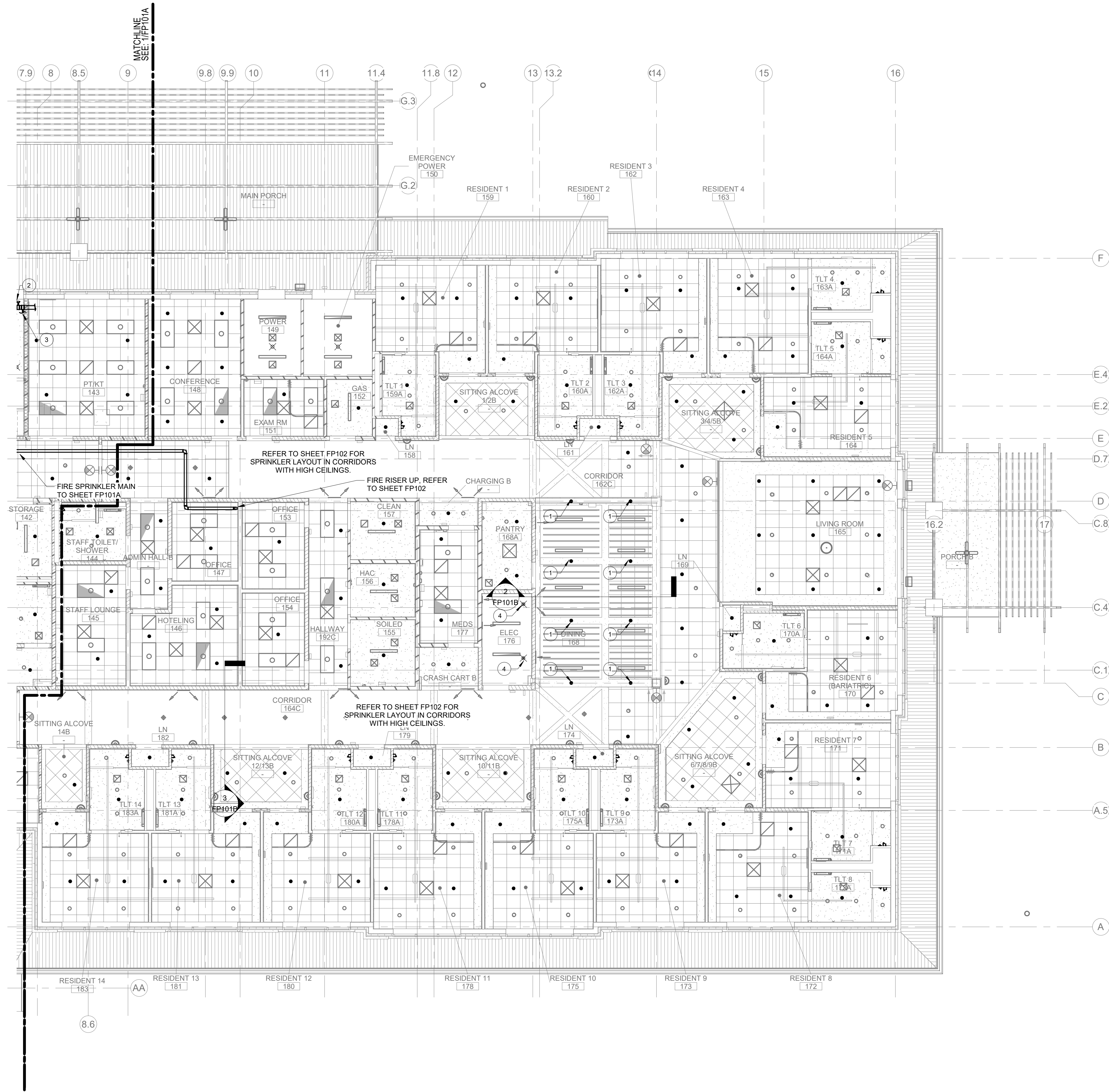
1 FIRE SPRINKLER FLOOR PLAN - LEVEL 1 - AREA B 1/8" = 1'-0"
