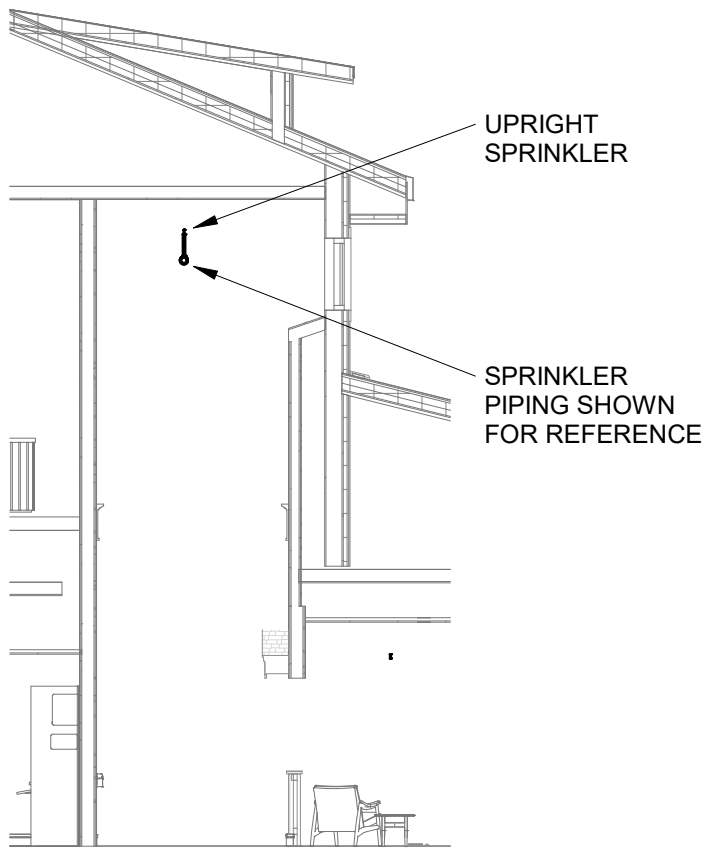
3 CORRIDOR 164C SECTION 1/8" = 1'-0"
