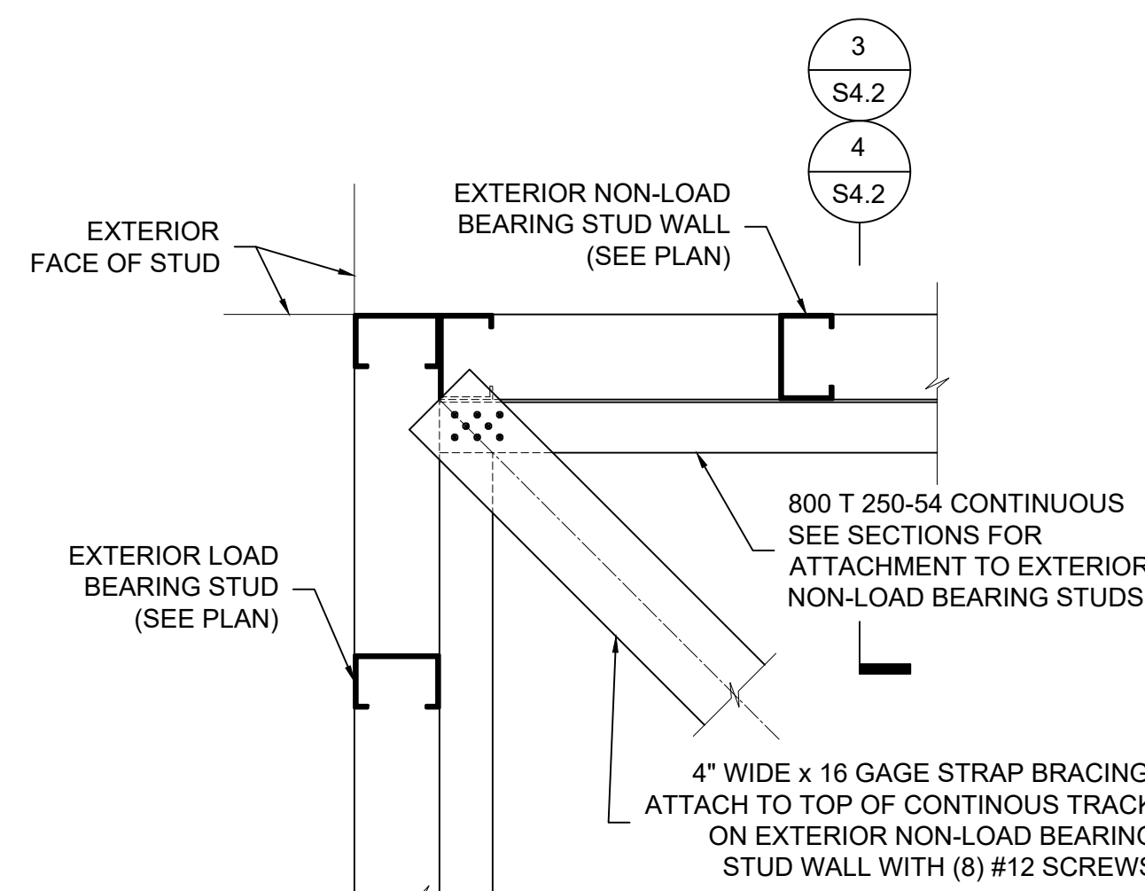
PLAN DETAIL 9 OF STRAP BRACING CORNER CONNECTION TO EXTERIOR CORNER WALL
