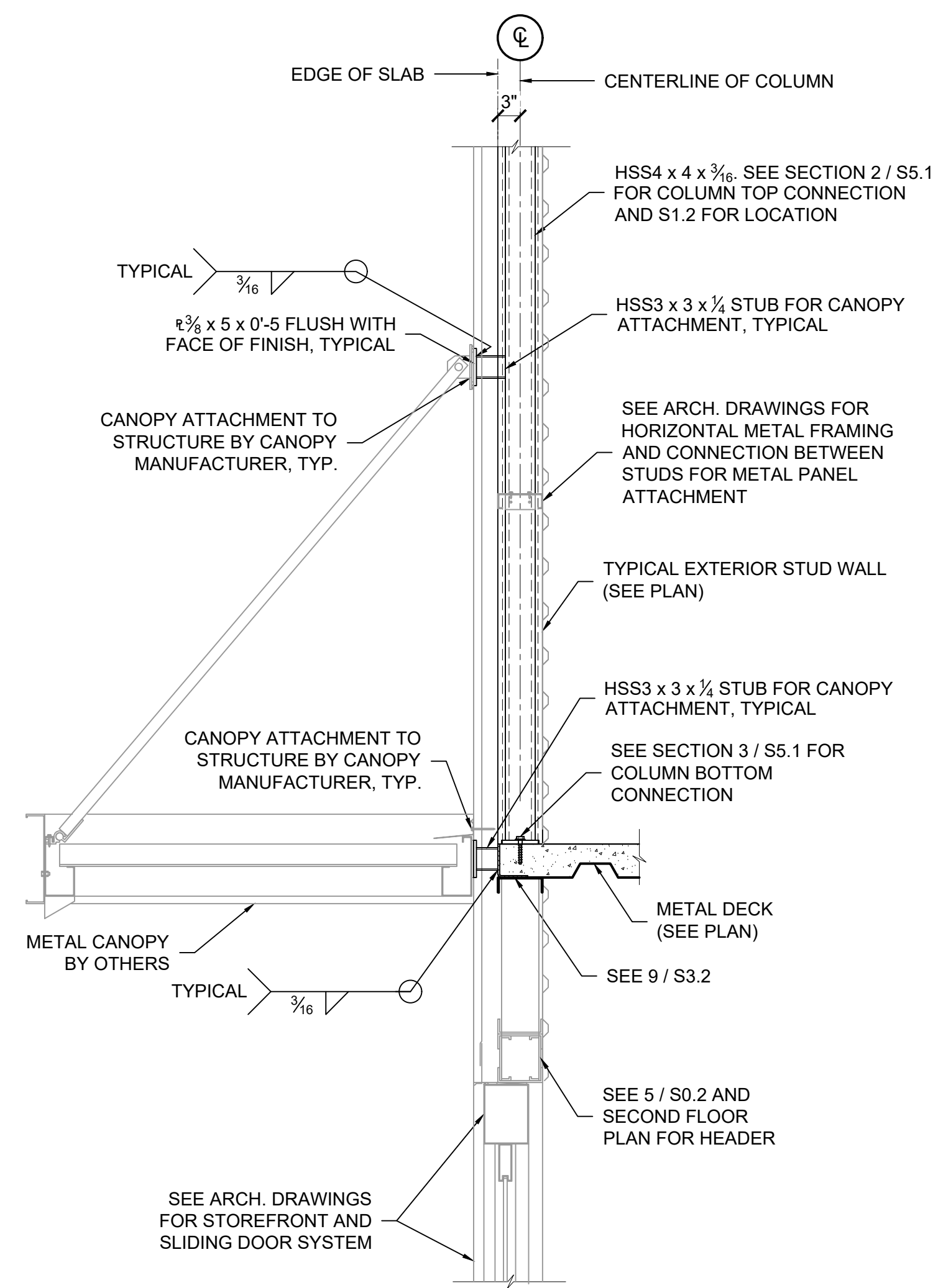
SECTION THRU CANOPY CONNECTION TO STEEL COLUMN AT STOREFRONT SCALE: \frac{3}{4}" = 1'-0" 1 S5.1
