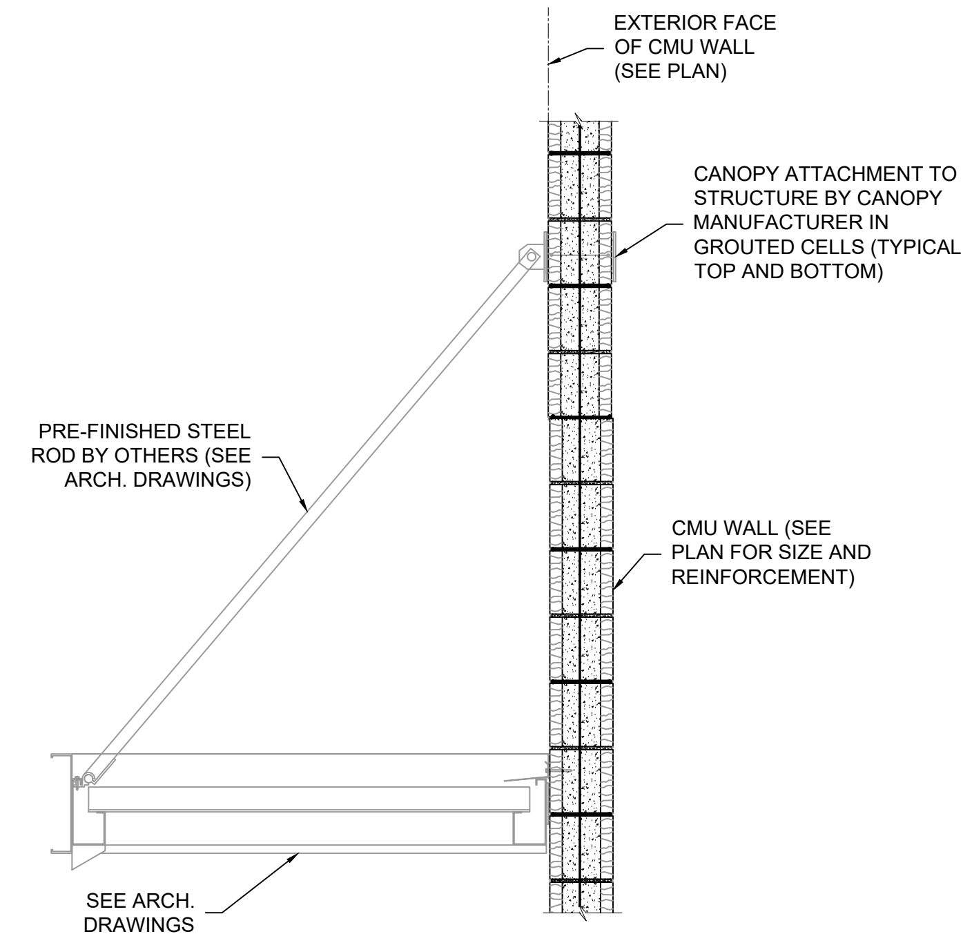
SECTION THRU CANOPY CONNECTION TO CMU WALL AT STOREFRONT SCALE: \frac{3}{4}" = 1'-0" 4 S5.1
