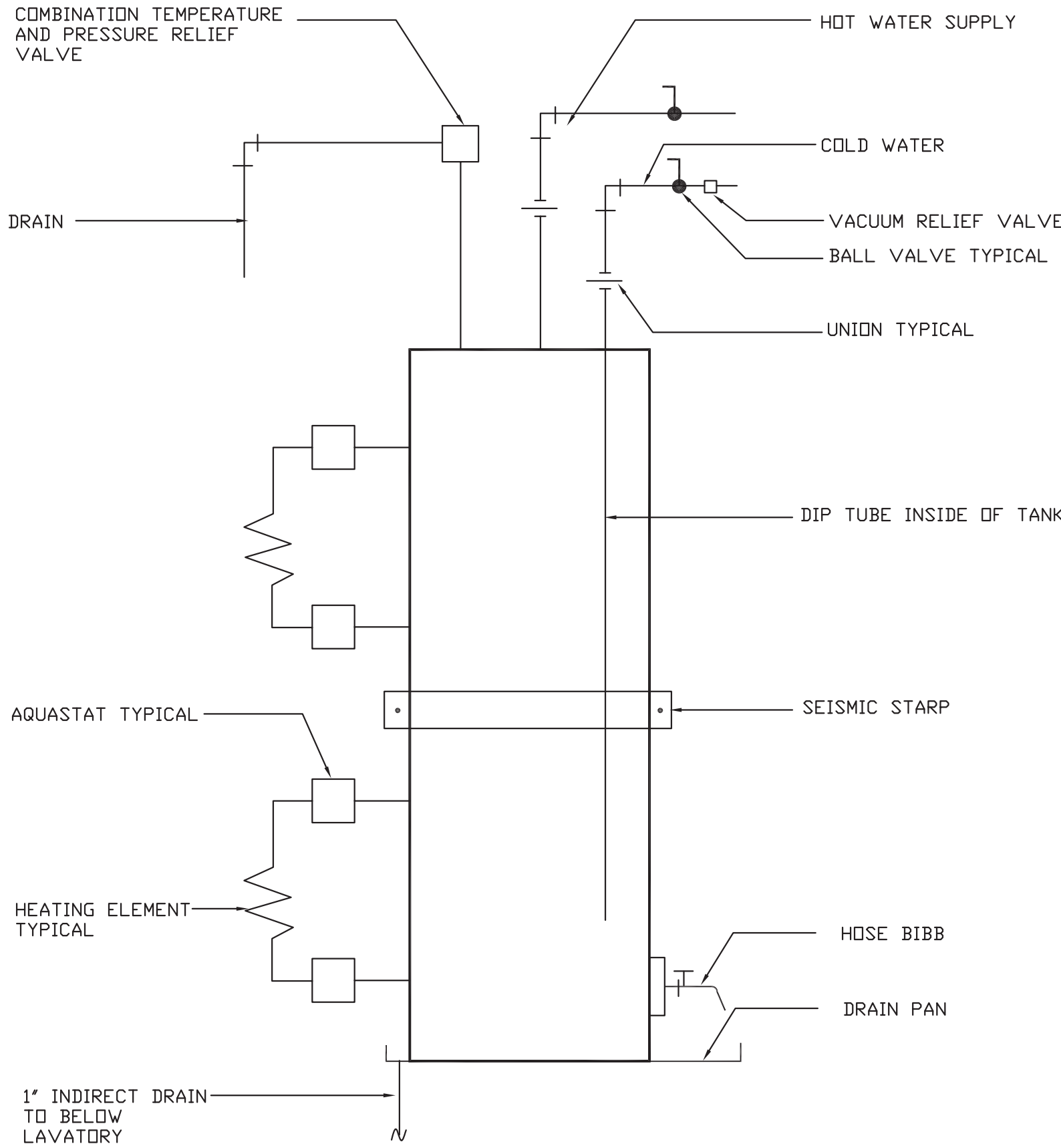
3 ELECTRIC WATER HEATER DETAIL SCALE: NOT TO SCALE
