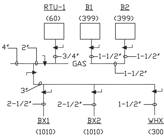
2 GAS RISER DIAGRAM SCALE: NOT TO SCALE
