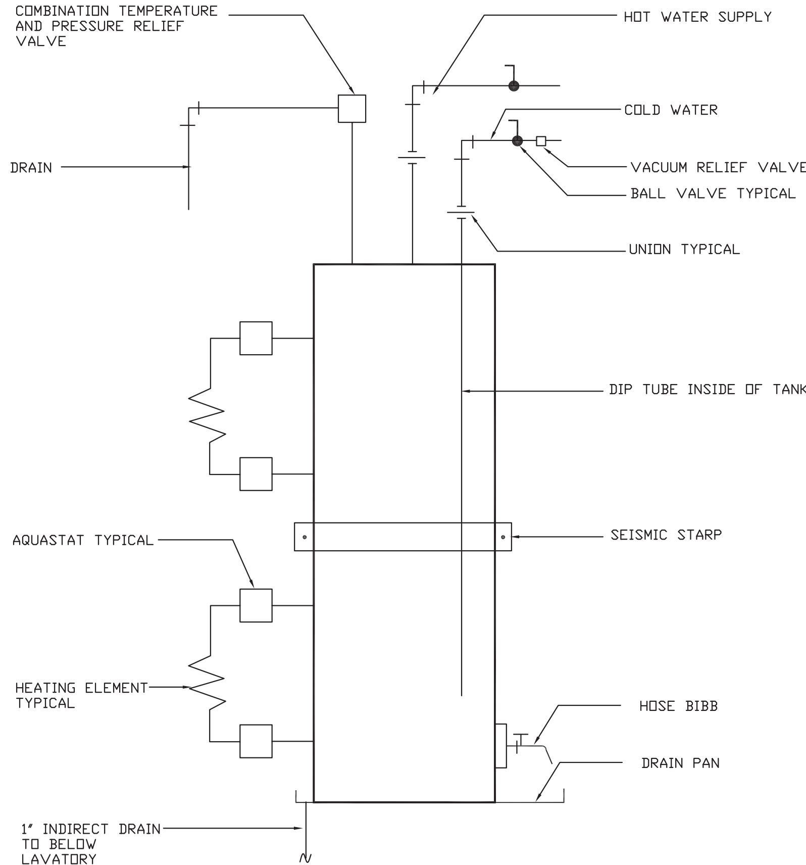
③ ELECTRIC WATER HEATER DETAIL SCALE: NOT TO SCALE
