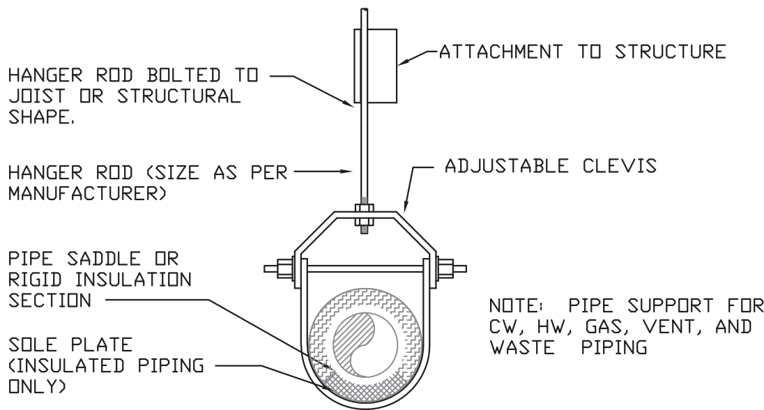
① PIPE HANGER DETAIL SCALE: NOT TO SCALE
