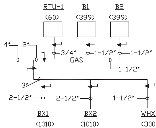
② GAS RISER DIAGRAM SCALE: NOT TO SCALE
