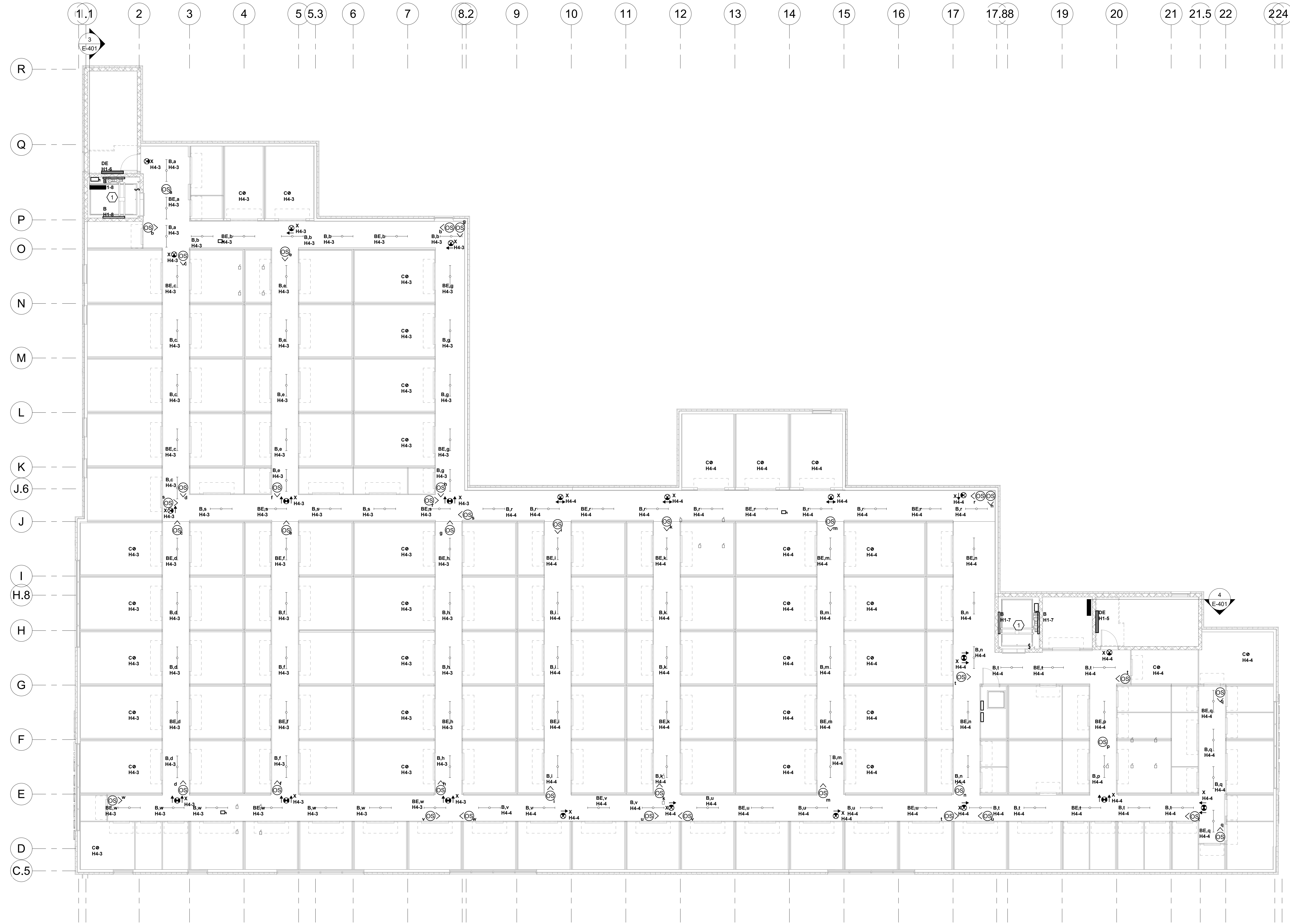
1 ELECTRICAL LIGHTING PLAN - FOURTH FLOOR 1/8" = 1'-0"
