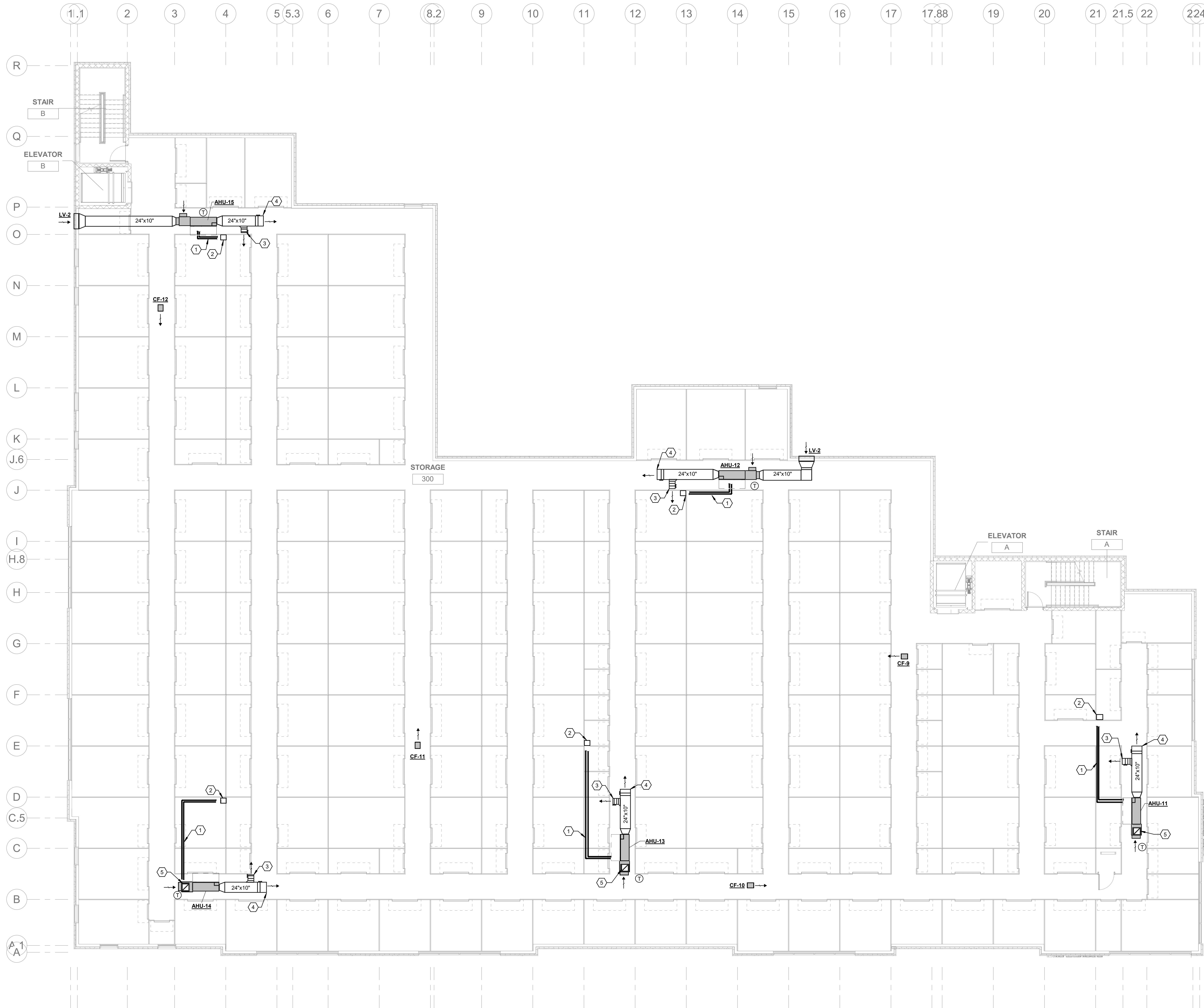
1 THIRD FLOOR MECHANICAL PLAN 1/8" = 1'-0"
