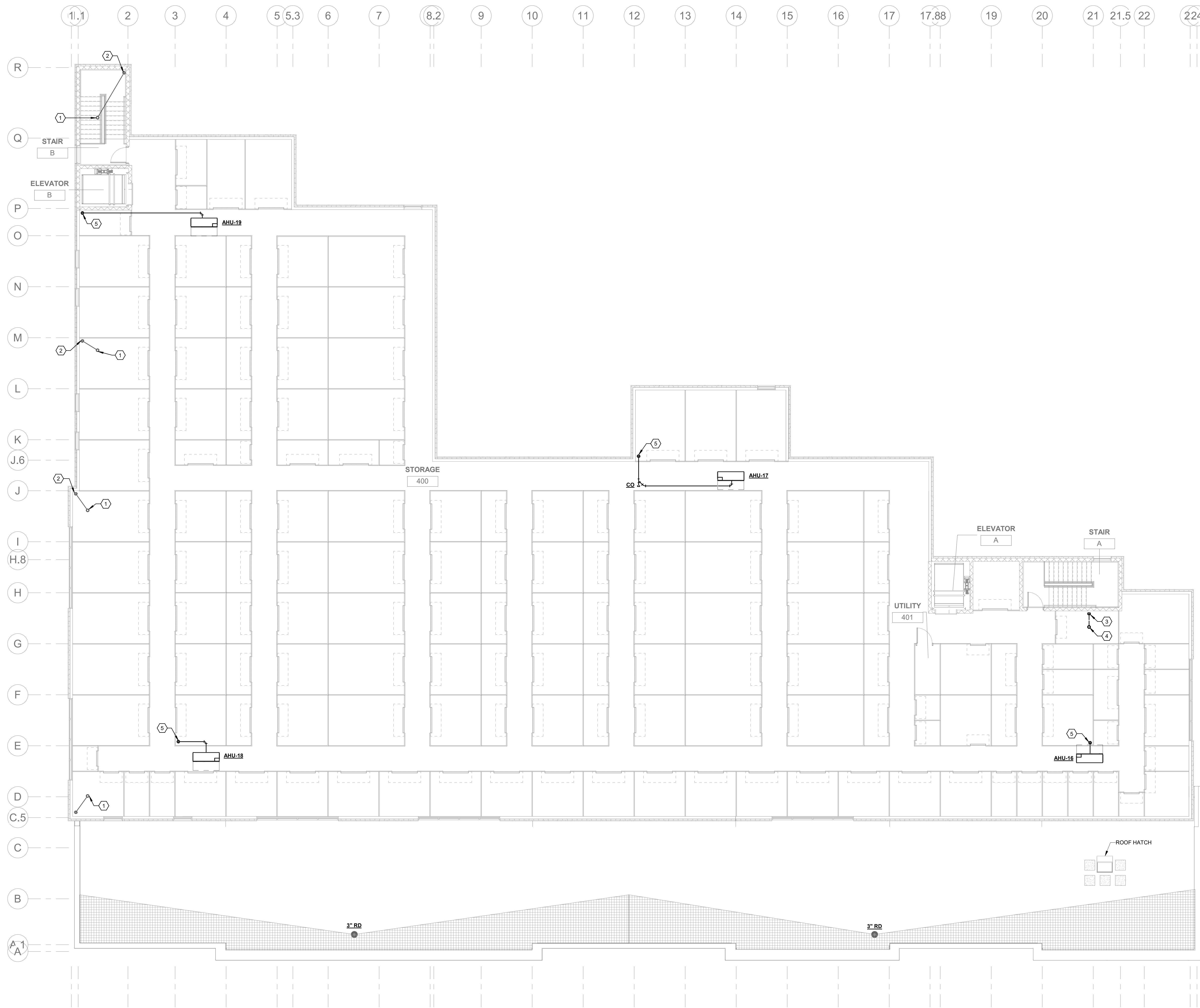
1 FOURTH FLOOR PLUMBING PLAN 1/8" = 1'-0"
