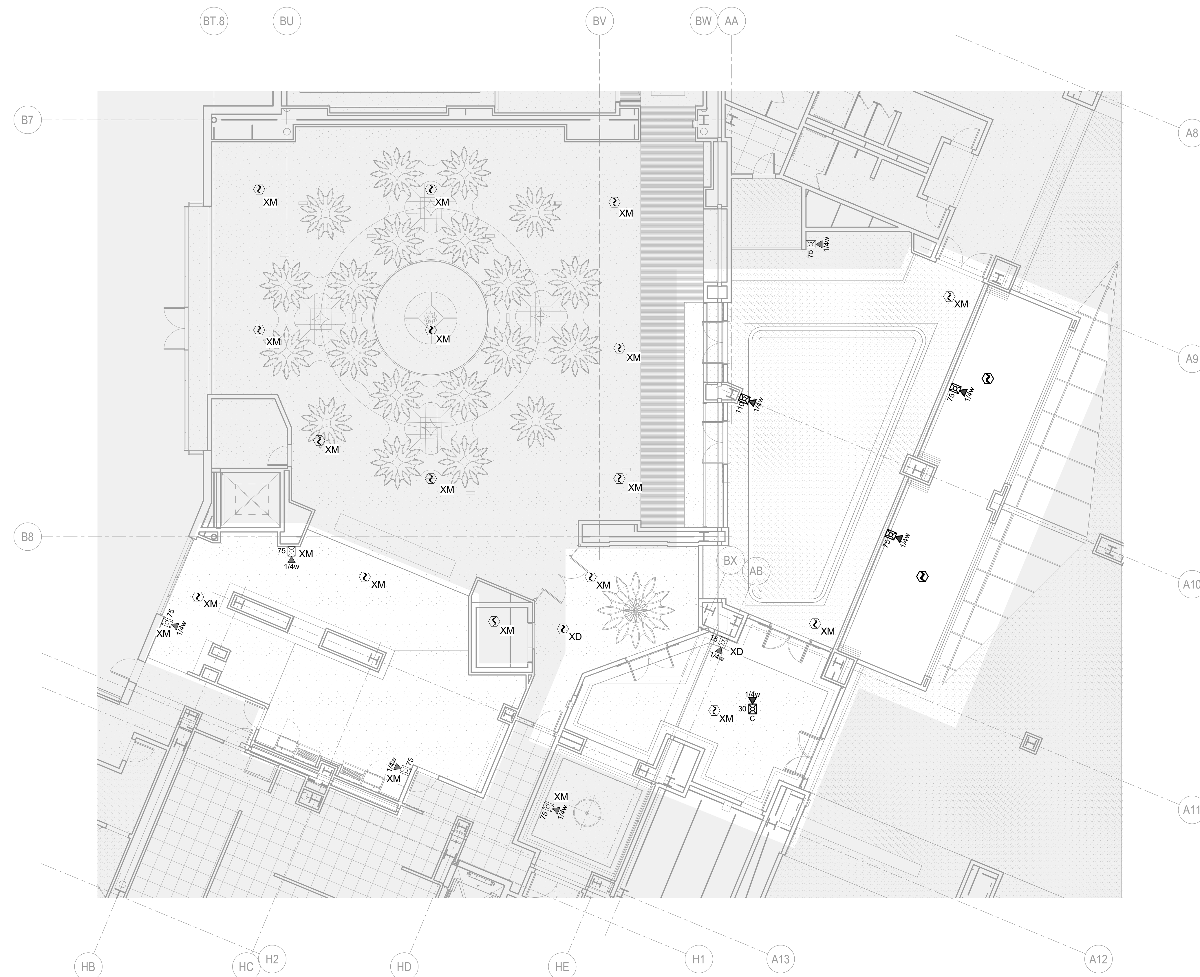
① FIRE ALARM - THIRD FLOOR 1/8" = 1'-0"
