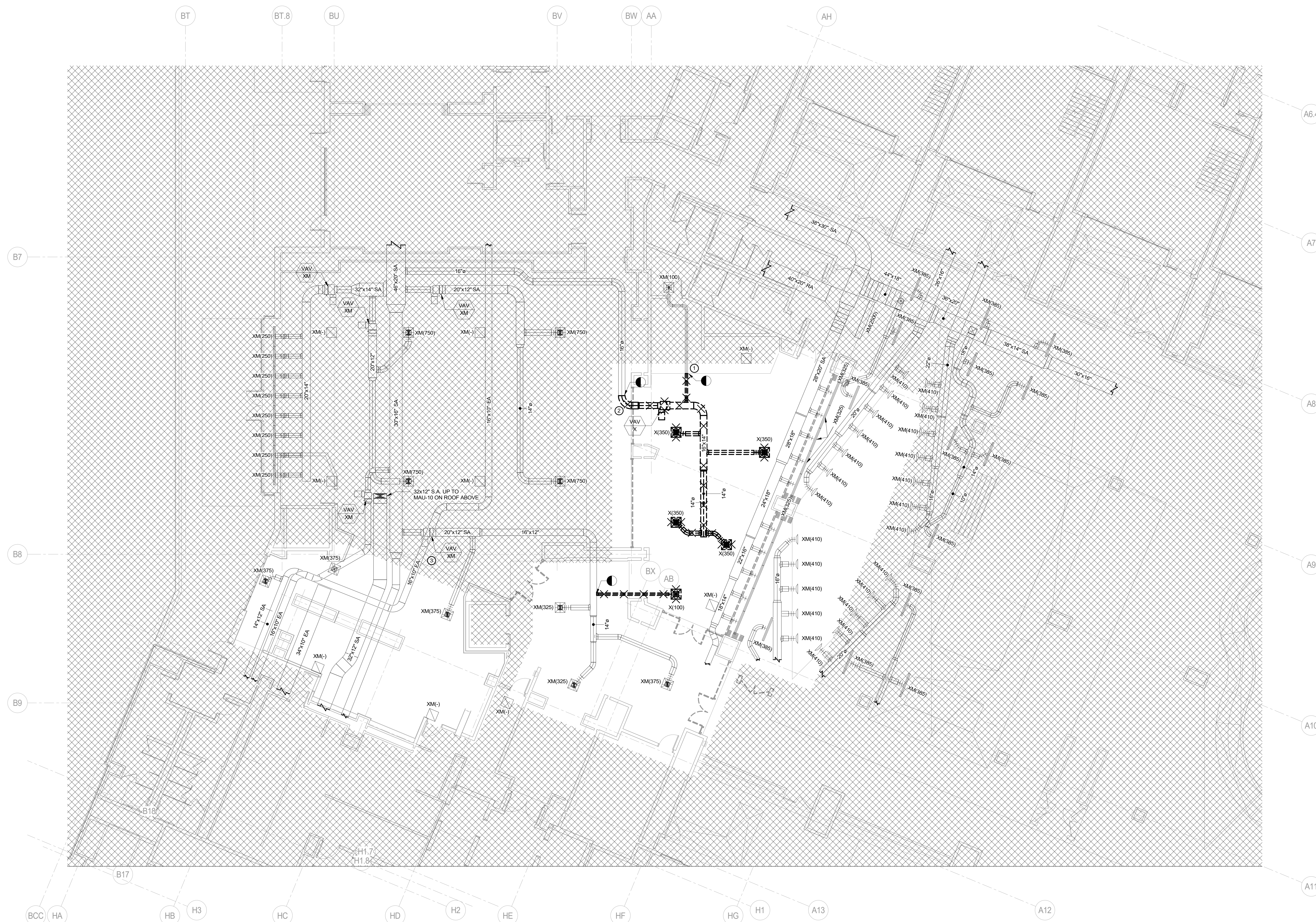
① HVAC - DEMO THIRD FLOOR 1/8" = 1'-0"
