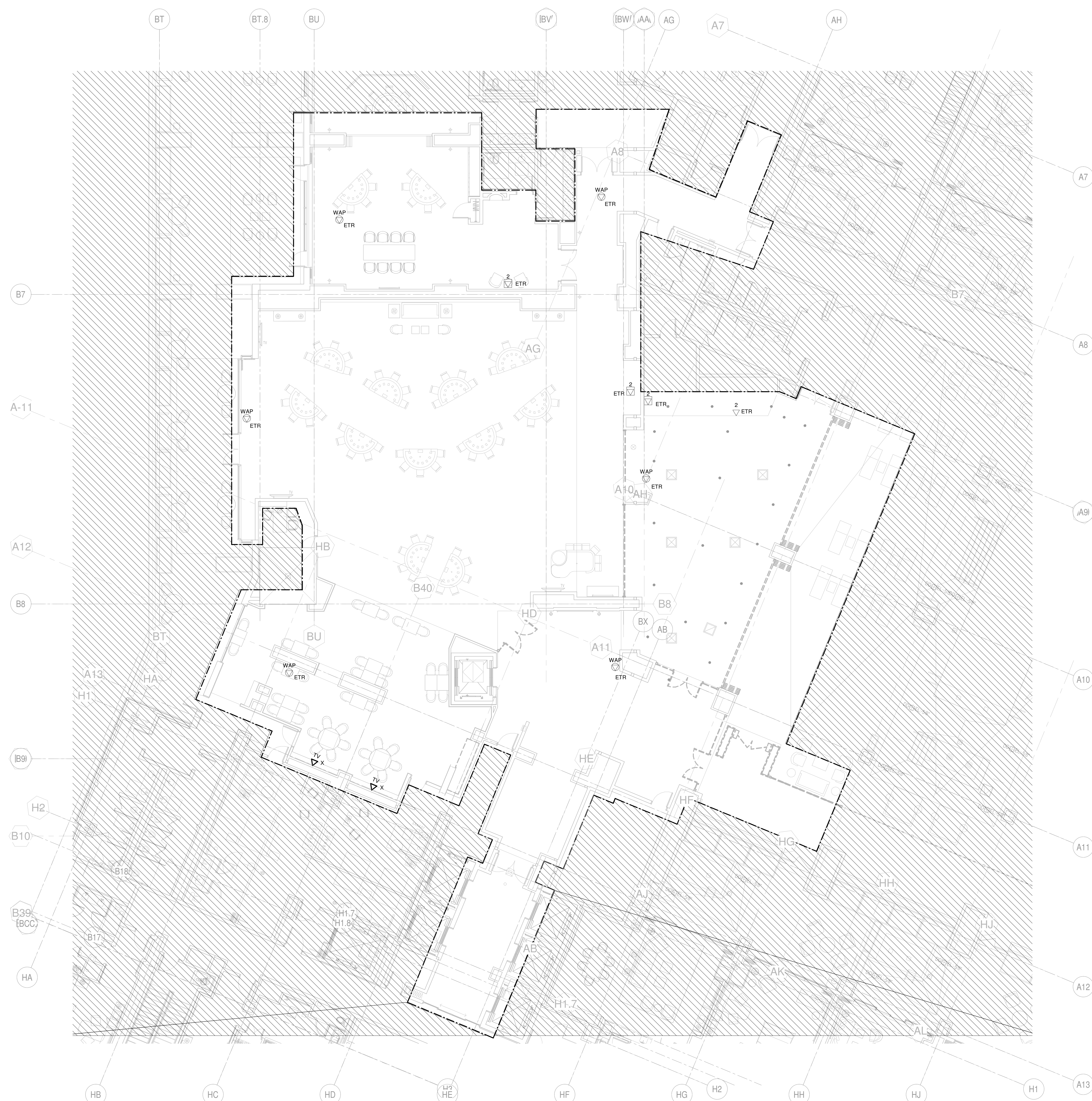
1 TELECOM - DEMO THIRD FLOOR 1/8" = 1'-0"
